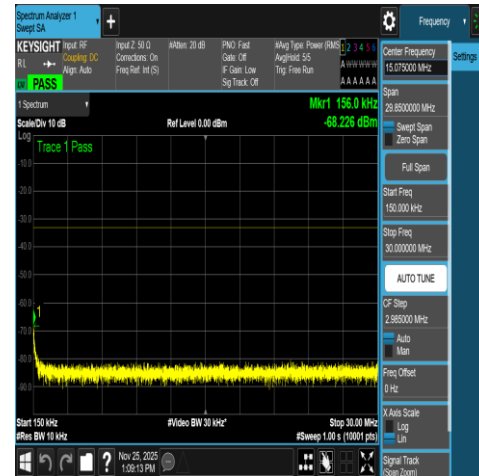
NTNV-N66-PC3-15-40-L-DFT-QPSK-Outter_Full-0. 15-30-Ant1-PASS
