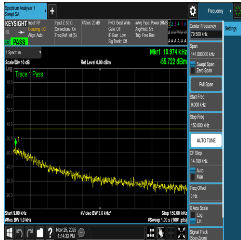
NTNV-N66-PC3-15-40-M-DFT-QPSK-Edge_1RB_ Left-0.009-0.15-Ant1-PASS
