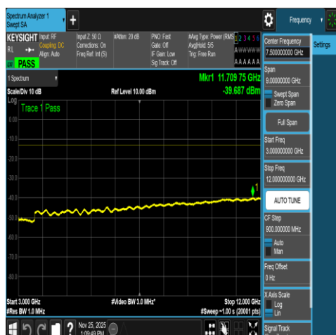
NTNV-N66-PC3-15-40-L-DFT-QPSK-Outter_Full-3 000-12000-Ant1-PASS
