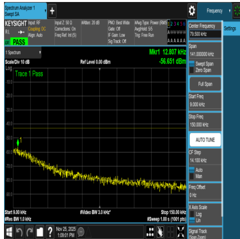
NTNV-N66-PC3-15-40-L-DFT-QPSK-Outter_Full-0. 009-0.15-Ant1-PASS
