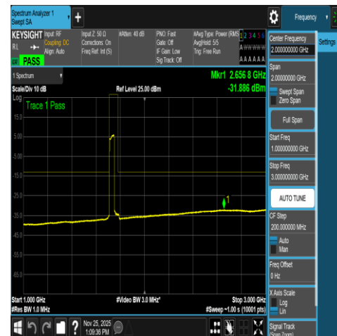
NTNV-N66-PC3-15-40-L-DFT-QPSK-Outter_Full-1 000-3000-Ant1-PASS
