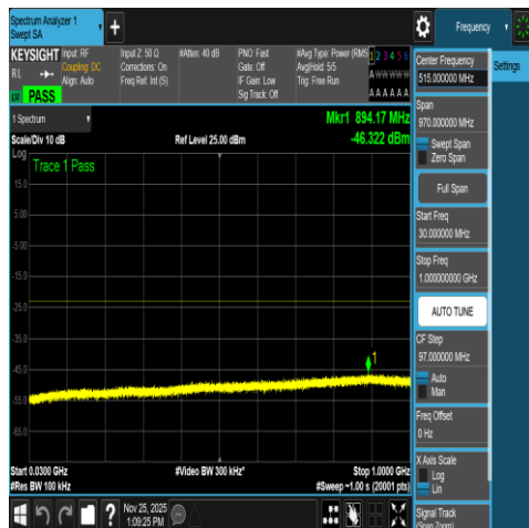
NTNV-N66-PC3-15-40-L-DFT-QPSK-Outter_Full-3 0-1000-Ant1-PASS
