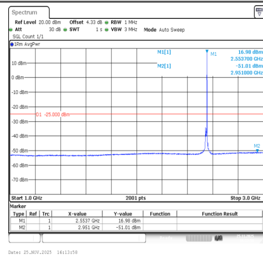
7-7-15MHz-15MHz-16QAM-16QAM-21225-21375- 1RB#74-0RB#0-1000~3000MHz-PASS
