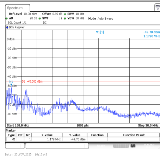
7-7-15MHz-15MHz-16QAM-16QAM-21225-21375- 1RB#74-0RB#0-0.15~30MHz-PASS
