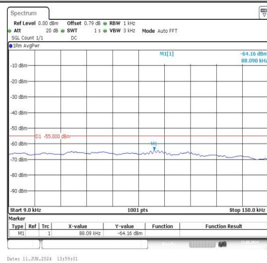
7-7-15MHz-15MHz-16QAM-16QAM-21225-21375 -1RB#74-0RB#0-0.009~0.15MHz-PASS
