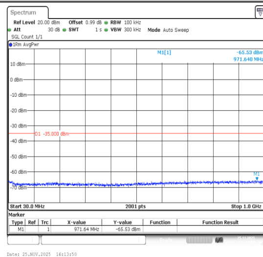
7-7-15MHz-15MHz-16QAM-16QAM-21225-21375 -1RB#74-0RB#0-30~1000MHz-PASS
