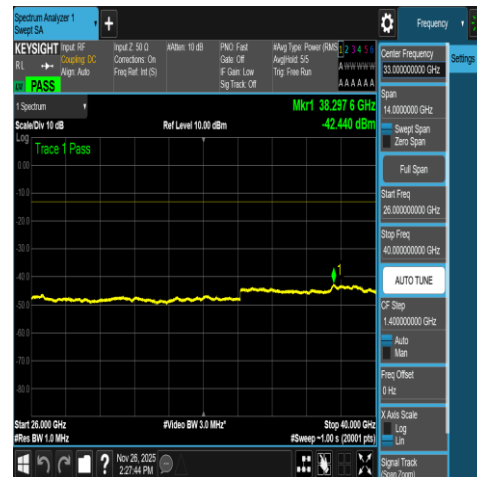
NTNV-DC_66A_n78A-3450-3550-PC2-30-5+15-M +L-N/A-N/A-DFT-QPSK-Outer_Full-26000-40000-PASS
