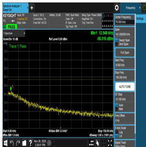
NTNV-DC_66A_n78A-3450-3550-PC2-30-5+15-M
