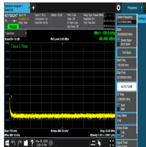
NTNV-DC_66A_n78A-3450-3550-PC2-30-5+15-M
