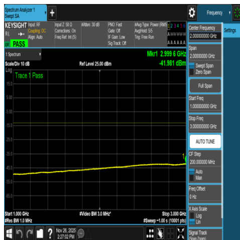
NTNV-DC_66A_n78A-3450-3550-PC2-30-5+15-M +L-N/A-N/A-DFT-QPSK-Outer_Full-1000-3000-PA
