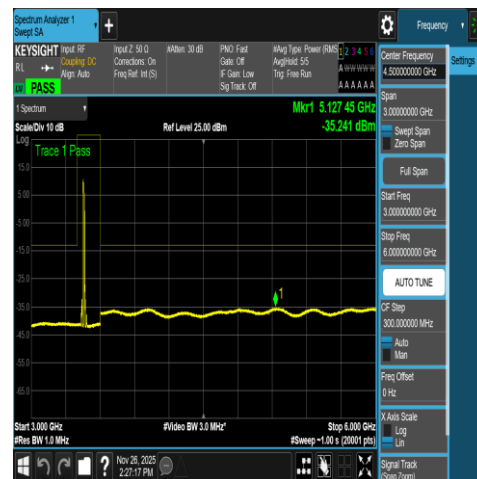
NTNV-DC_66A_n78A-3450-3550-PC2-30-5+15-M +L-N/A-N/A-DFT-QPSK-Outer_Full-3000-6000-PA
