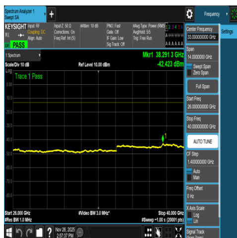
NTNV-DC_66A_n78A-3450-3550-PC2-30-5+40-M +L-N/A-N/A-DFT-QPSK-Edge_1RB_Left-26000-40
