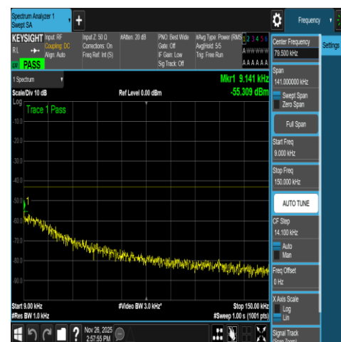
NTNV-DC_66A_n78A-3450-3550-PC2-30-5+40-M +L-N/A-N/A-DFT-QPSK-Edge_1RB_Right-0.009-0
