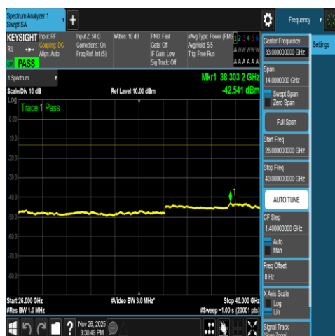
NTNV-DC_66A_n78A-3450-3550-PC2-30-5+70-M +L-N/A-N/A-DFT-QPSK-Outer_Full-26000-40000-
