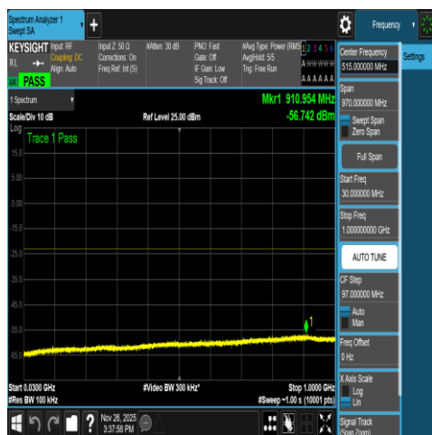
NTNV-DC_66A_n78A-3450-3550-PC2-30-5+70-M +L-N/A-N/A-DFT-QPSK-Outer_Full-30-1000-PASS
