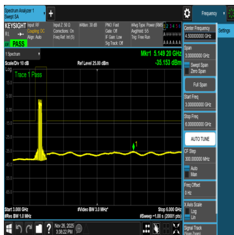
NTNV-DC_66A_n78A-3450-3550-PC2-30-5+70-M +L-N/A-N/A-DFT-QPSK-Outer_Full-3000-6000-PA SS
