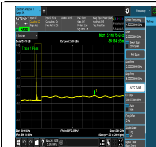
NTNV-DC_66A_n78A-3450-3550-PC2-30-5+80-M +L-N/A-N/A-DFT-QPSK-Edge_1RB_Left-3000-600 0-PASS
