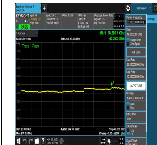
NTNV-DC_66A_n78A-3450-3550-PC2-30-5+80-M +L-N/A-N/A-DFT-QPSK-Edge_1RB_Left-26000-40 000-PASS
