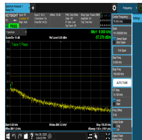
NTNV-DC_66A_n78A-3450-3550-PC2-30-5+80-M +L-N/A-N/A-DFT-QPSK-Edge_1RB_Right-0.009-0 .15-PASS
