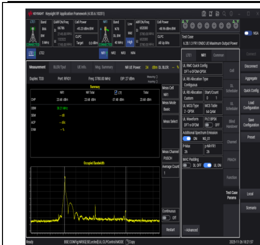
NTNV-DC_66A_n78A-3700-3800-PC2-30-5+40-M +H-N/A-N/A-DFT-QPSK-Edge_1RB_Left-PASS
