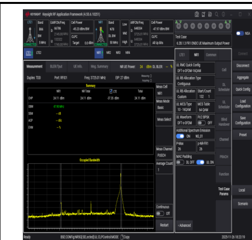
NTNV-DC_66A_n78A-3700-3800-PC2-30-5+50-M +L-N/A-N/A-DFT-16QAM-Edge_1RB_Right-PASS
