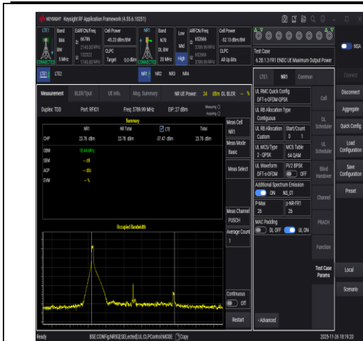
NTNV-DC_66A_n78A-3700-3800-PC2-30-5+20-M +H-N/A-N/A-DFT-QPSK-Edge_1RB_Left-PASS
