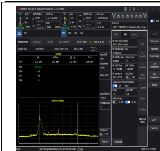
NTNV-DC_66A_n78A-3700-3800-PC2-30-5+50-M +L-N/A-N/A-DFT-16QAM-Edge_1RB_Left-PASS
