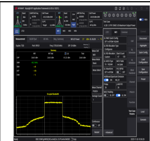
NTNV-DC_66A_n78A-3700-3800-PC2-30-5+100-M+M-N/A-N/A-DFT-16QAM-Inner_Full-PASS
