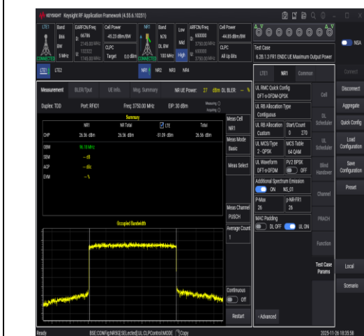
NTNV-DC_66A_n78A-3700-3800-PC2-30-5+100-M+M-N/A-N/A-DFT-QPSK-Outer_Full-PASS
