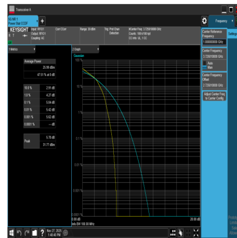
NTNV-DC_66A_n78A-3700-3800-PC2-30-5+50-M +L-N/A-N/A-DFT-16QAM-Outer_Full-PASS
