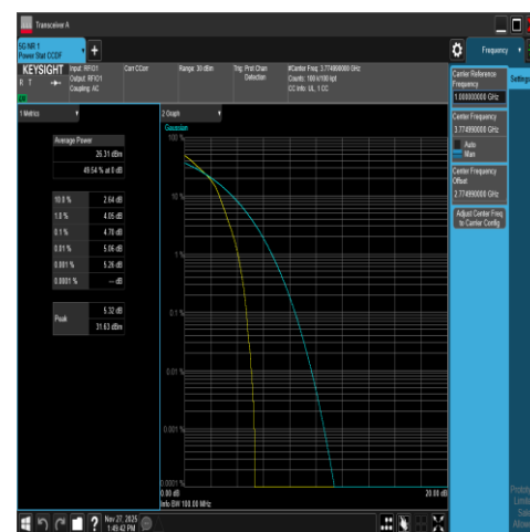
NTNV-DC_66A_n78A-3700-3800-PC2-30-5+50-M +H-N/A-N/A-DFT-16QAM-Outer_Full-PASS
