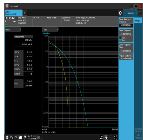
NTNV-DC_66A_n78A-3700-3800-PC2-30-5+15-M +L-N/A-N/A-DFT-16QAM-Outer_Full-PASS
