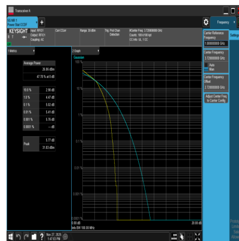
NTNV-DC_66A_n78A-3700-3800-PC2-30-5+40-M +L-N/A-N/A-DFT-16QAM-Outer_Full-PASS
