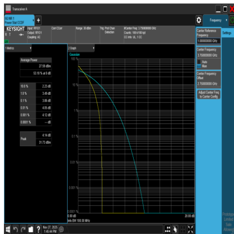
NTNV-DC_66A_n78A-3700-3800-PC2-30-5+20-M +M-N/A-N/A-DFT-QPSK-Outer_Full-PASS
