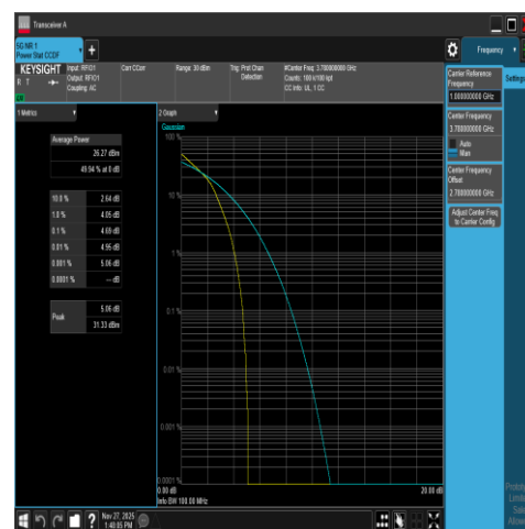
NTNV-DC_66A_n78A-3700-3800-PC2-30-5+40-M +H-N/A-N/A-DFT-16QAM-Outer_Full-PASS
