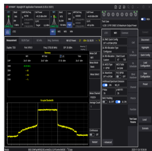
NTNV-DC_66A_n78A-3700-3800-PC2-30-5+100-M+M-N/A-N/A-DFT-QPSK-Inner_Full-PASS
