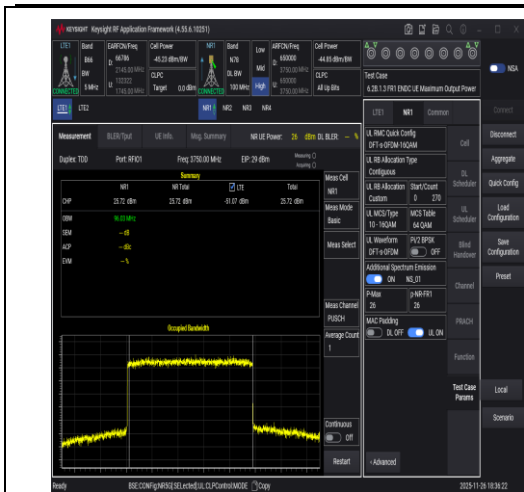
NTNV-DC_66A_n78A-3700-3800-PC2-30-5+100-M+M-N/A-N/A-DFT-16QAM-Outer_Full-PASS
