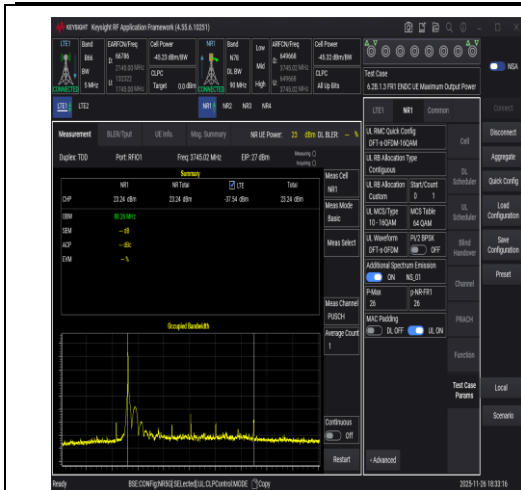
NTNV-DC_66A_n78A-3700-3800-PC2-30-5+90-M +L-N/A-N/A-DFT-16QAM-Edge_1RB_Left-PASS
