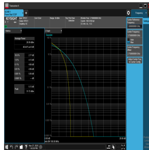
NTNV-DC_66A_n78A-3700-3800-PC2-30-5+20-M +M-N/A-N/A-DFT-16QAM-Outer_Full-PASS
