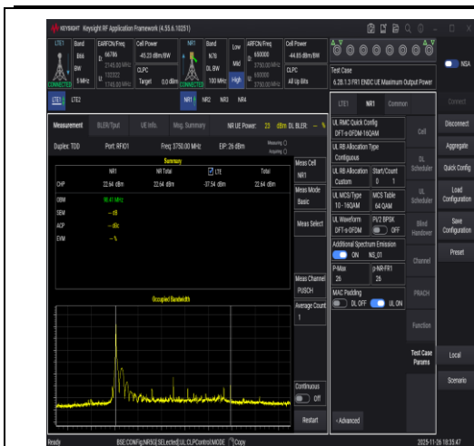
NTNV-DC_66A_n78A-3700-3800-PC2-30-5+100-M+L-N/A-N/A-DFT-16QAM-Edge_1RB_Left-PASS
