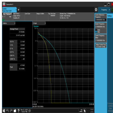
NTNV-DC_66A_n78A-3700-3800-PC2-30-5+50-M +M-N/A-N/A-DFT-QPSK-Outer_Full-PASS
