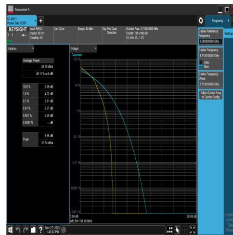
NTNV-DC_66A_n78A-3700-3800-PC2-30-5+20-M +L-N/A-N/A-DFT-16QAM-Outer_Full-PASS
