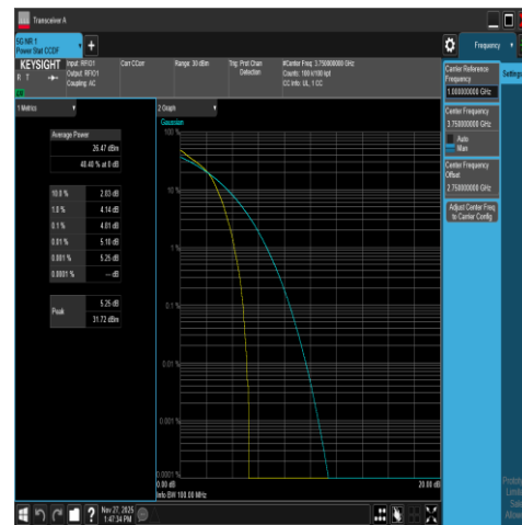
NTNV-DC_66A_n78A-3700-3800-PC2-30-5+40-M +M-N/A-N/A-DFT-16QAM-Outer_Full-PASS
