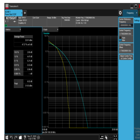
NTNV-DC_66A_n78A-3700-3800-PC2-30-5+60-M +L-N/A-N/A-DFT-16QAM-Outer_Full-PASS
