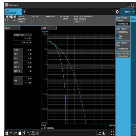
NTNV-DC_66A_n78A-3700-3800-PC2-30-5+50-M +M-N/A-N/A-DFT-16QAM-Outer_Full-PASS
