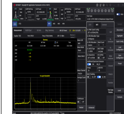
NTNV-DC_66A_n78A-3700-3800-PC2-30-5+90-M +M-N/A-N/A-DFT-QPSK-Edge_1RB_Left-PASS
