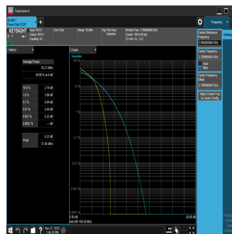
NTNV-DC_66A_n78A-3700-3800-PC2-30-5+20-M +H-N/A-N/A-DFT-16QAM-Outer_Full-PASS
