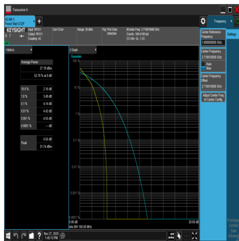
NTNV-DC_66A_n78A-3700-3800-PC2-30-5+20-M +L-N/A-N/A-DFT-QPSK-Outer_Full-PASS
