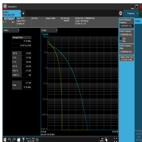
NTNV-DC_66A_n78A-3700-3800-PC2-30-5+20-M +H-N/A-N/A-DFT-QPSK-Outer_Full-PASS
