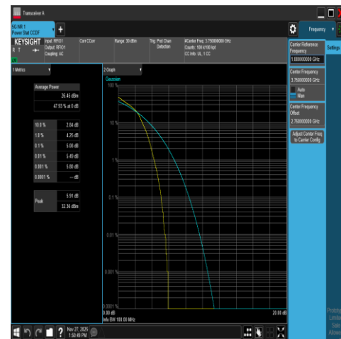
NTNV-DC_66A_n78A-3700-3800-PC2-30-5+60-M +M-N/A-N/A-DFT-16QAM-Outer_Full-PASS
