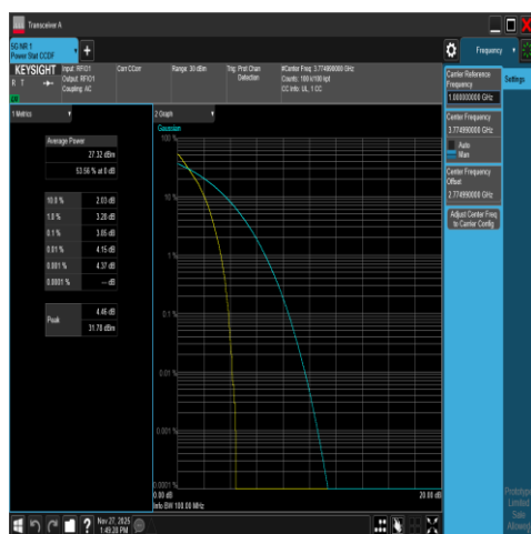
NTNV-DC_66A_n78A-3700-3800-PC2-30-5+50-M +H-N/A-N/A-DFT-QPSK-Outer_Full-PASS
