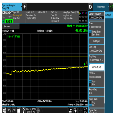
NTNV-N7-PC3-15-15-M-DFT-QPSK-Edge_1RB_R- ight-3000-12000-Ant1-PASS
