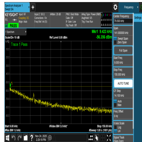
NTNV-N7-PC3-15-15-M-DFT-QPSK-Edge_1RB_R- ight-0.009-0.15-Ant1-PASS
