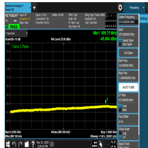
NTNV-N7-PC3-15-15-M-DFT-QPSK-Edge_1RB_R- ight-30-1000-Ant1-PASS
