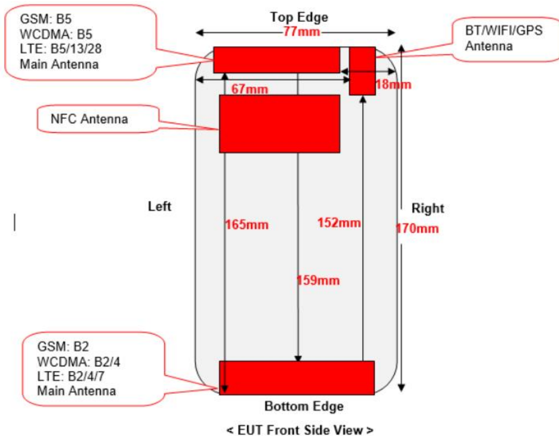
Block Diagram for EUT Antenna Position
