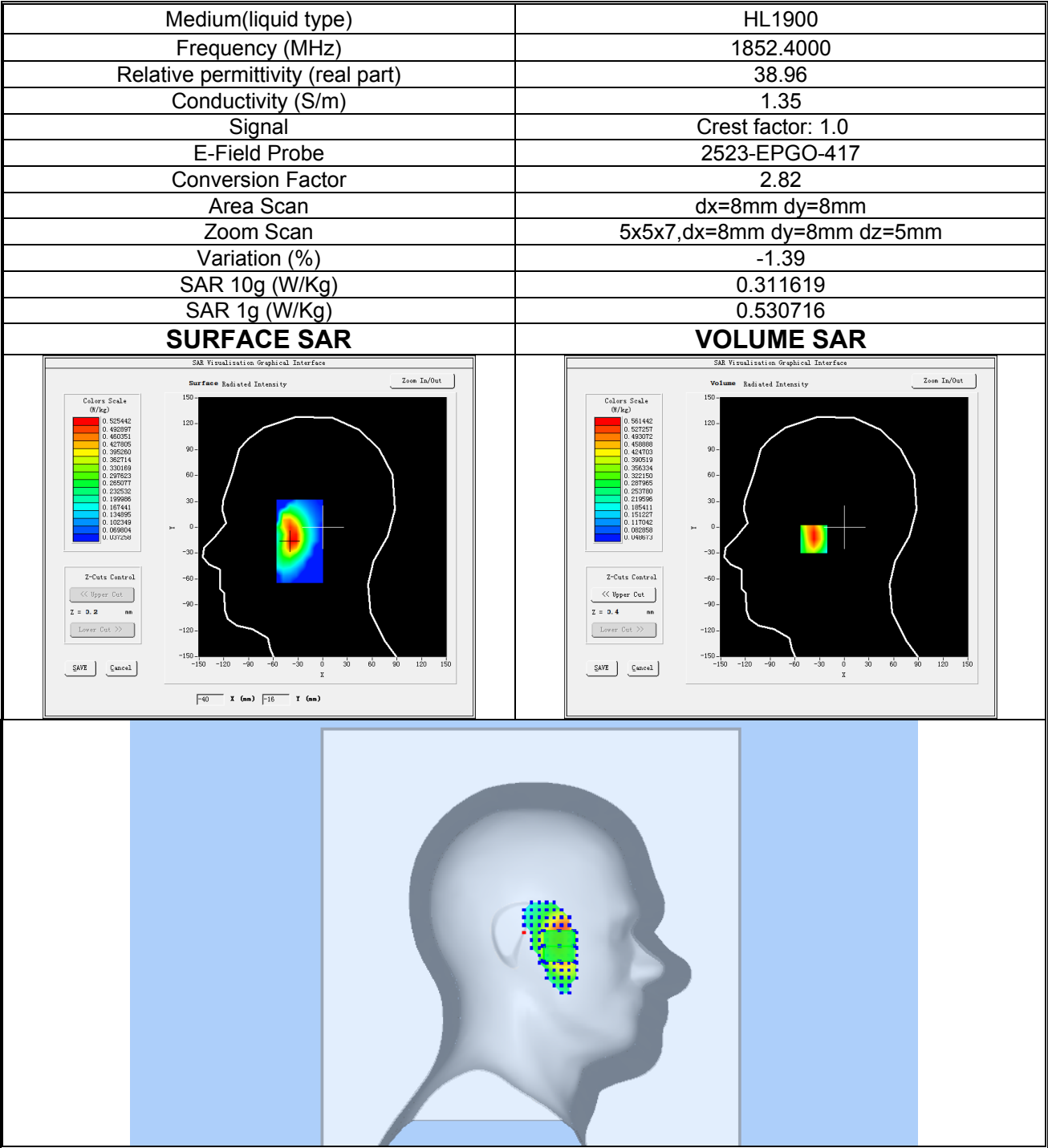
Plot 5: WCDMA BAND II, Low channel (Left Head Cheek) Product Description: Smart Phone Test Date: 2025-11-10
