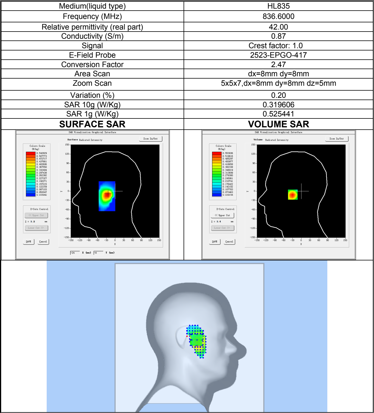
Plot 9: WCDMA BAND V, Middle channel (Left Head Cheek) Product Description: Smart Phone Test Date: 2025-10-23
