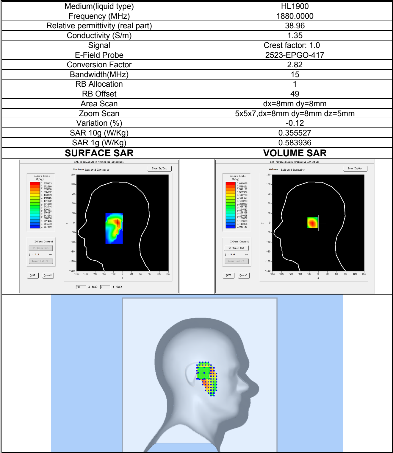
Plot 11:LTE BAND 2, Middle channel (Left Head Cheek) Product Description:Smart Phone Test Date: 2025-11-10
