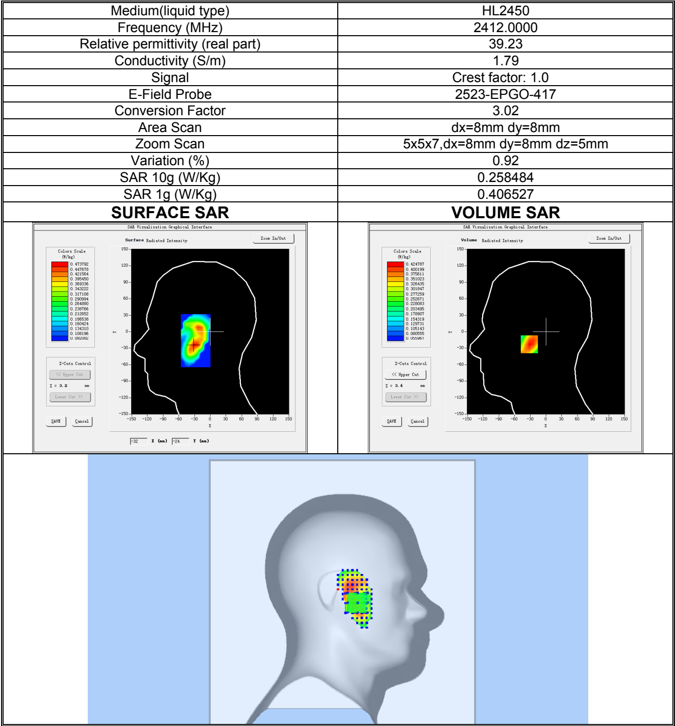
Plot 21:2.4G Wi-Fi, Low channel (Left Head Cheek) Product Description: Smart Phone Test Date: 2025-10-18
