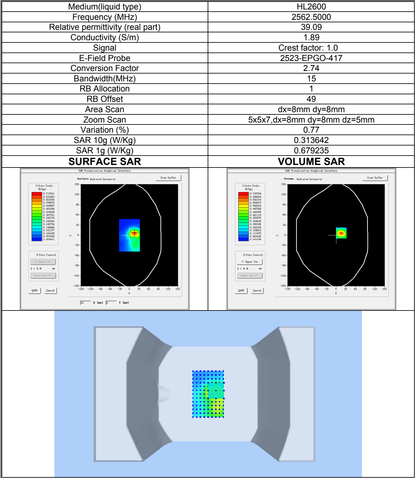
Plot 18: LTE BAND 7, High channel (Body-worn/ Hotspot, Back Side) Product Description: Smart Phone Test Date: 2025-11-07
