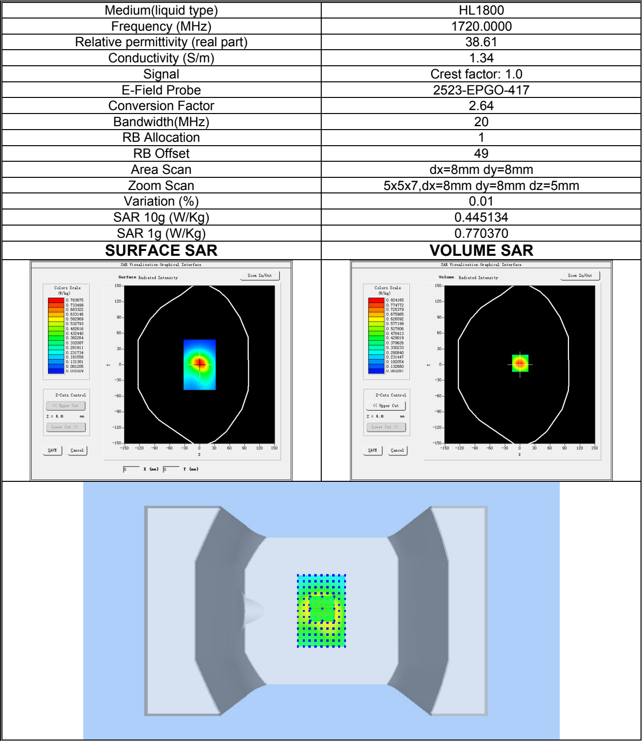
Plot 14: LTE BAND 4, Low channel (Body-worn/ Hotspot, Back Side) Product Description: Smart Phone Test Date: 2025-11-10
