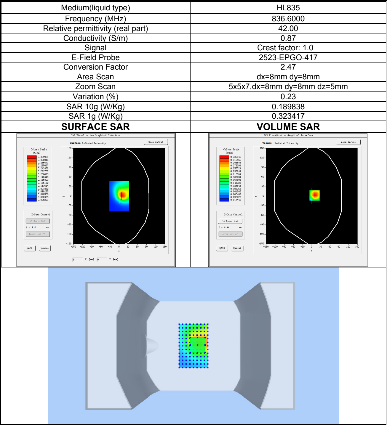
Plot 10: WCDMA BAND V, Middle channel (Body-worn/Hotspot, Back Side) Product Description: Smart Phone Test Date: 2025-10-23
