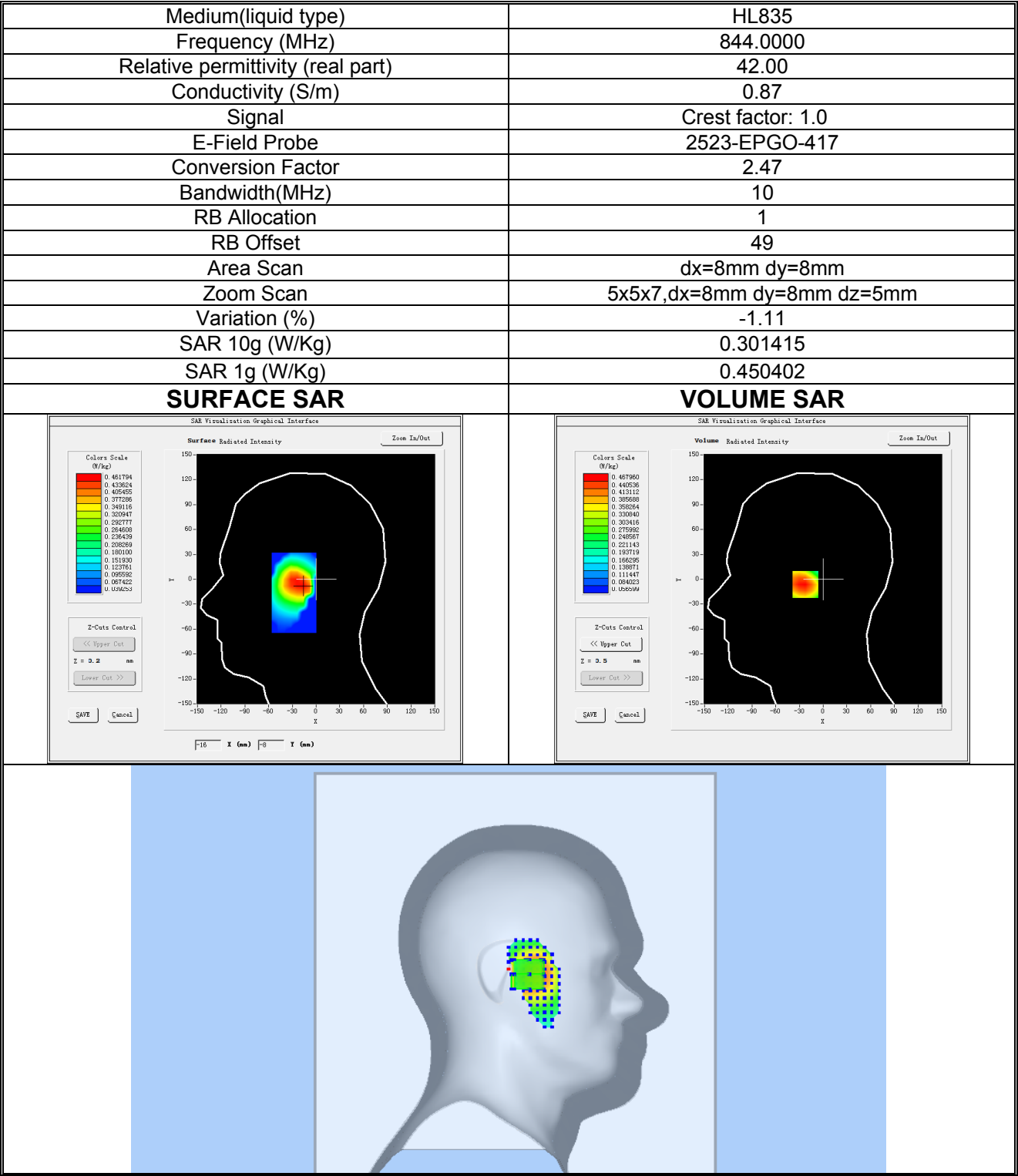
Plot 15:LTE BAND 5, High channel (Left Head Cheek) Product Description: Smart Phone Test Date: 2025-10-23
