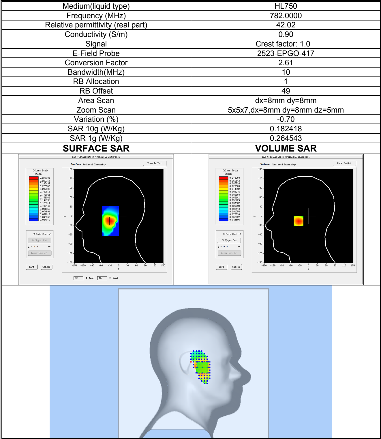
Plot 19:LTE BAND 13, Low channel (Left Head Cheek) Product Description: Smart Phone Test Date: 2025-10-22
