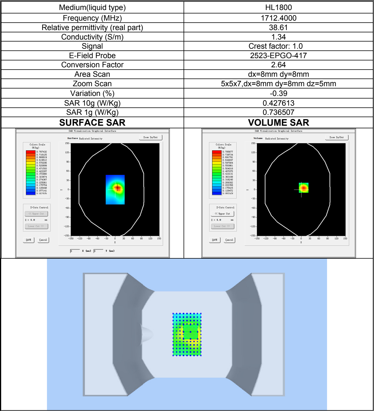
Plot 8: WCDMA BAND IV, Low channel (Body-worn/Hotspot, Back Side) Product Description: Smart Phone Test Date: 2025-11-10
