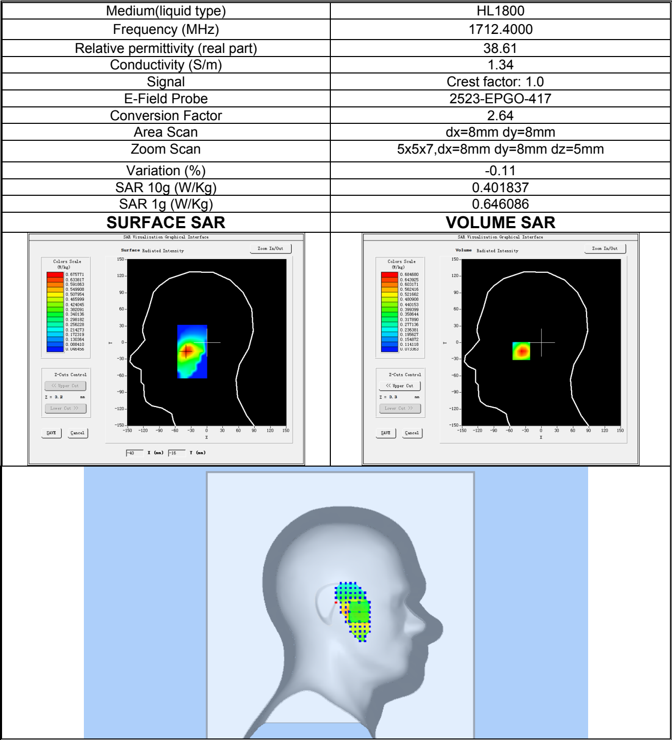
Plot 7: WCDMA BAND IV, Low channel (Left Head Cheek) Product Description: Smart Phone Test Date: 2025-11-10
