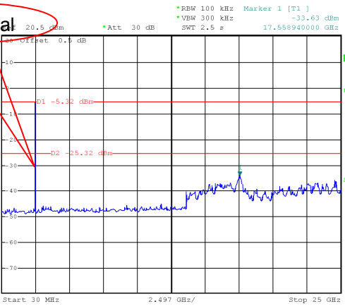
Mode: channel 39
