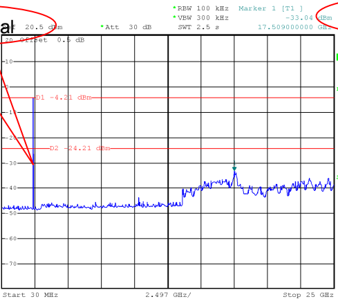
Mode: channel 0
