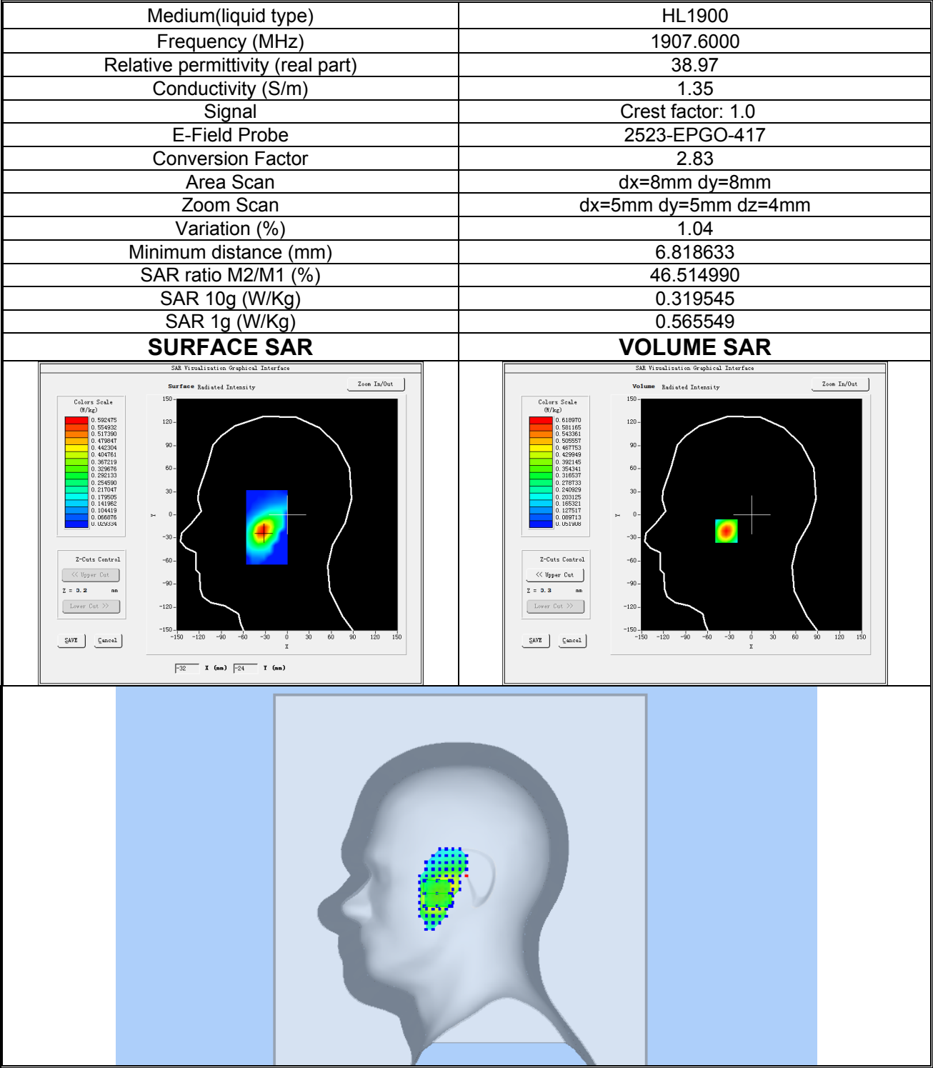
Plot 5: WCDMA BAND II, High channel (Right Head Cheek) Product Description: Smart Phone Test Date: 2026-08-15
