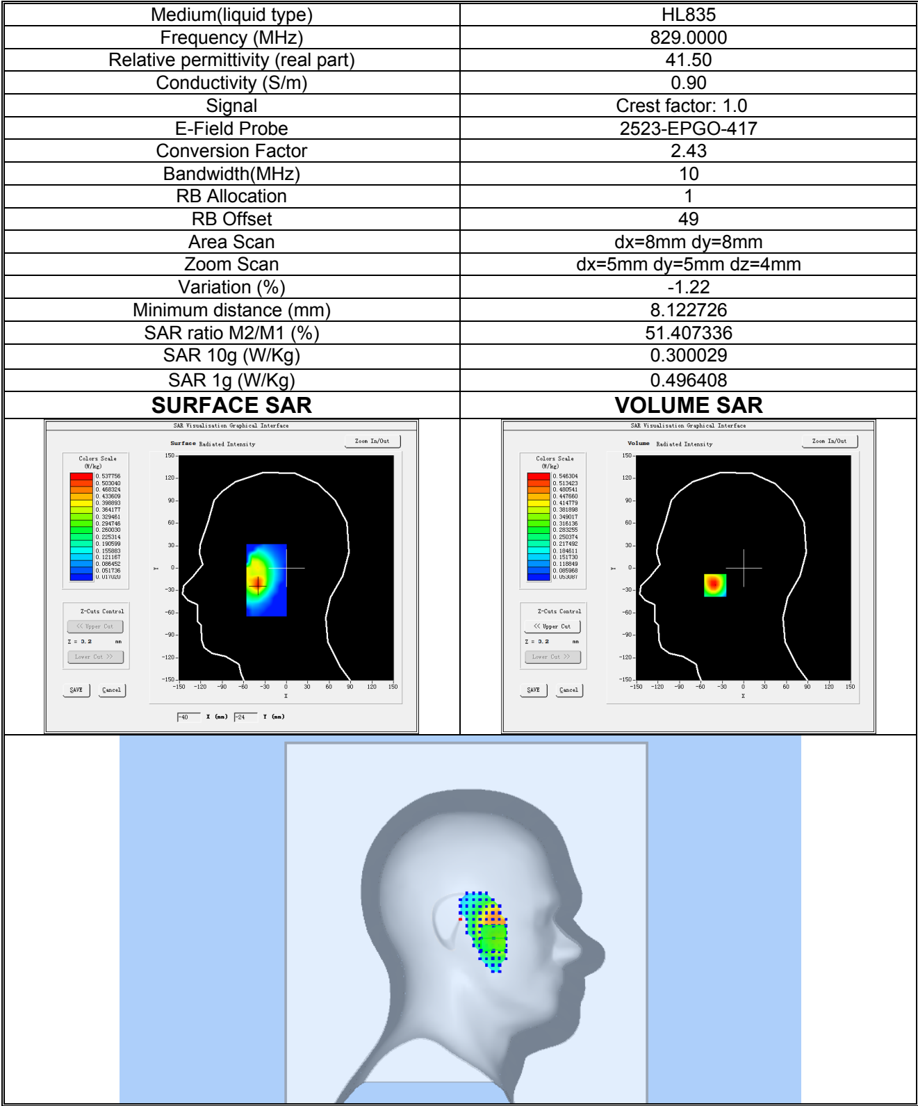
Plot 15:LTE BAND 5, Low channel (Left Head Cheek) Product Description: Smart Phone Test Date: 2026-08-13
