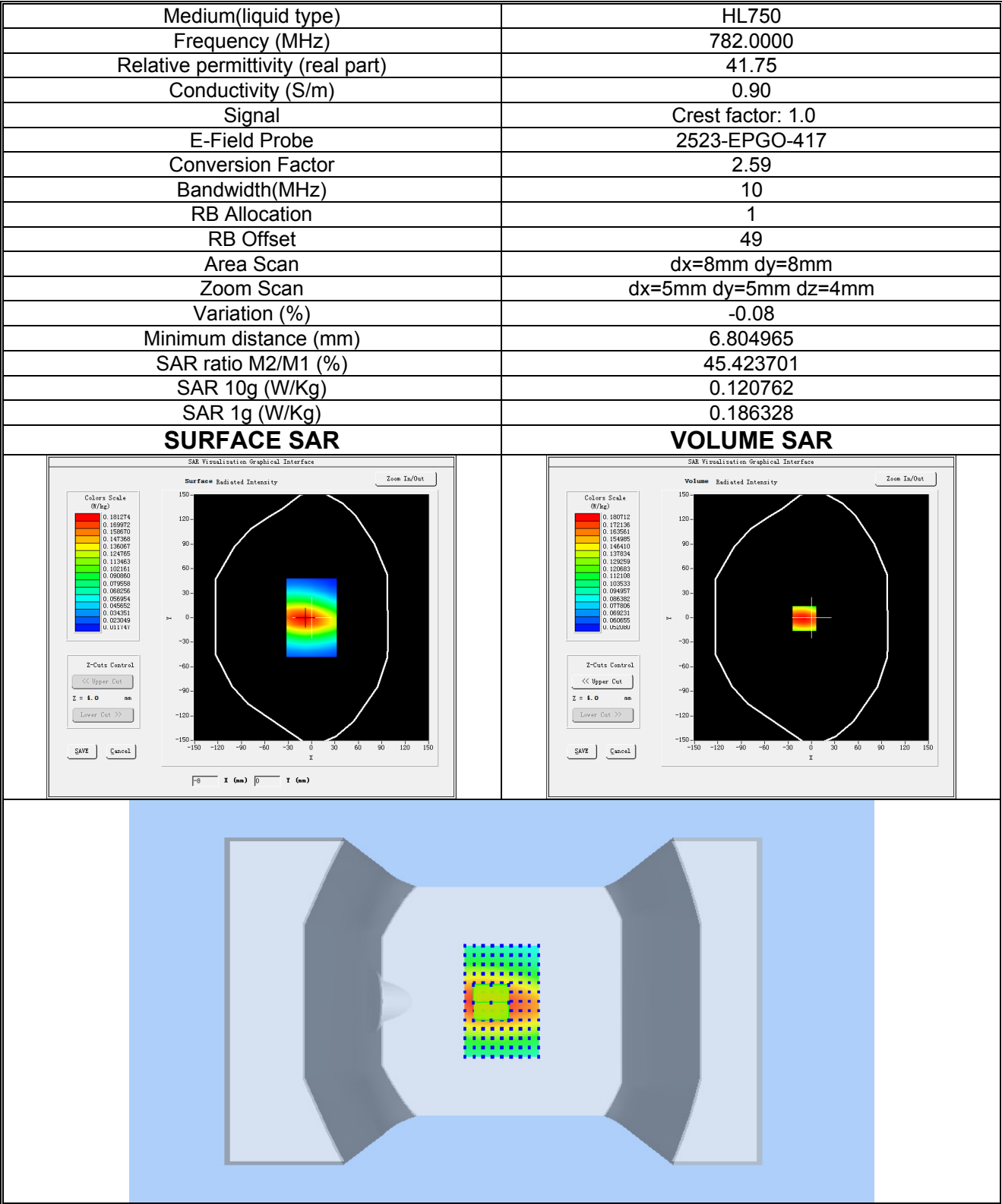
Plot 20: LTE BAND 13, Low channel (Body-worn/ Hotspot, Left Edge) Product Description: Smart Phone Test Date: 2026-08-16
