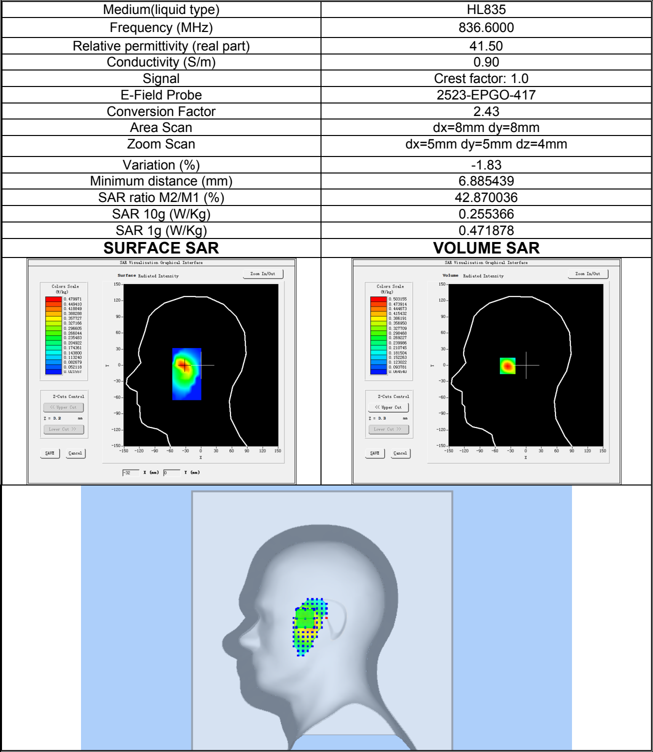
Plot 9: WCDMA BAND V, Middle channel (Right Head Cheek) Product Description: Smart Phone Test Date: 2026-08-13
