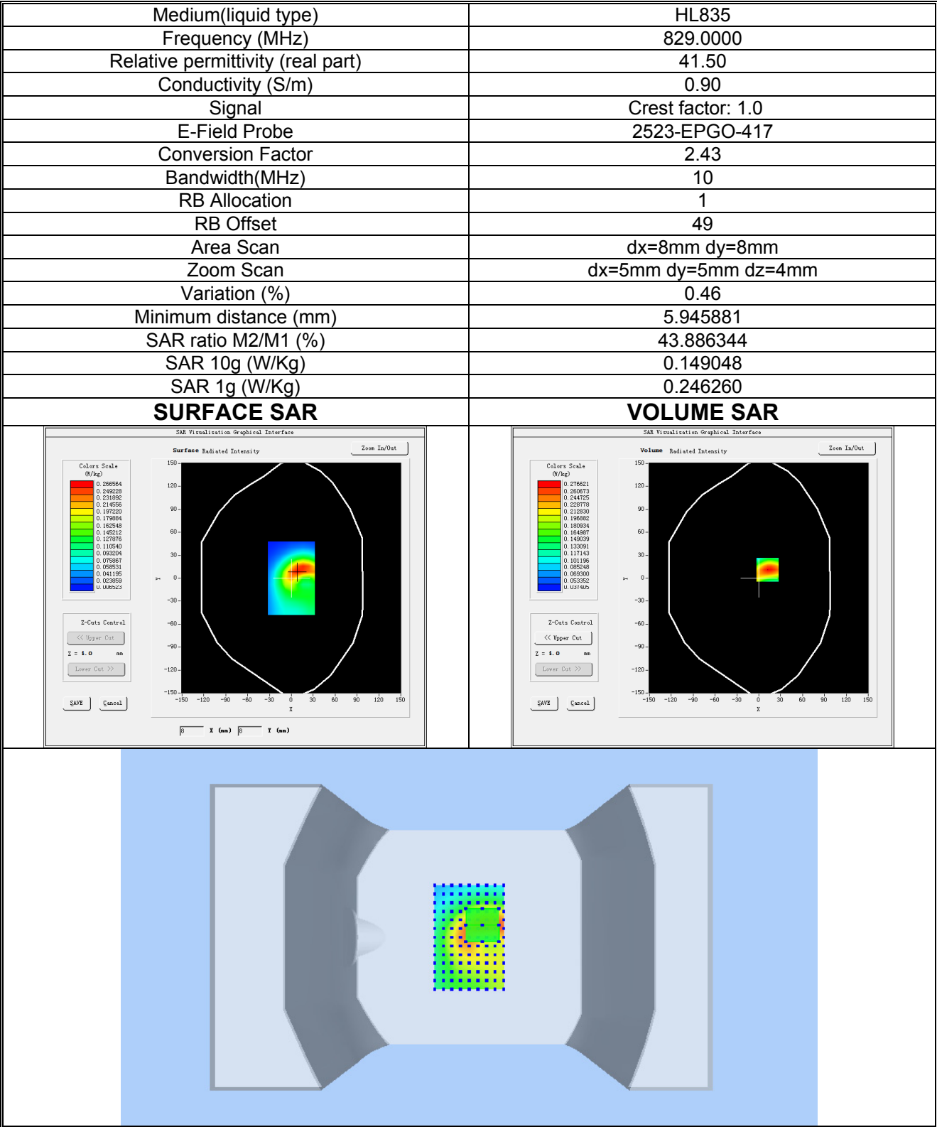
Plot 16: LTE BAND 5, Low channel (Body-worn/ Hotspot, Back Side) Product Description: Smart Phone Test Date: 2026-08-13
