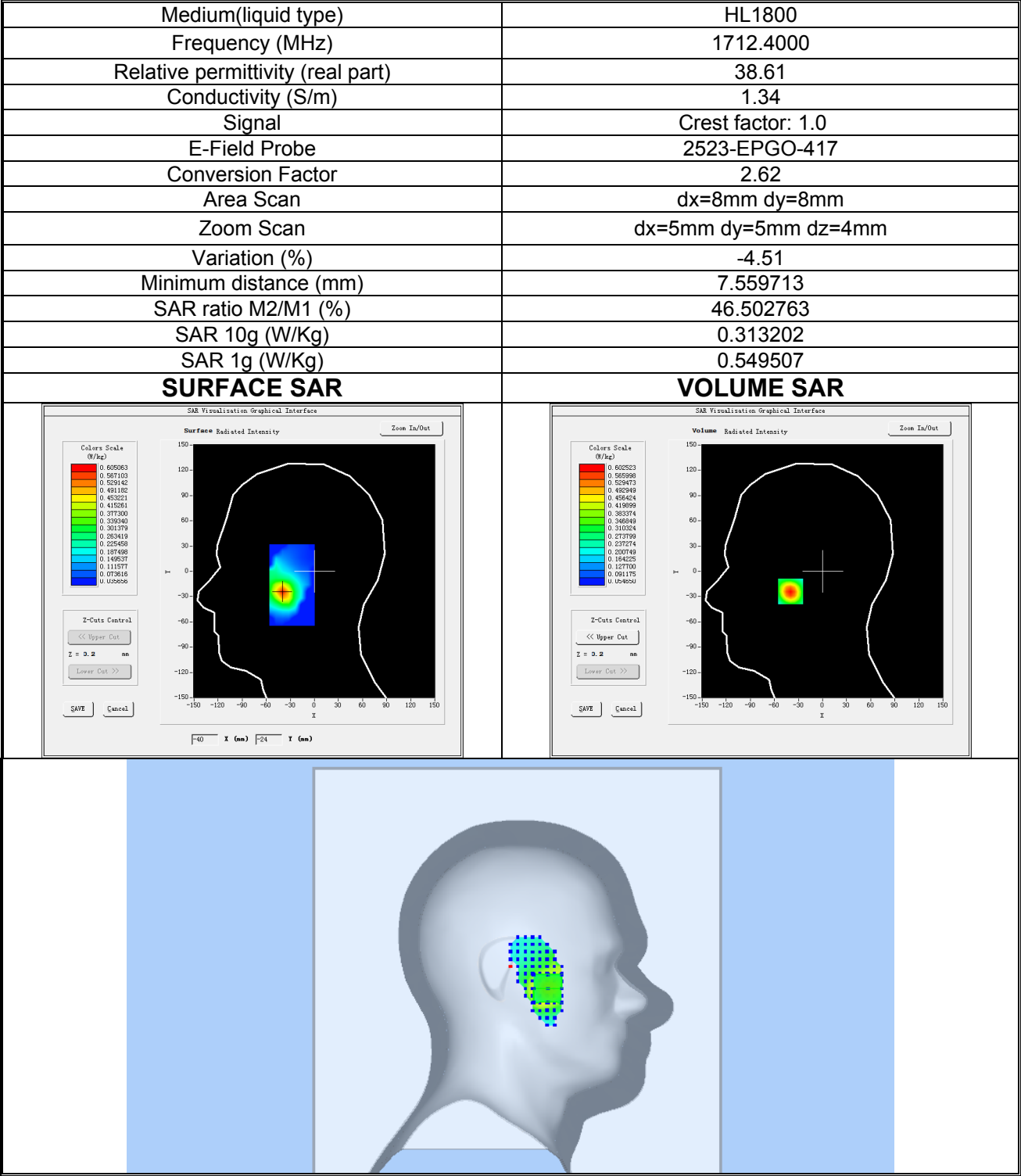
Plot 7: WCDMA BAND IV, Low channel (Left Head Cheek) Product Description: Smart Phone Test Date: 2026-08-19
