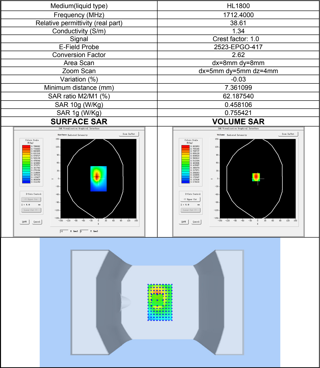
Plot 8: WCDMA BAND IV, Low channel (Body-worn/Hotspot, Back Side) Product Description: Smart Phone Test Date: 2026-08-19
