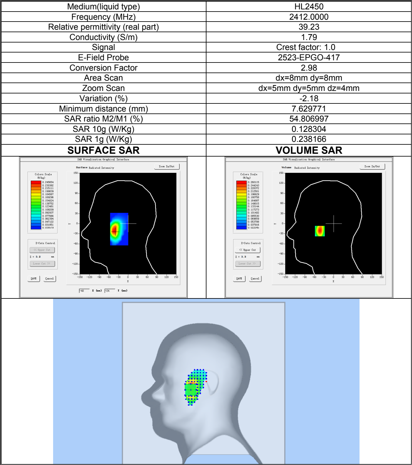
Plot 21:2.4G Wi-Fi, Low channel (Right Head Cheek) Product Description: Smart Phone Test Date: 2026-08-13
