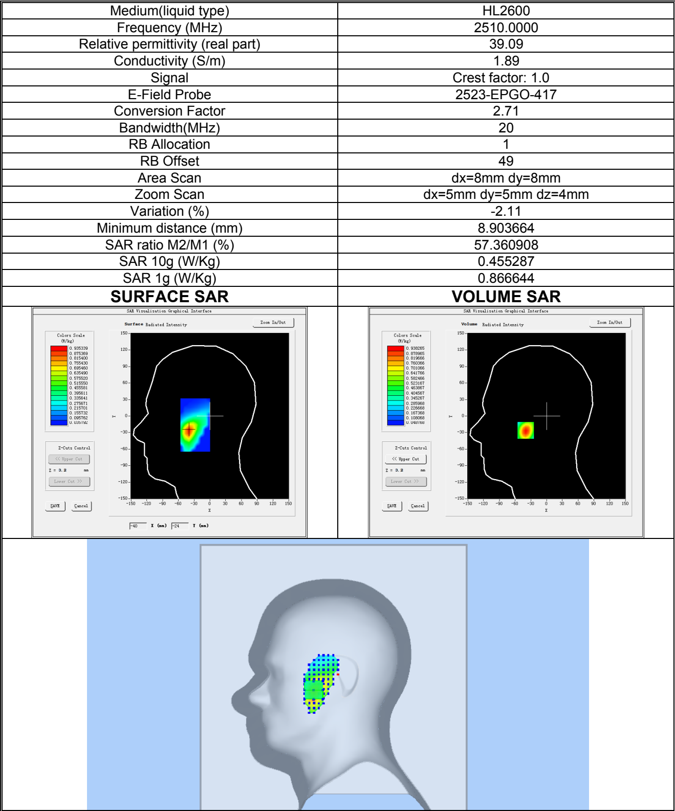
Plot 17:LTE BAND 7, Low channel (Right Head Cheek) Product Description: Smart Phone Test Date: 2026-08-17
