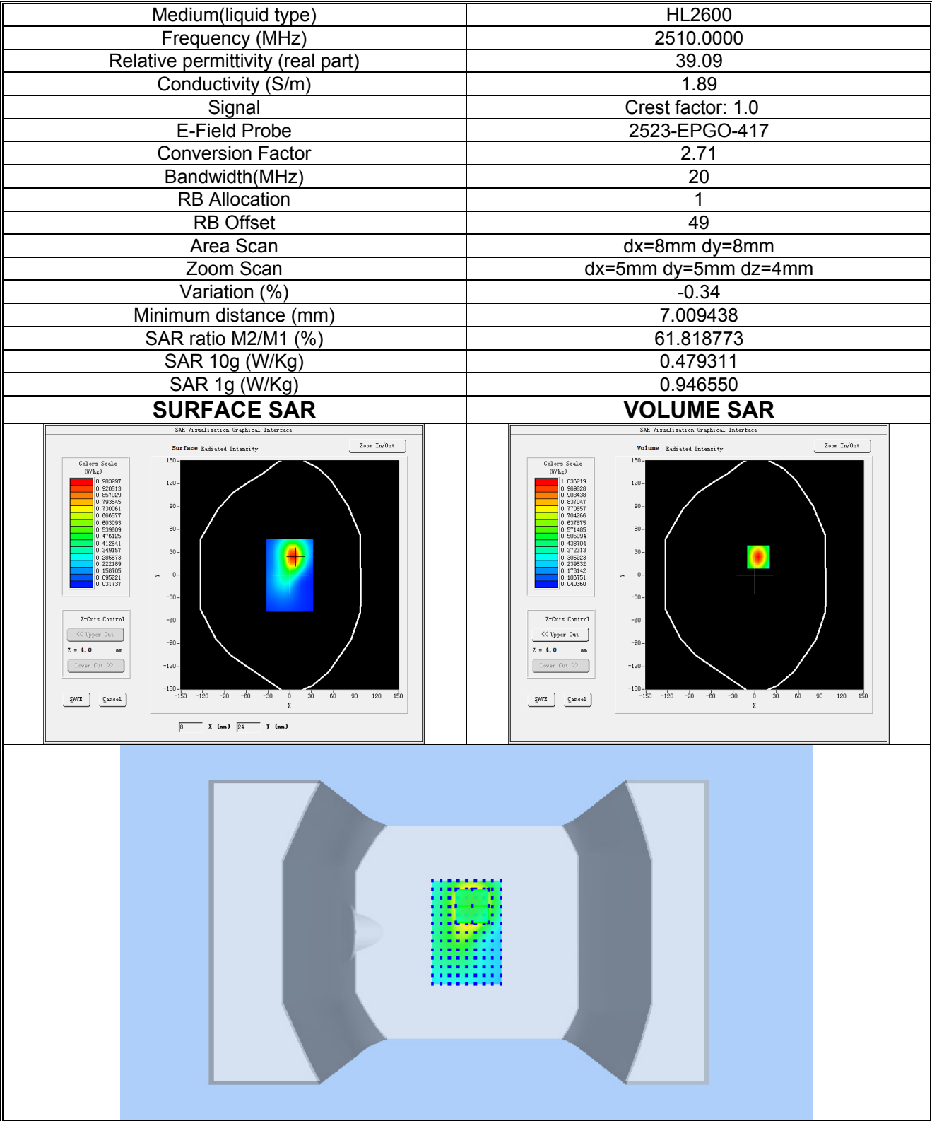
Plot 18: LTE BAND 7, Low channel (Body-worn/ Hotspot, Bottom Edge) Product Description: Smart Phone Test Date: 2026-08-17
