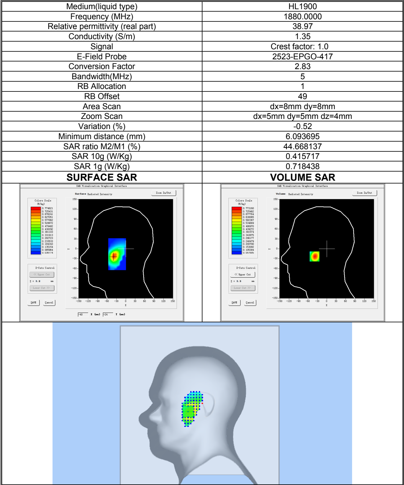
Plot 11:LTE BAND 2, Middle channel (Right Head Cheek) Product Description:Smart Phone Test Date: 2026-08-15
