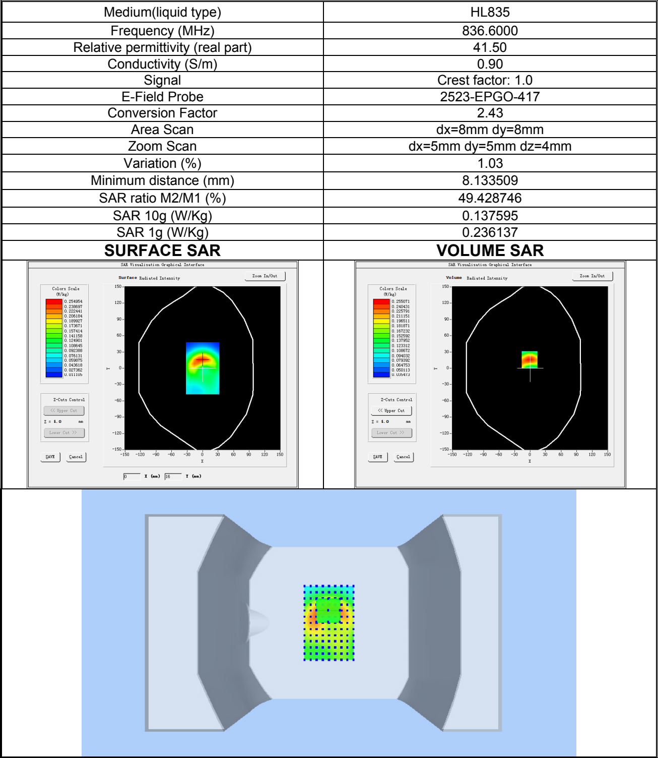
Plot 10: WCDMA BAND V, Middle channel (Body-worn/Hotspot, Back Side) Product Description: Smart Phone Test Date: 2026-08-13
