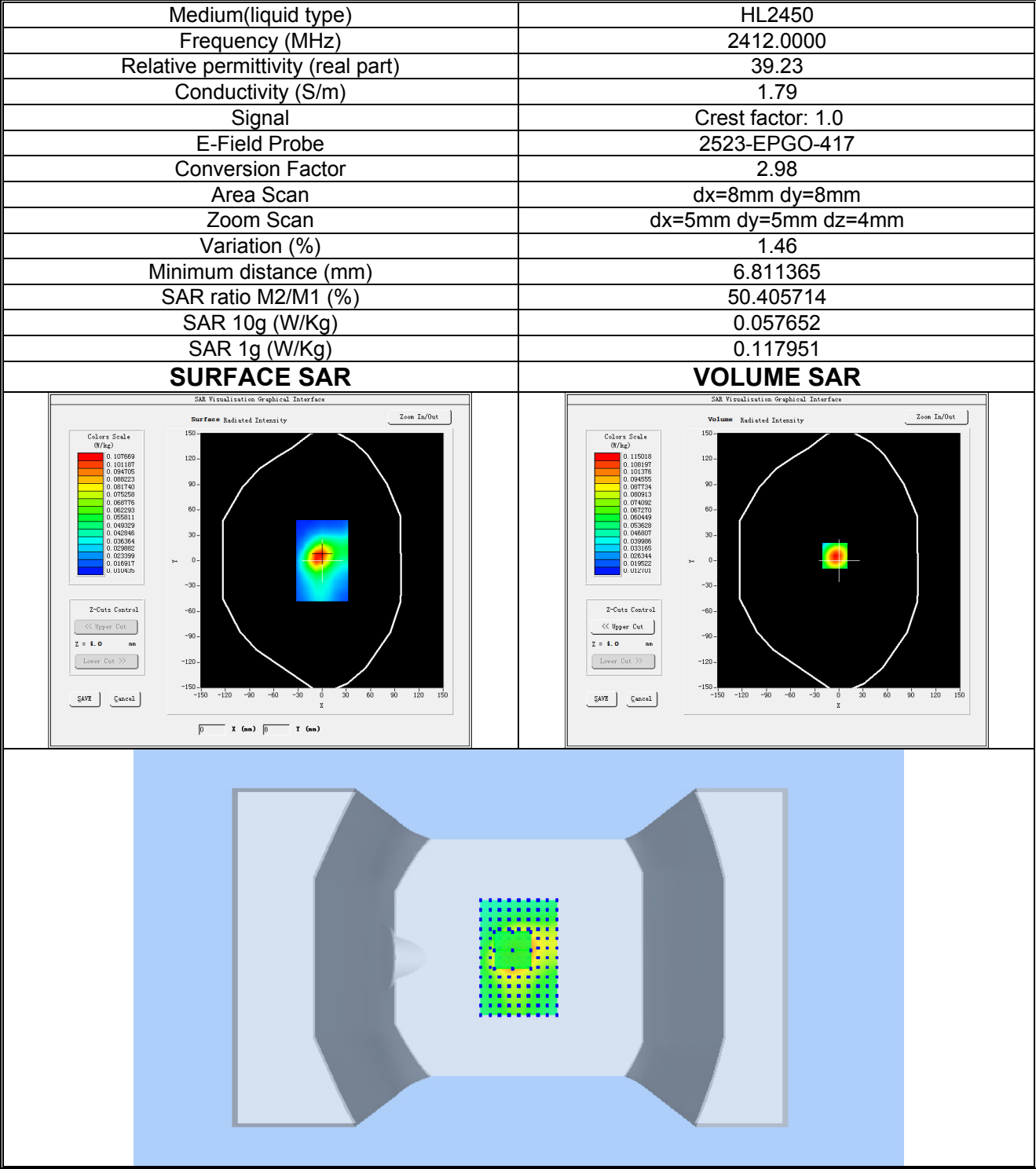
Plot 22: 2.4G Wi-Fi, Low channel (Body-worn/ Hotspot, Back Side) Product Description: Smart Phone Test Date: 2026-08-13
