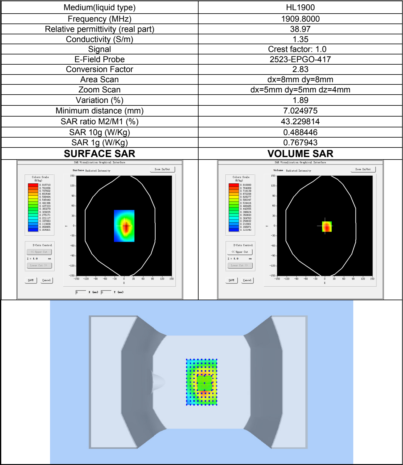
Plot 4: GSM 1900, High channel (Body-worn /Hotspot, Back Side) Product Description: Smart Phone Test Date: 2026-08-15
