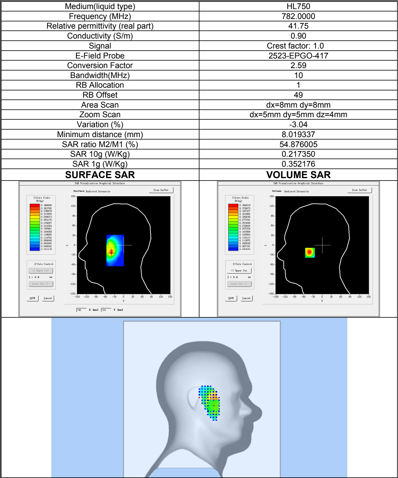
Plot 19:LTE BAND 13, Low channel (Left Head Cheek) Product Description: Smart Phone Test Date: 2026-08-16
