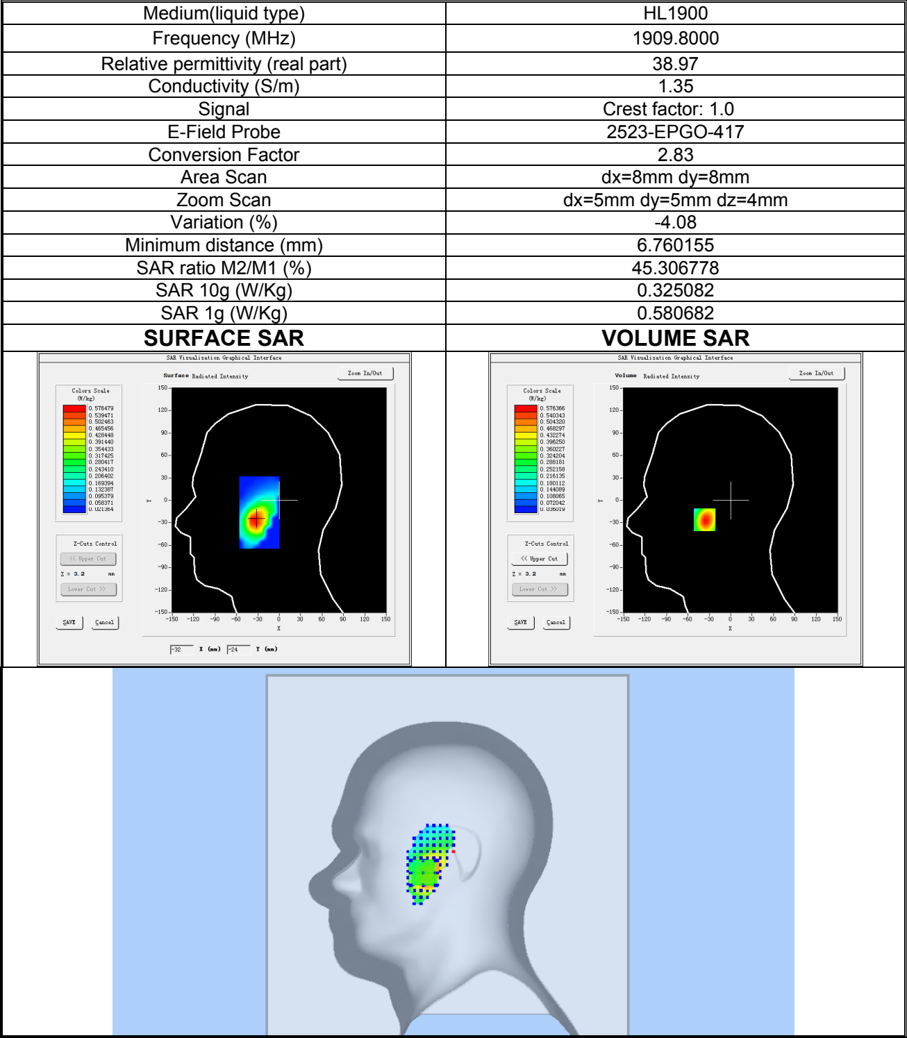
Plot 3: GSM 1900, High channel (Right Head Cheek) Product Description: Smart Phone Test Date: 2026-08-15
