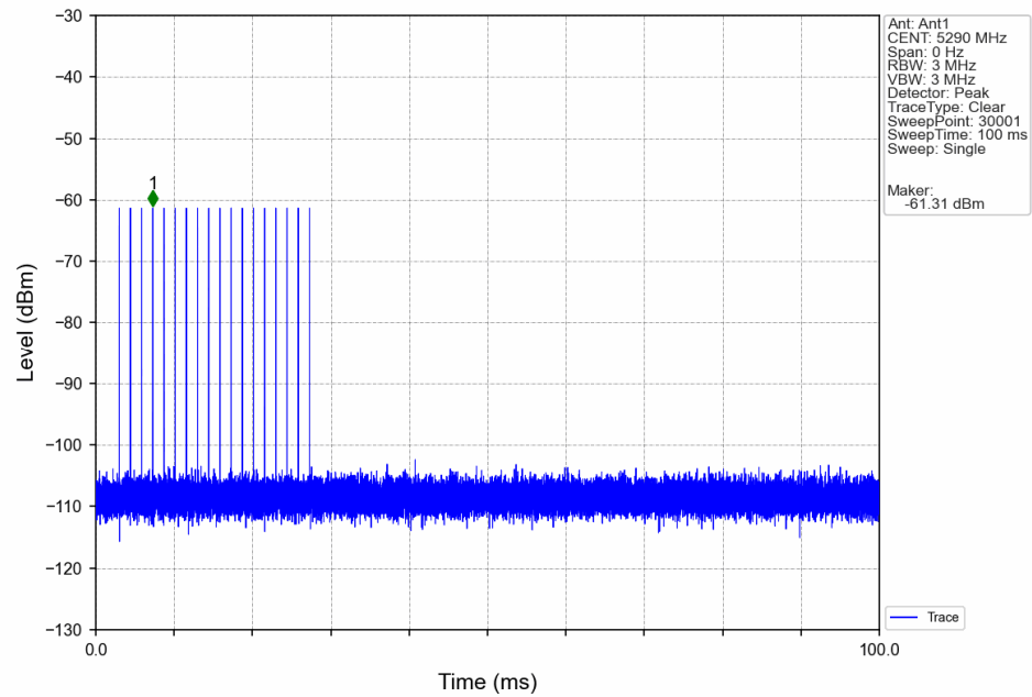
Radar Signal 5290
