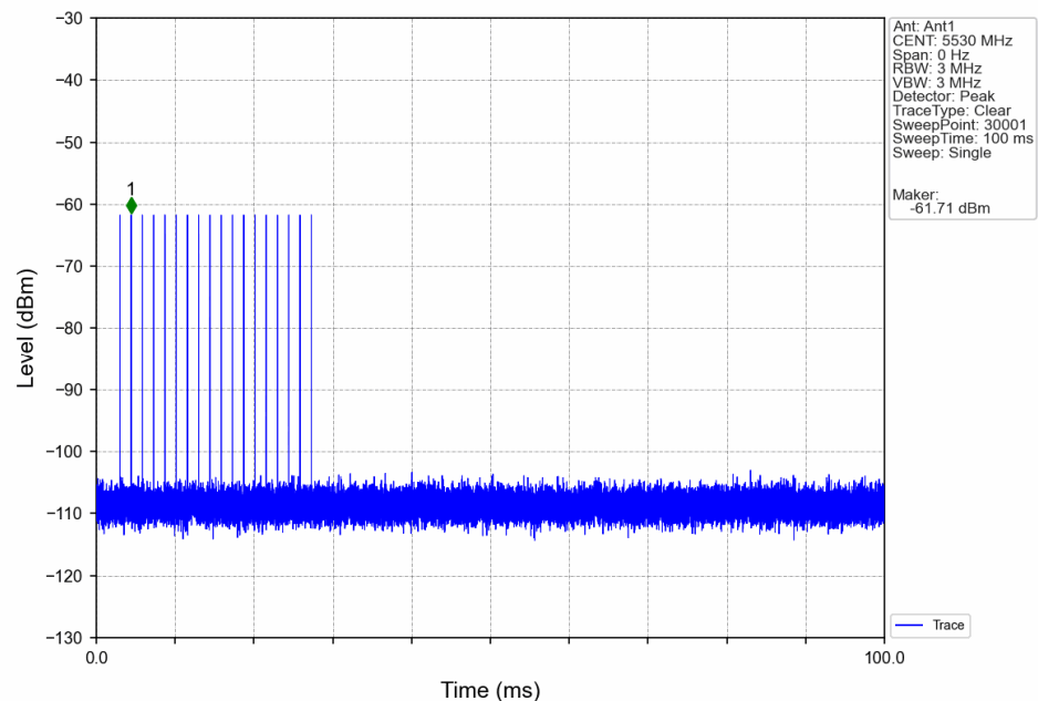
Radar Signal 5530
