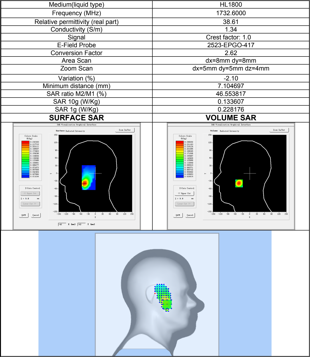
Plot 7: WCDMA BAND IV, Middle channel (Left Head Cheek) Product Description: Smart Phone Test Date: 2026-08-14
