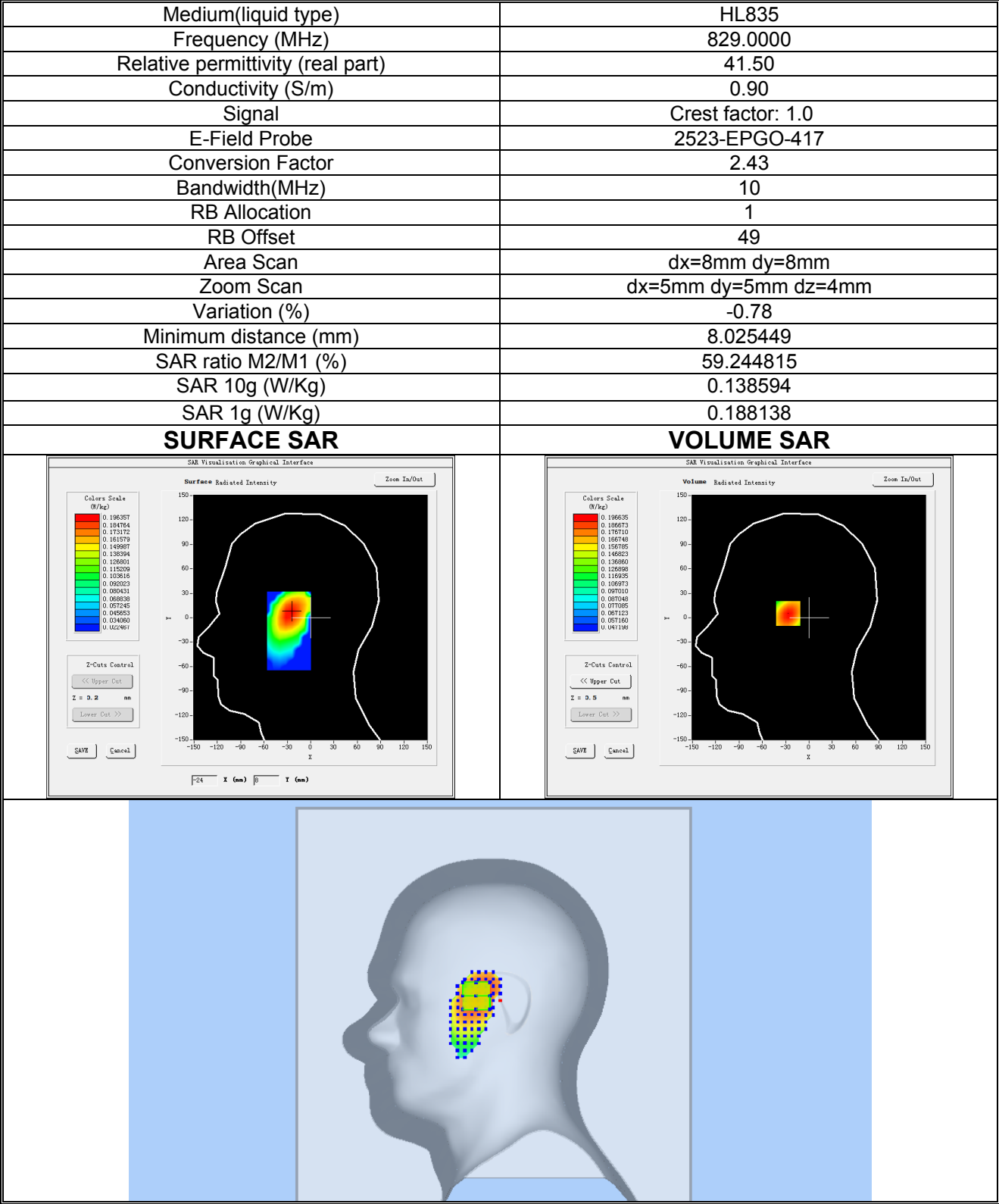
Plot 15:LTE BAND 5, Low channel (Right Head Cheek) Product Description: Smart Phone Test Date: 2026-08-13
