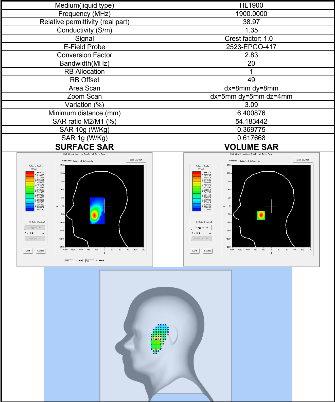
Plot 11:LTE BAND 2, High channel (Right Head Cheek) Product Description:Smart Phone Test Date: 2026-08-13
