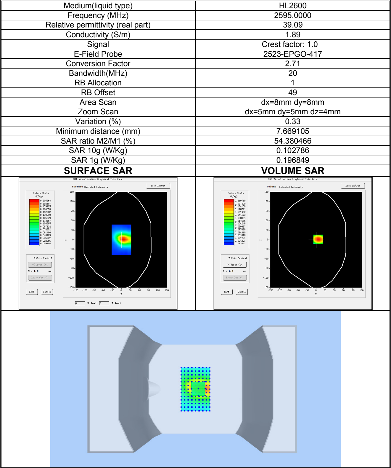
Plot 24: LTE BAND 38, Middle channel (Body-worn/ Hotspot, Left Edge) Product Description: Smart Phone Test Date: 2026-08-15
