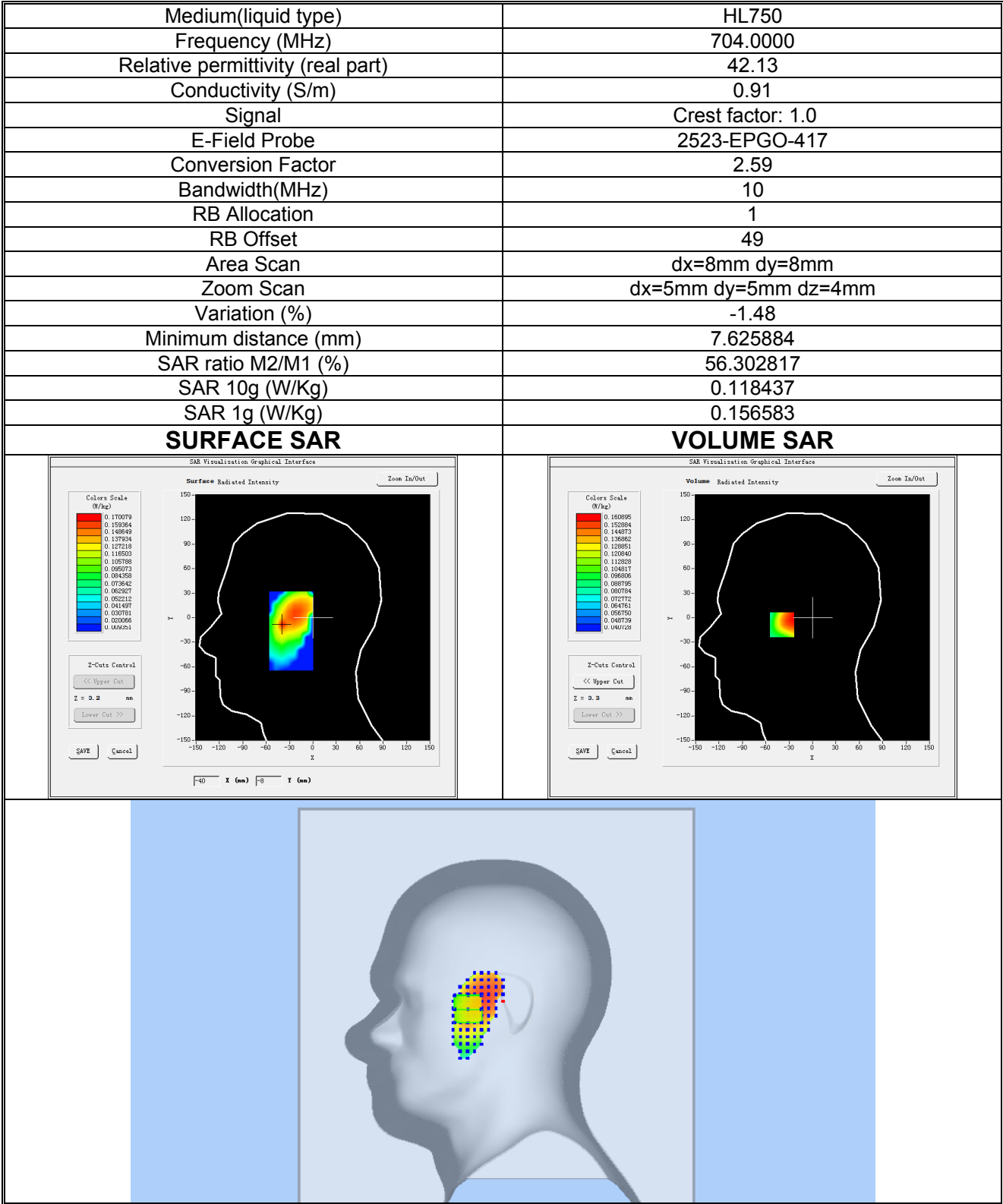
Plot 19:LTE BAND 12, Low channel (Right Head Cheek) Product Description: Smart Phone Test Date: 2026-08-16
