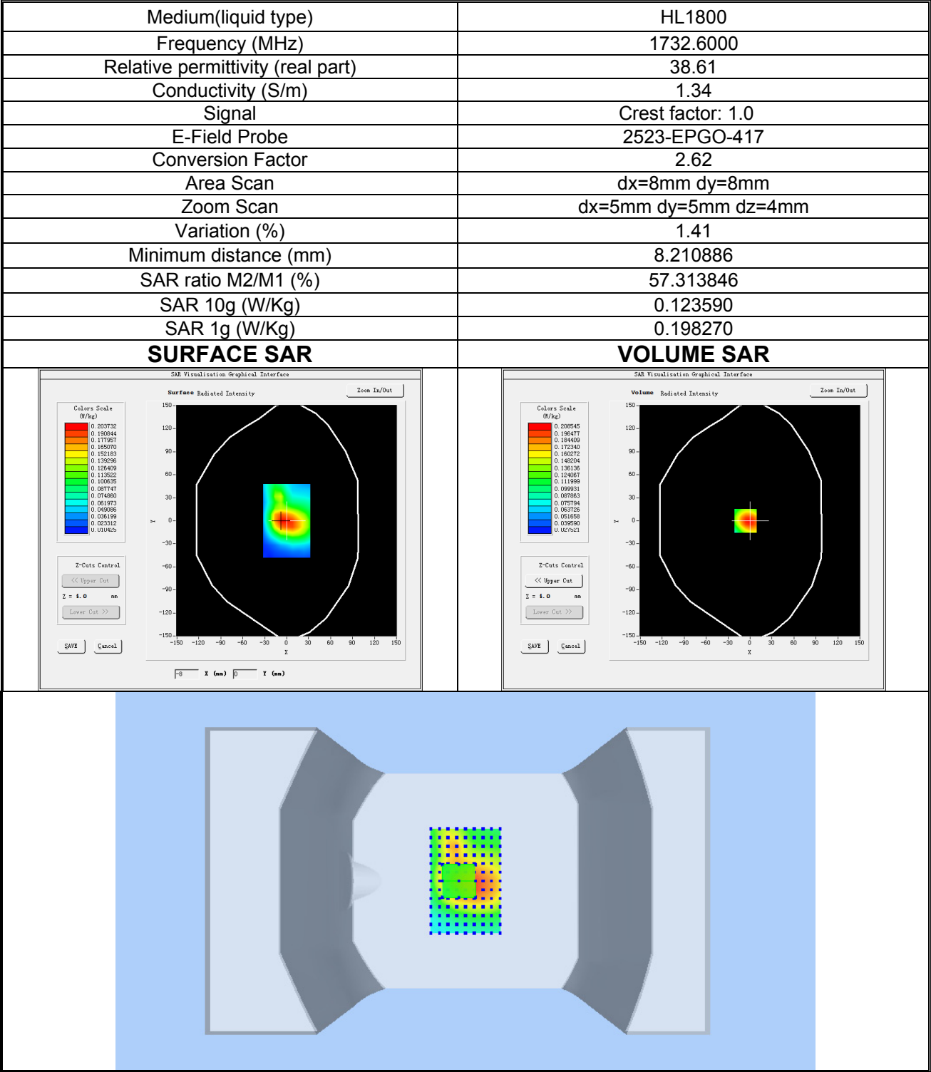
Plot 8: WCDMA BAND IV, Middle channel (Body-worn/Hotspot, Back Side) Product Description: Smart Phone Test Date: 2026-08-14
