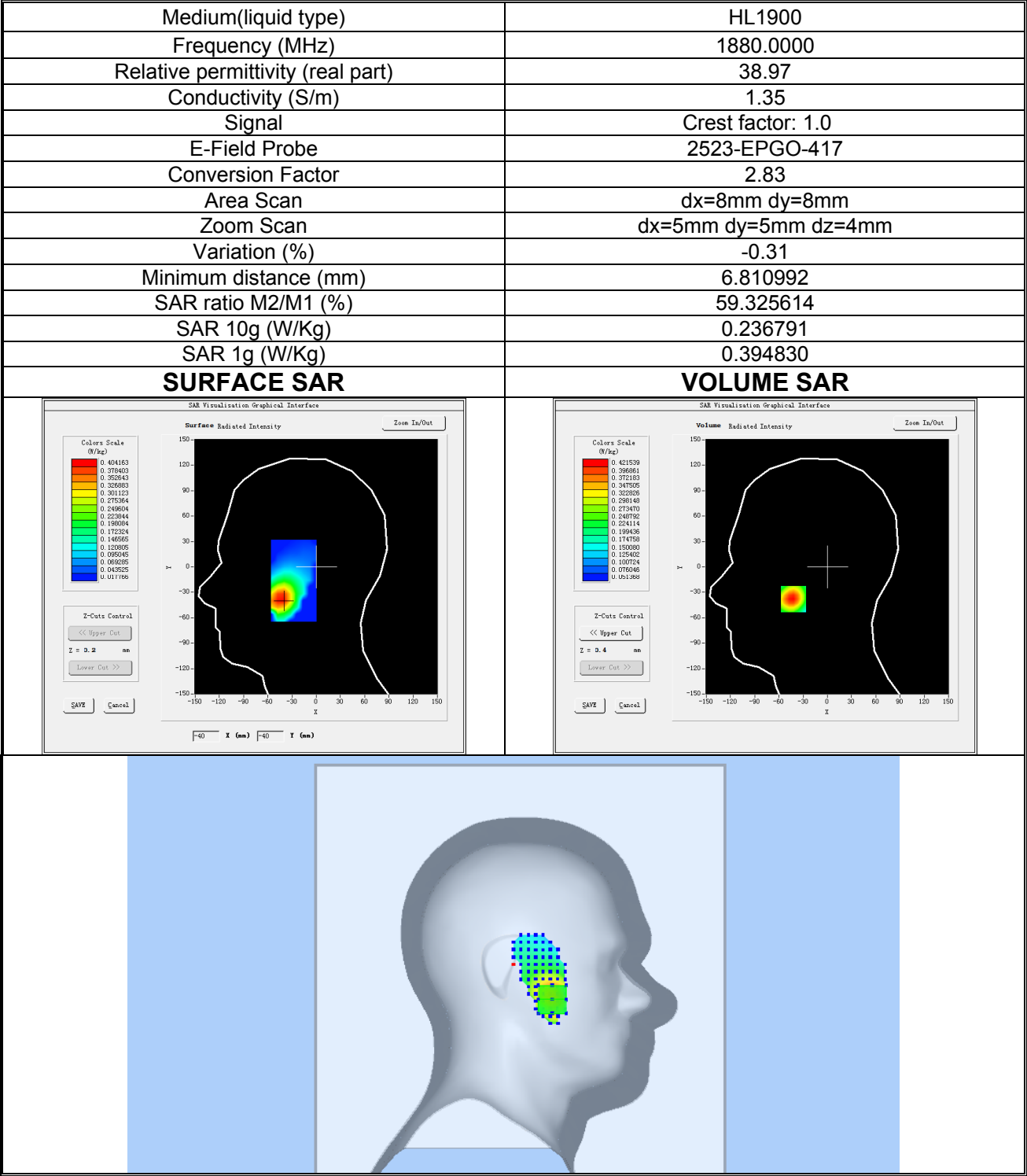
Plot 5: WCDMA BAND II, Middle channel (Left Head Cheek) Product Description: Smart Phone Test Date: 2026-08-13
