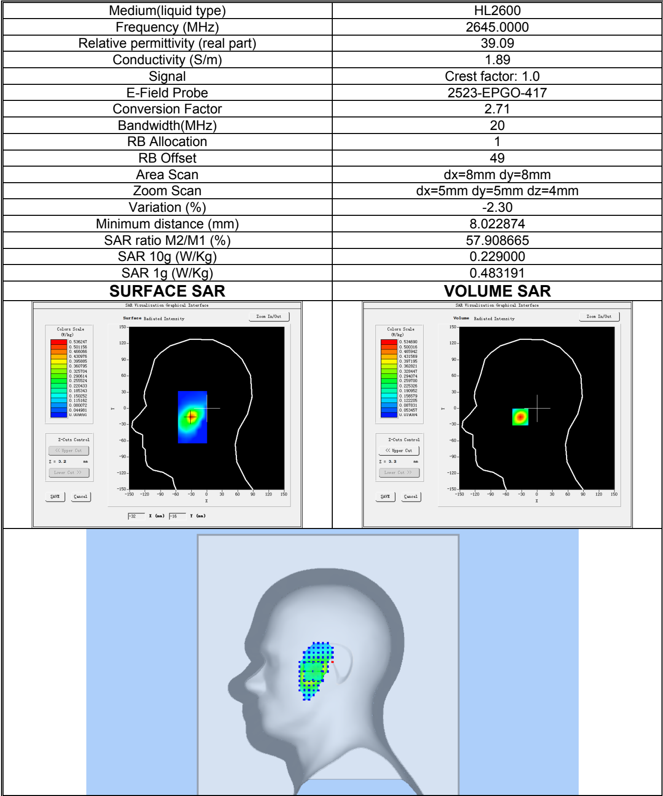
Plot 29:LTE BAND 41, High channel (Right Head Cheek) Product Description: Smart Phone Test Date: 2026-08-15
