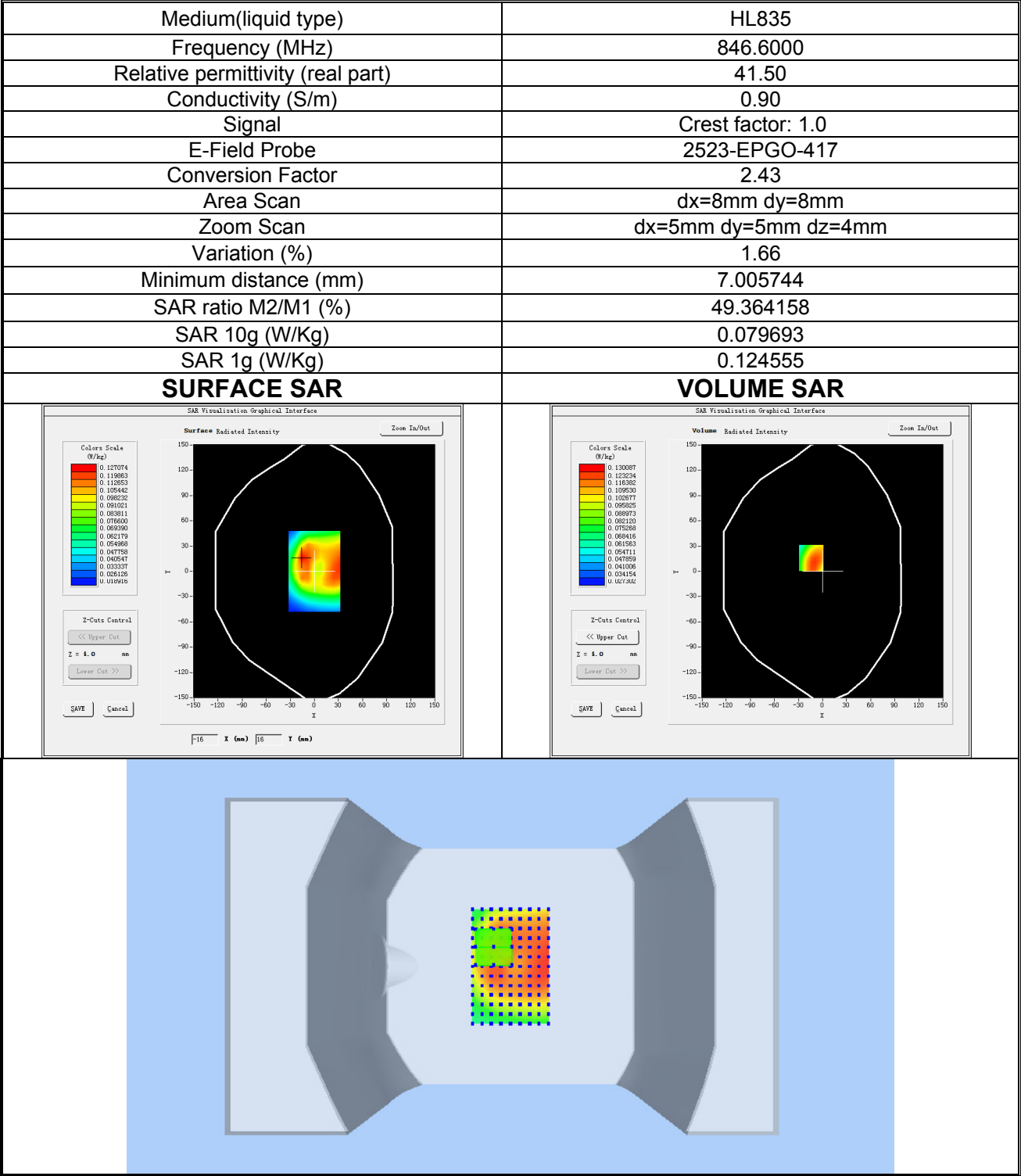
Plot 10: WCDMA BAND V, High channel (Body-worn/Hotspot, Front Side) Product Description: Smart Phone Test Date: 2026-08-13
