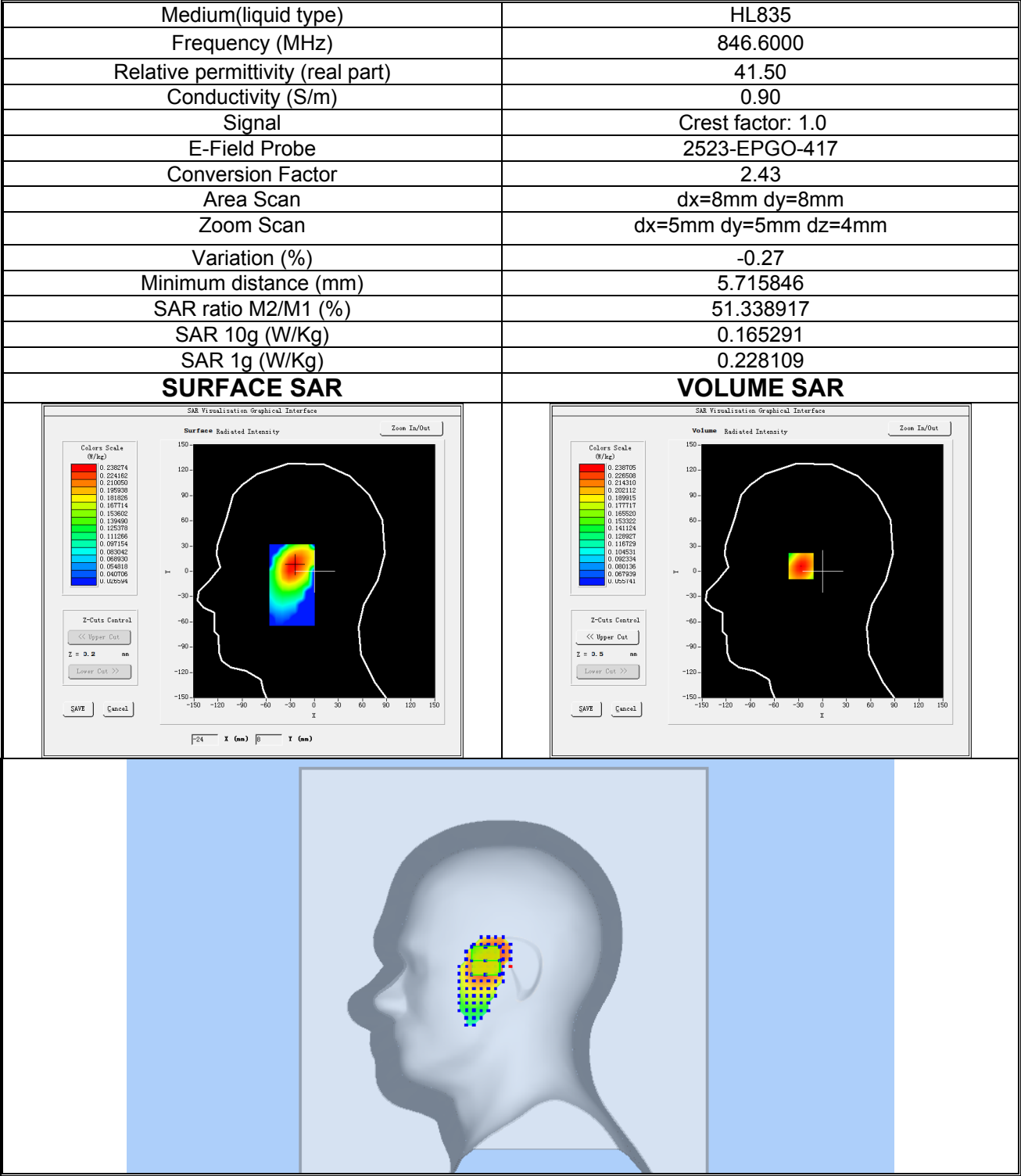
Plot 9: WCDMA BAND V, High channel (Right Head Cheek) Product Description: Smart Phone Test Date: 2026-08-13
