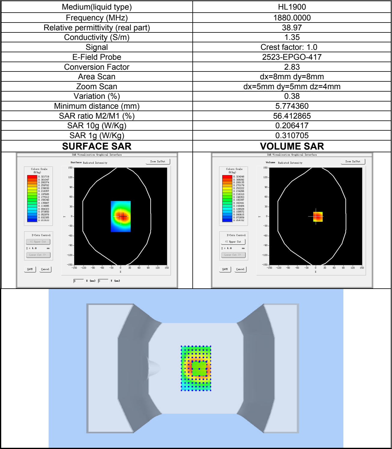
Plot 6: WCDMA BAND II, Middle channel (Body-worn /Hotspot, Back Side) Product Description: Smart Phone Test Date: 2026-08-13
