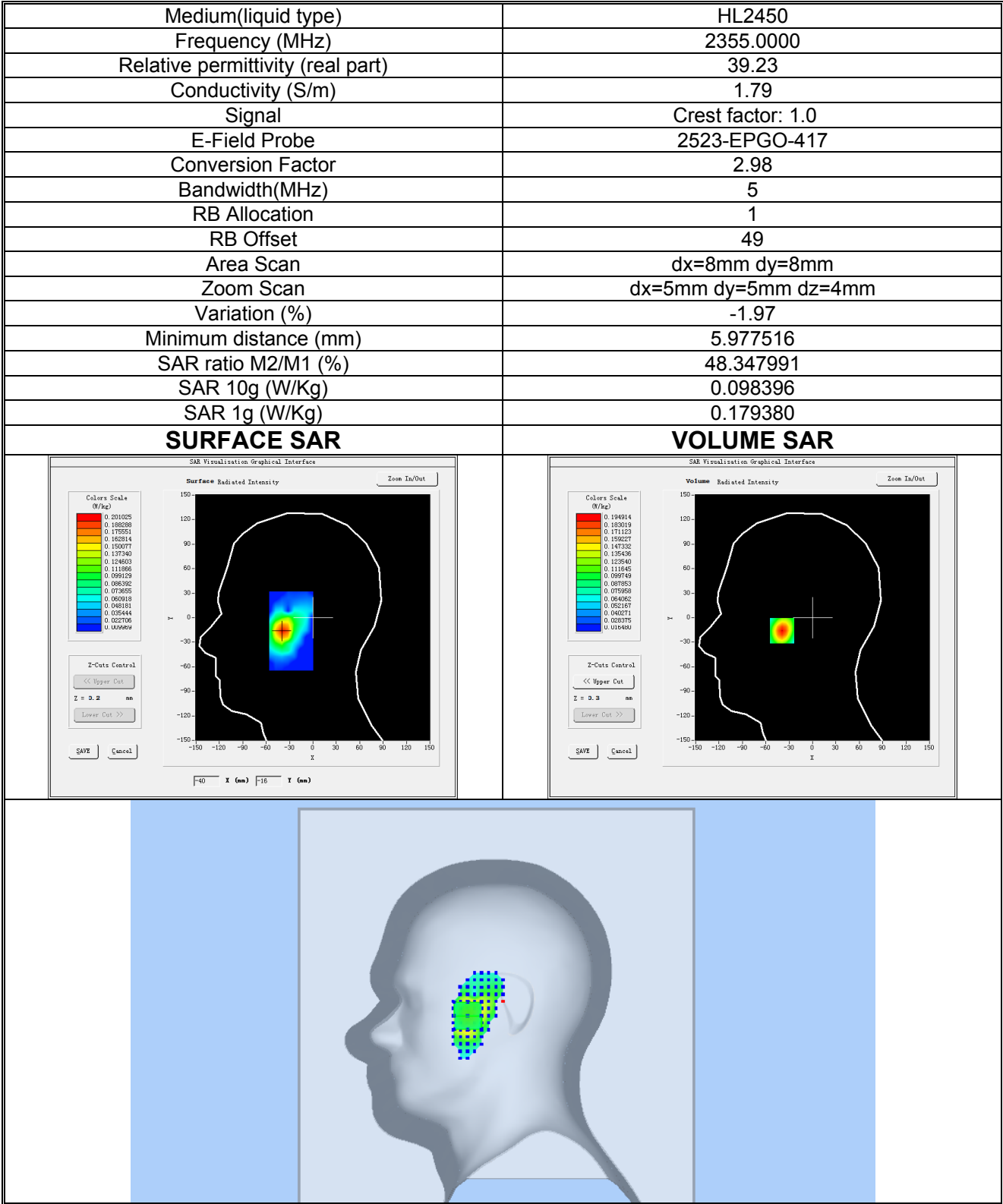
Plot 27:LTE BAND 40(2350-2360), Middle channel (Right Head Cheek) Product Description: Smart Phone Test Date: 2026-08-17
