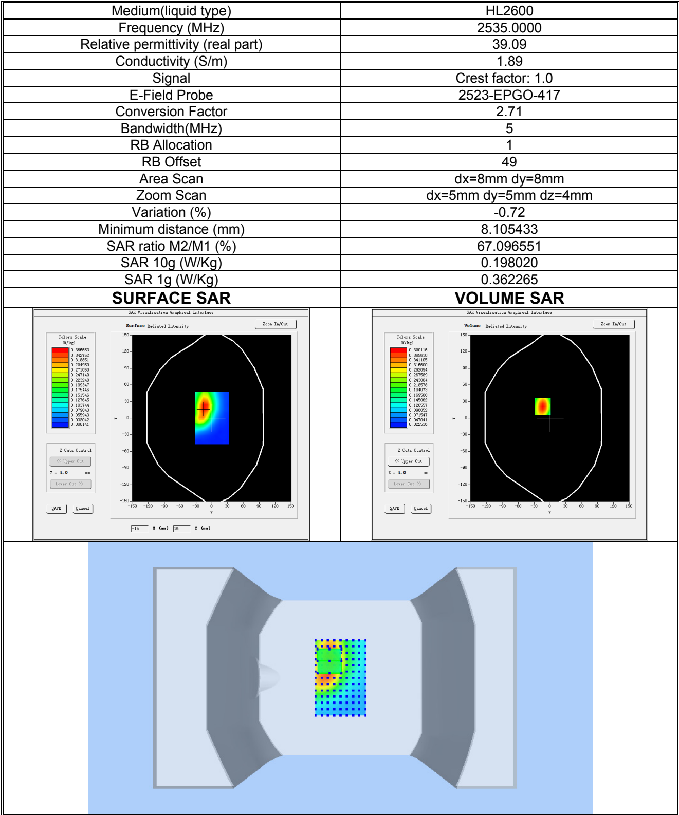
Plot 18: LTE BAND 7, Middle channel (Body-worn/ Hotspot, Back Side) Product Description: Smart Phone Test Date: 2026-08-15
