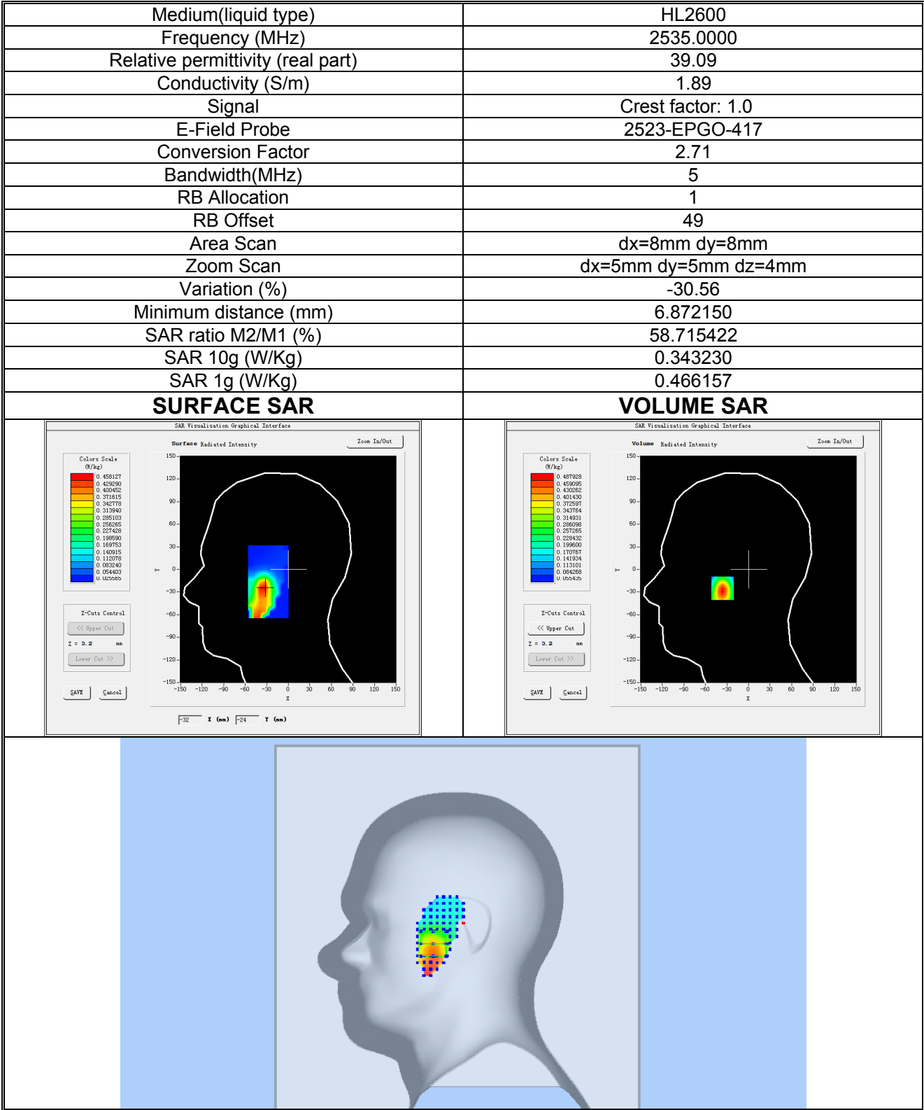
Plot 17:LTE BAND 7, Middle channel (Right Head Cheek) Product Description: Smart Phone Test Date: 2026-08-15
