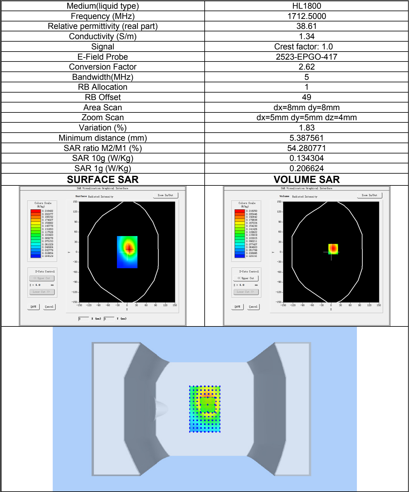
Plot 14: LTE BAND 4, Low channel (Body-worn/ Hotspot, Front Side) Product Description: Smart Phone Test Date: 2026-08-14
