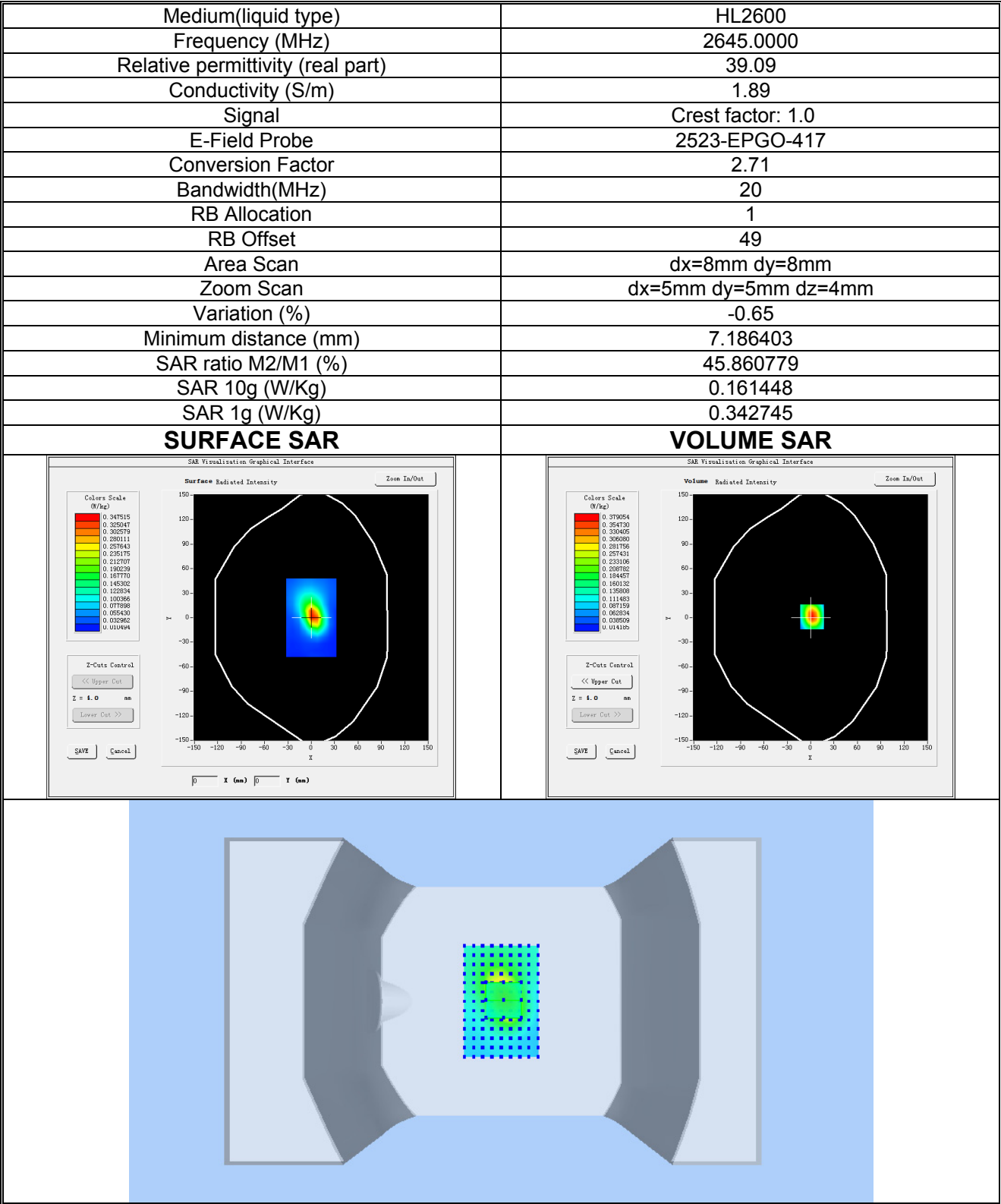
Plot 30: LTE BAND 41, High channel (Body-worn/ Hotspot, Bottom Edge) Product Description: Smart Phone Test Date: 2026-08-15
