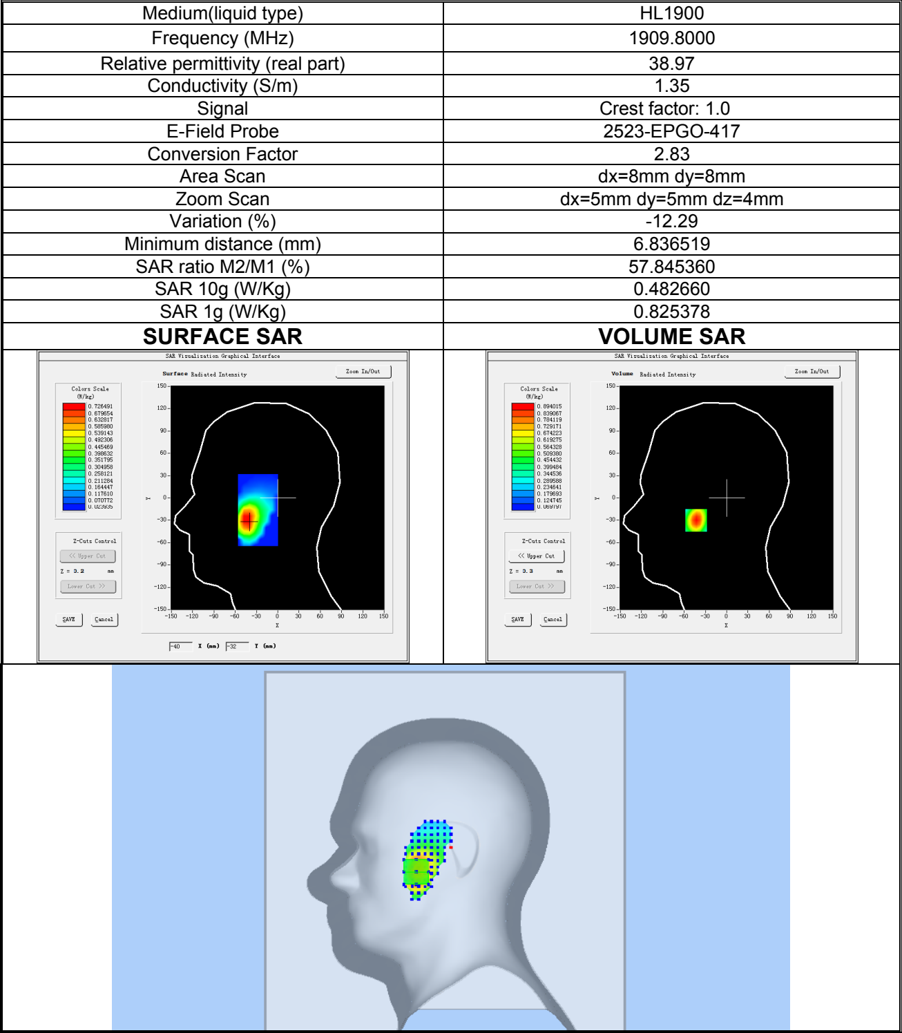
Plot 3: GSM 1900, High channel (Right Head Cheek) Product Description: Smart Phone Test Date: 2026-08-13
