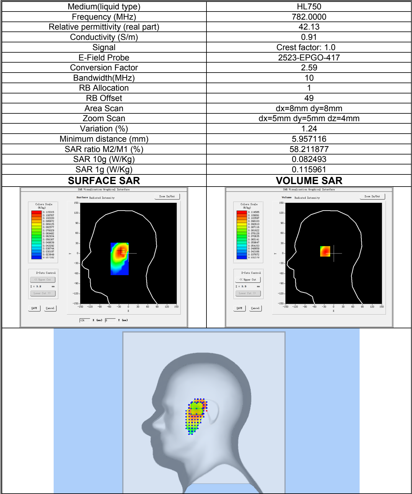
Plot 21:LTE BAND 13, Low channel (Right Head Cheek) Product Description: Smart Phone Test Date: 2026-08-16
