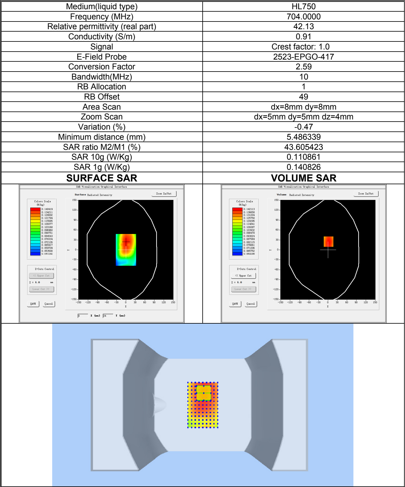
Plot 20: LTE BAND 12, Low channel (Body-worn/ Hotspot, Back Side) Product Description: Smart Phone Test Date: 2026-08-16
