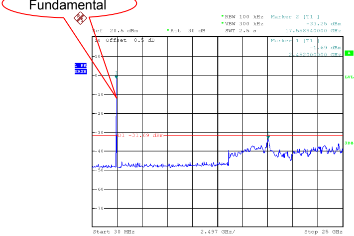
Mode: TX 11 n HT40 channel 9
