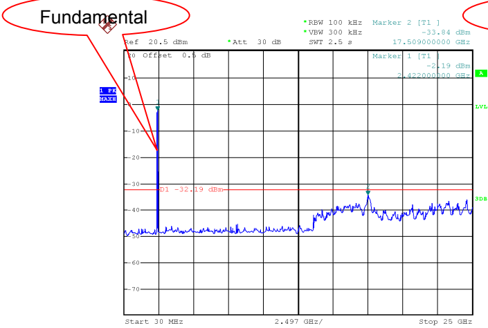
Mode: TX 11n HT40 channel 3
