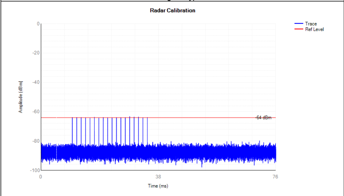
Radar Signal Type 3
