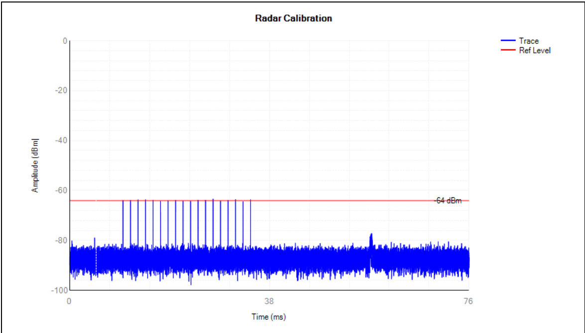
Radar Signal Type 4
