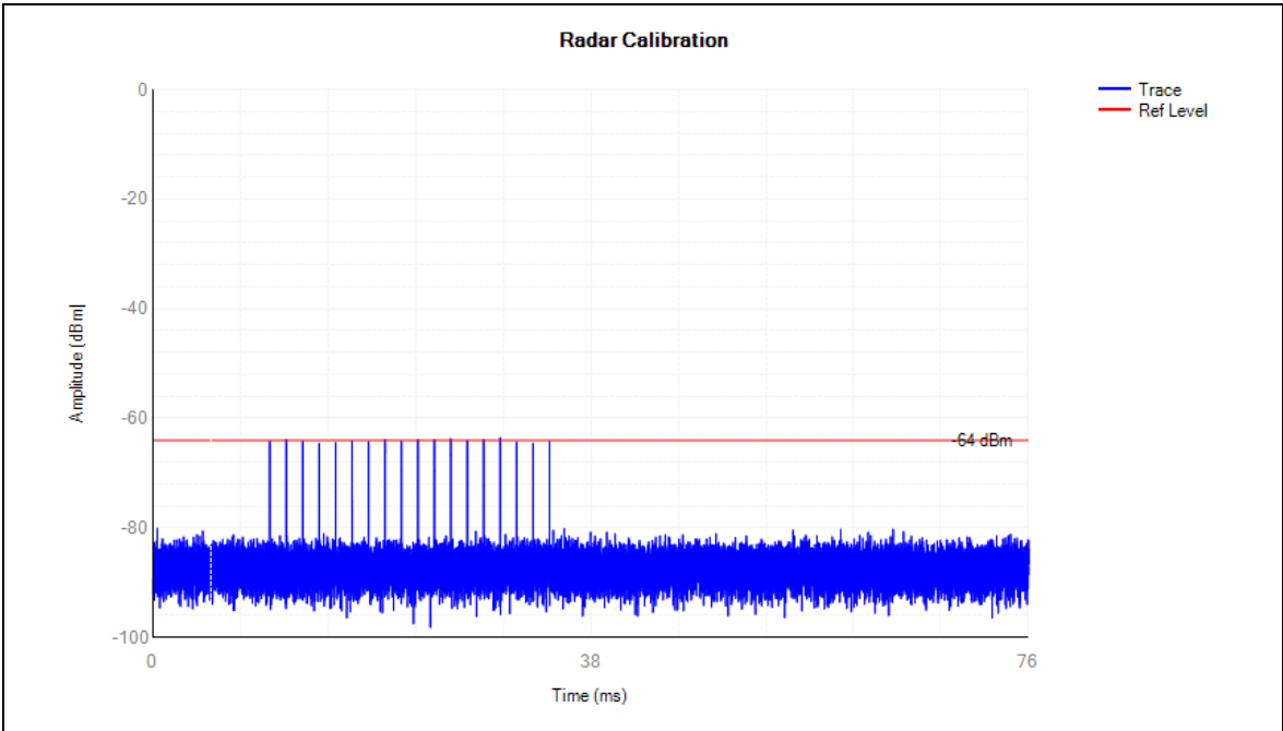
Radar Signal Type 6
