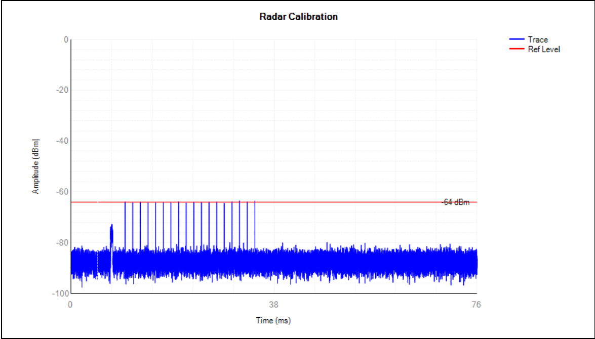
Radar Signal Type 6 AAB B
