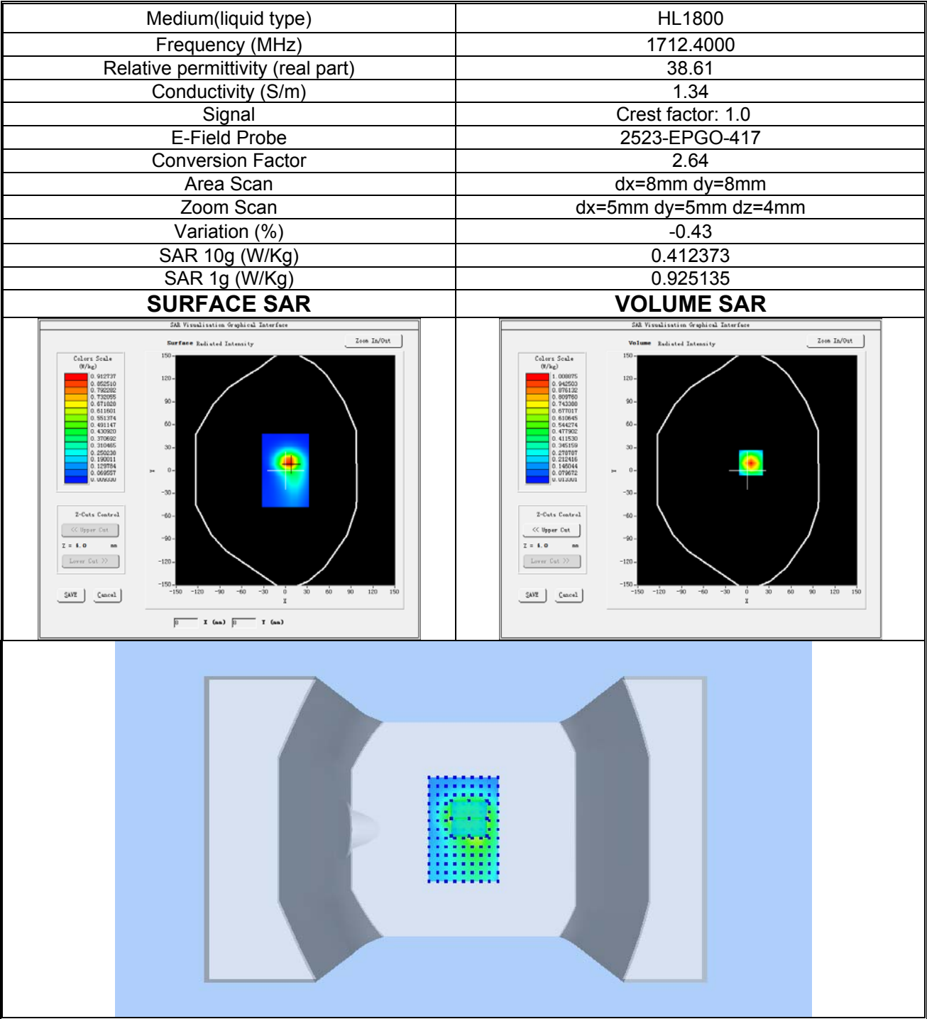
Plot 8: WCDMA BAND IV, Low channel (Body-worn/Hotspot, Bottom Edge) Product Description: Smart Phone Test Date: 2026-01-23
