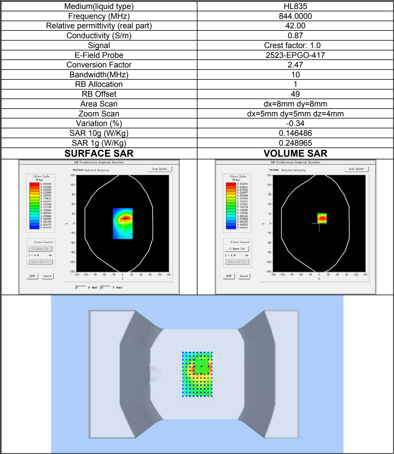
Plot 16: LTE BAND 5, High channel (Body-worn/ Hotspot, Front Side) Product Description: Smart Phone Test Date: 2026-01-25
