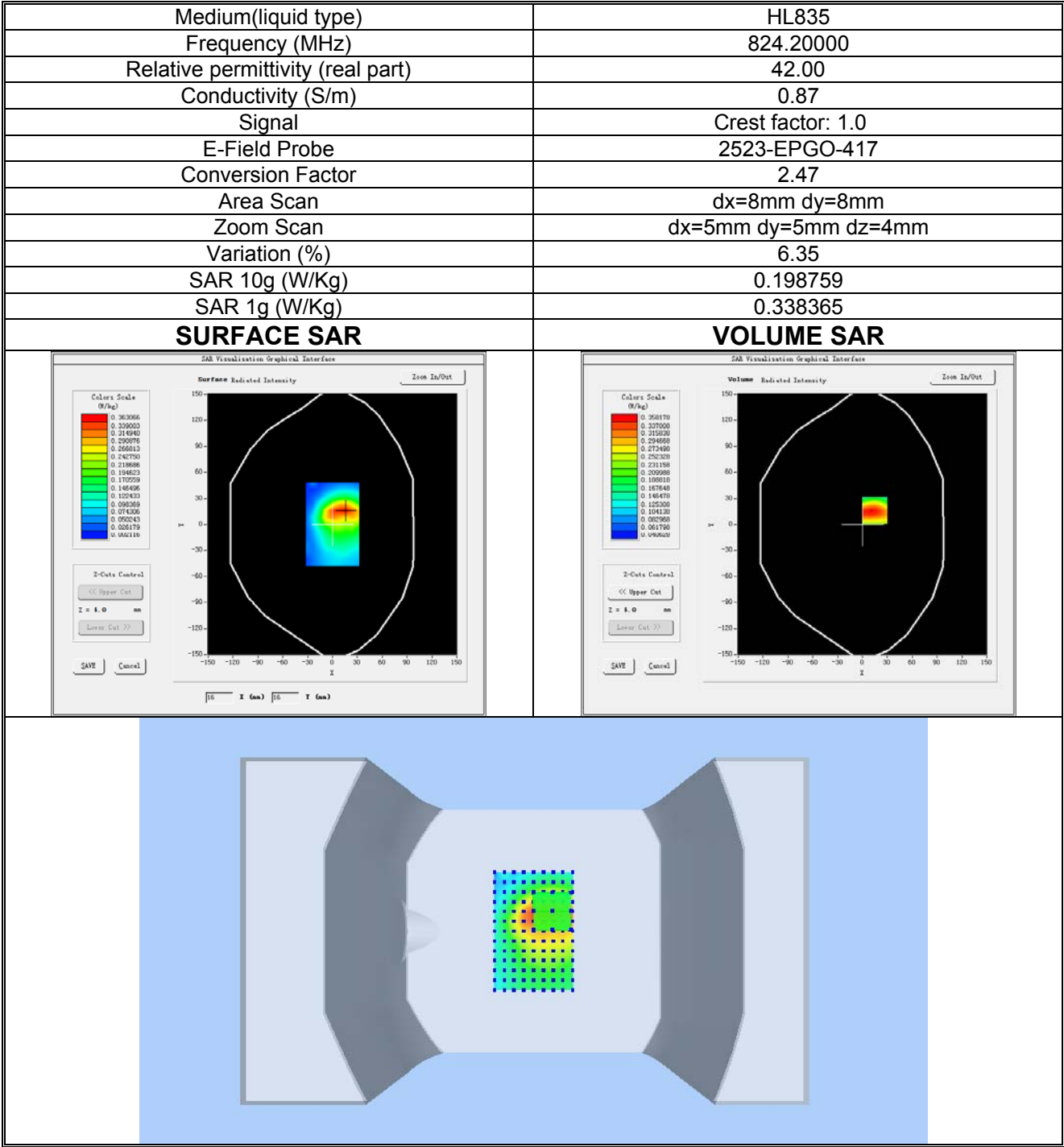
Plot 2: GPRS850, Low channel (Body-worn /Hotspot, Front Side) Product Description:Smart Phone Test Date: 2026-01-25
