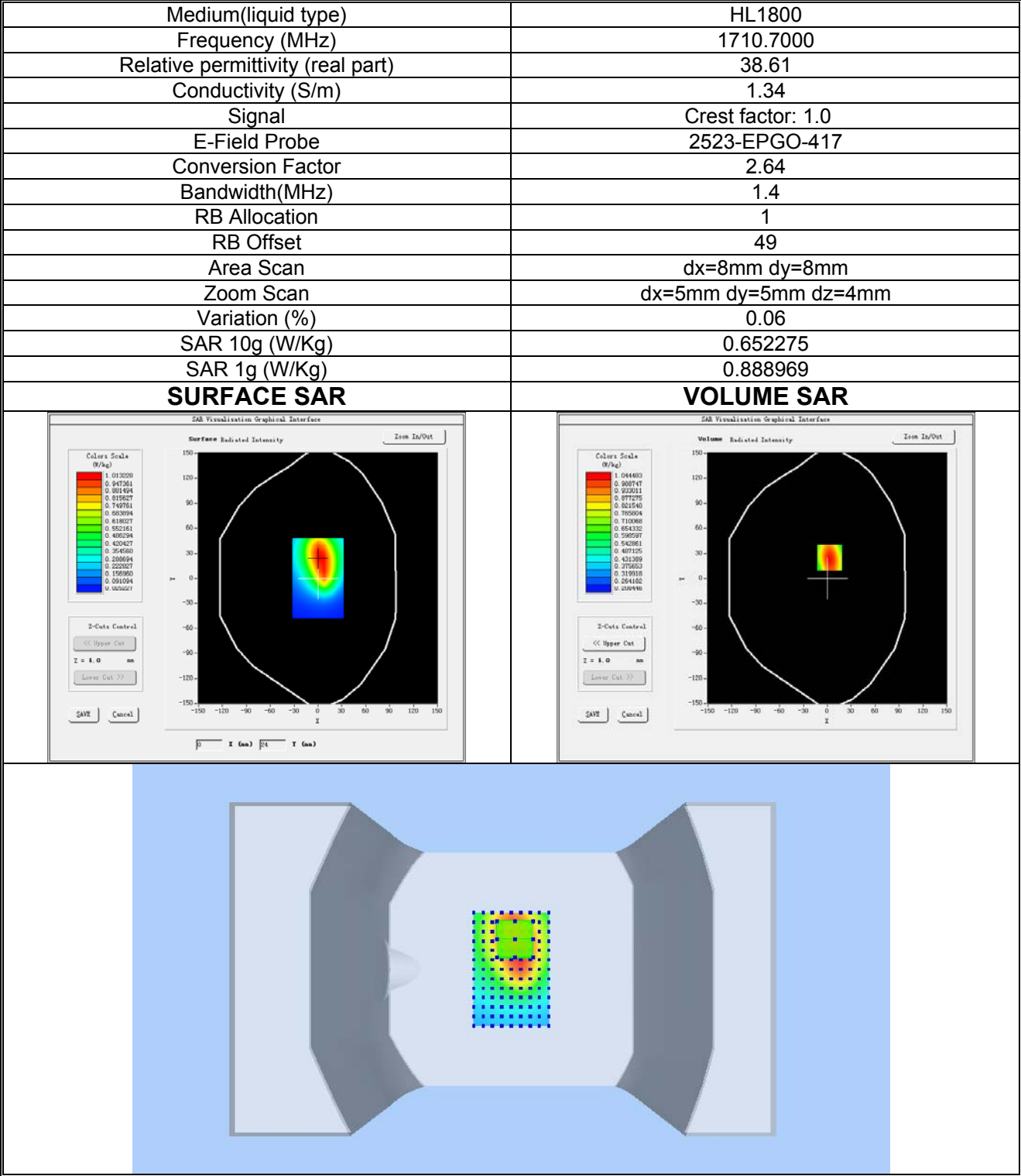
Plot 14: LTE BAND 4, Low channel (Body-worn/ Hotspot, Bottom Edge) Product Description: Smart Phone Test Date: 2026-01-23
