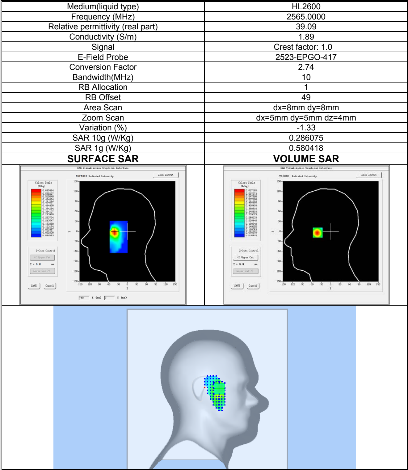
Plot 17:LTE BAND 7, High channel (Left Head Cheek) Product Description: Smart Phone Test Date: 2026-01-22
