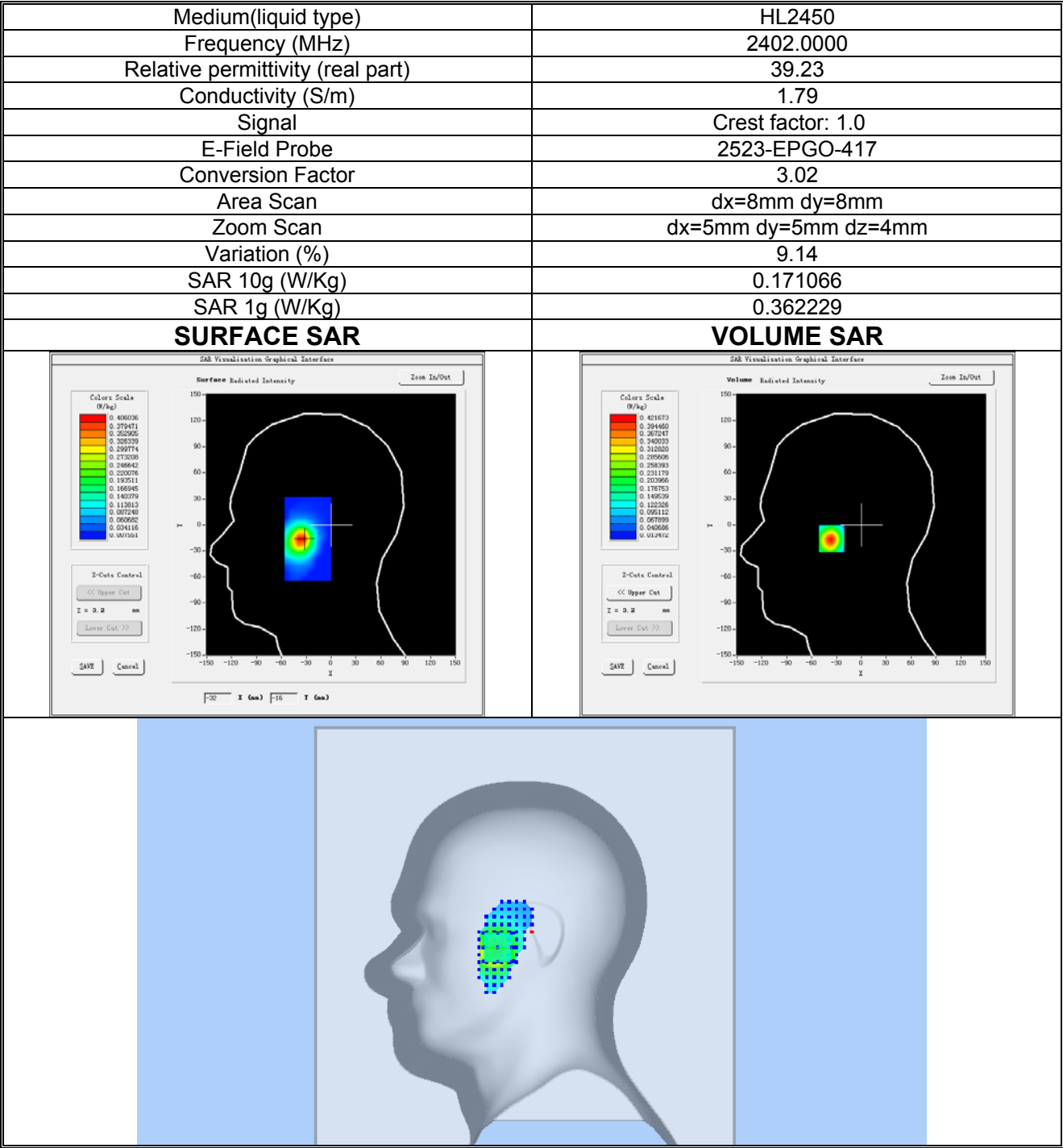
Plot 23: Bluetooth, Low channel (Right Head Cheek) Product Description: Smart Phone Test Date: 2026-01-22
