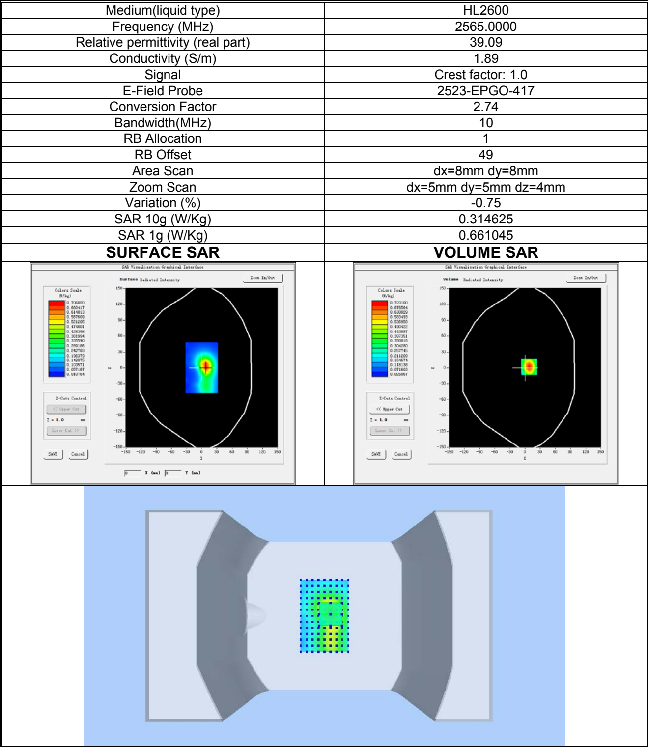
Plot 18: LTE BAND 7, High channel (Body-worn/ Hotspot, Bottom Edge) Product Description: Smart Phone Test Date: 2026-01-22
