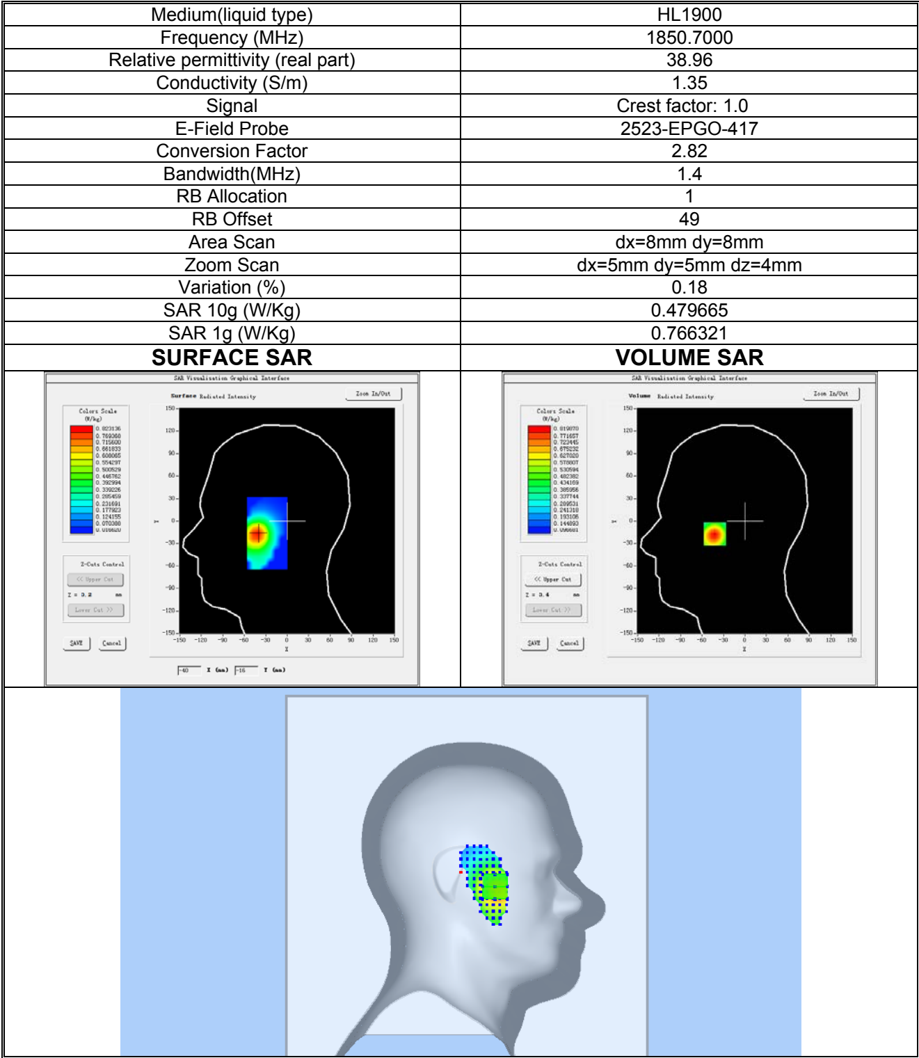
Plot 11:LTE BAND 2, Low channel (Left Head Cheek) Product Description:Smart Phone Test Date: 2026-02-01
