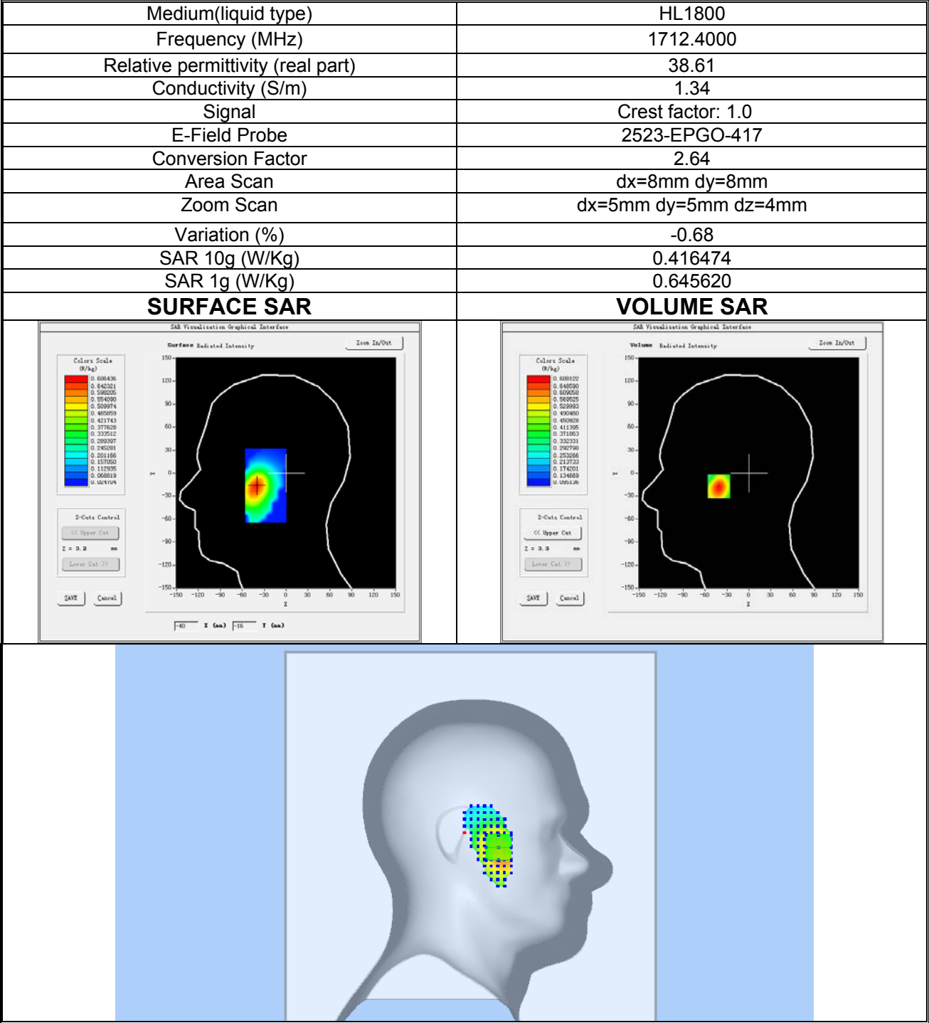
Plot 7: WCDMA BAND IV, Low channel (Left Head Cheek) Product Description: Smart Phone Test Date: 2026-01-23
