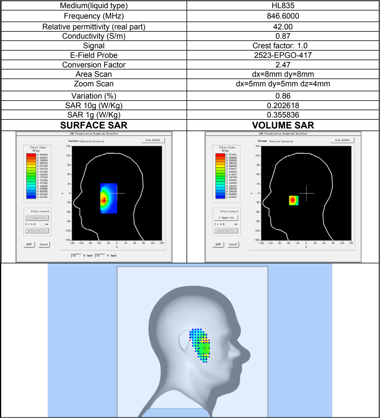
Plot 9: WCDMA BAND V, High channel (Left Head Cheek) Product Description: Smart Phone Test Date: 2026-01-25
