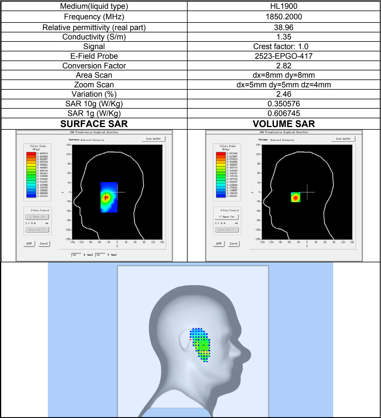
Plot 3: GSM 1900, Low channel (Left Head Cheek) Product Description: Smart Phone Test Date: 2026-02-01
