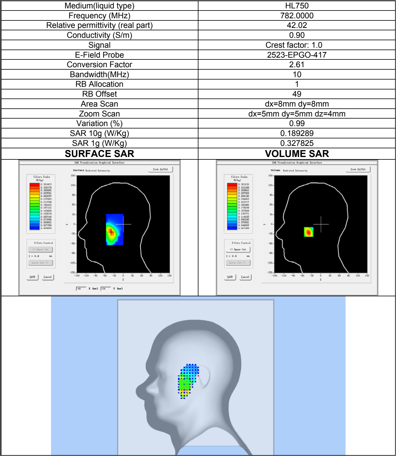
Plot 19:LTE BAND 13, Low channel (Right Head Cheek) Product Description: Smart Phone Test Date: 2026-01-25
