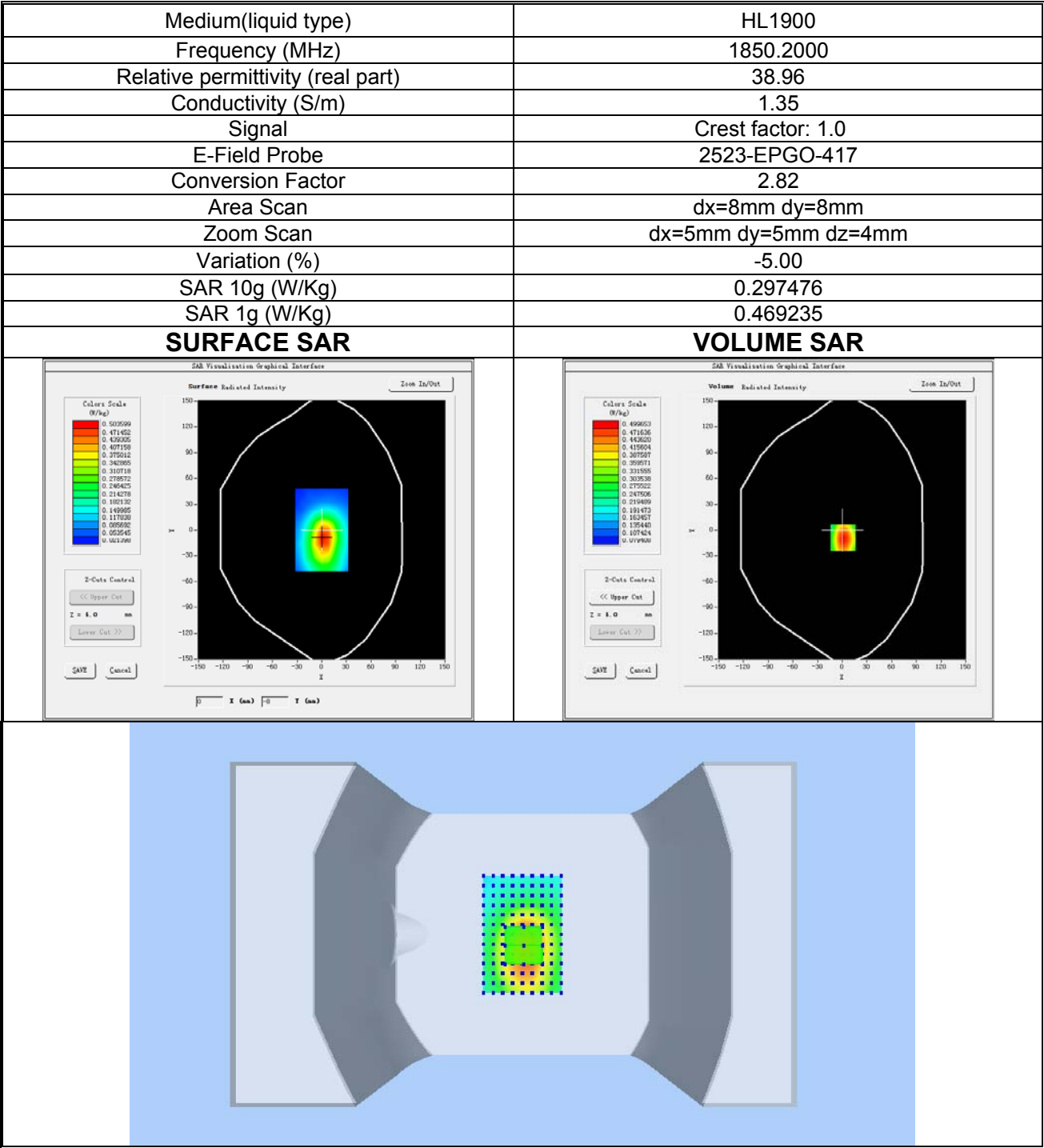
Plot 4: GSM 1900, Low channel (Body-worn /Hotspot, Bottom Edge) Product Description: Smart Phone Test Date: 2026-02-01
