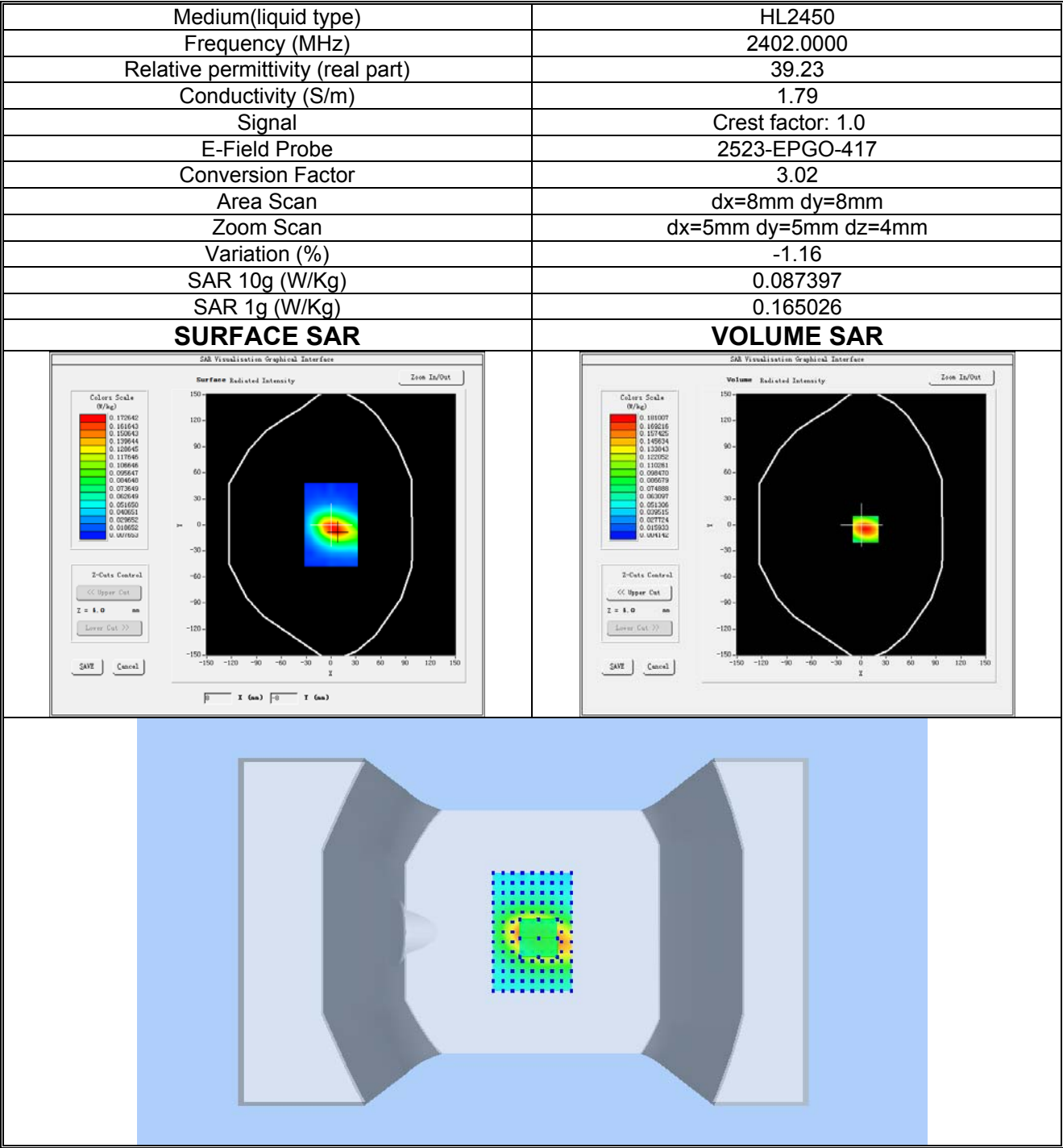
Plot 24: Bluetooth, Low channel (Body-worn/ Hotspot, Back Side) Product Description: Smart Phone Test Date: 2026-01-22
