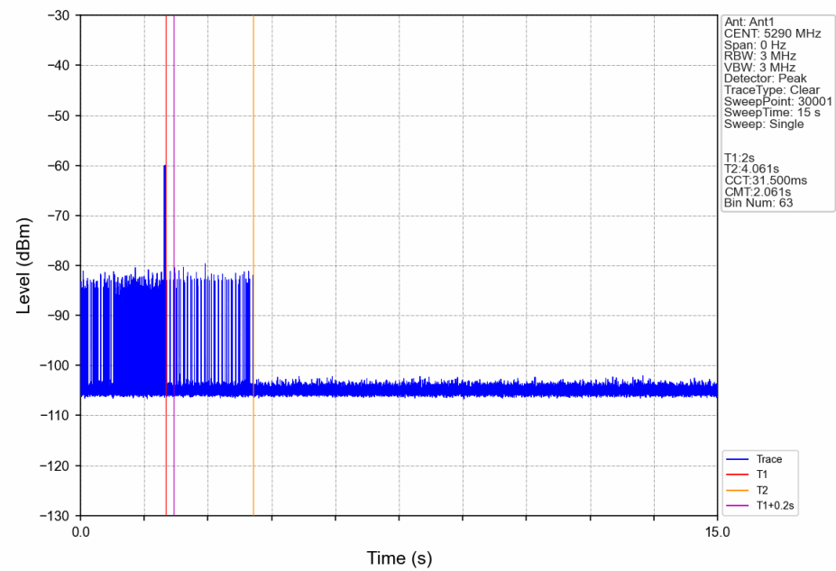
802.11ac80 channel 58 5290MHz
