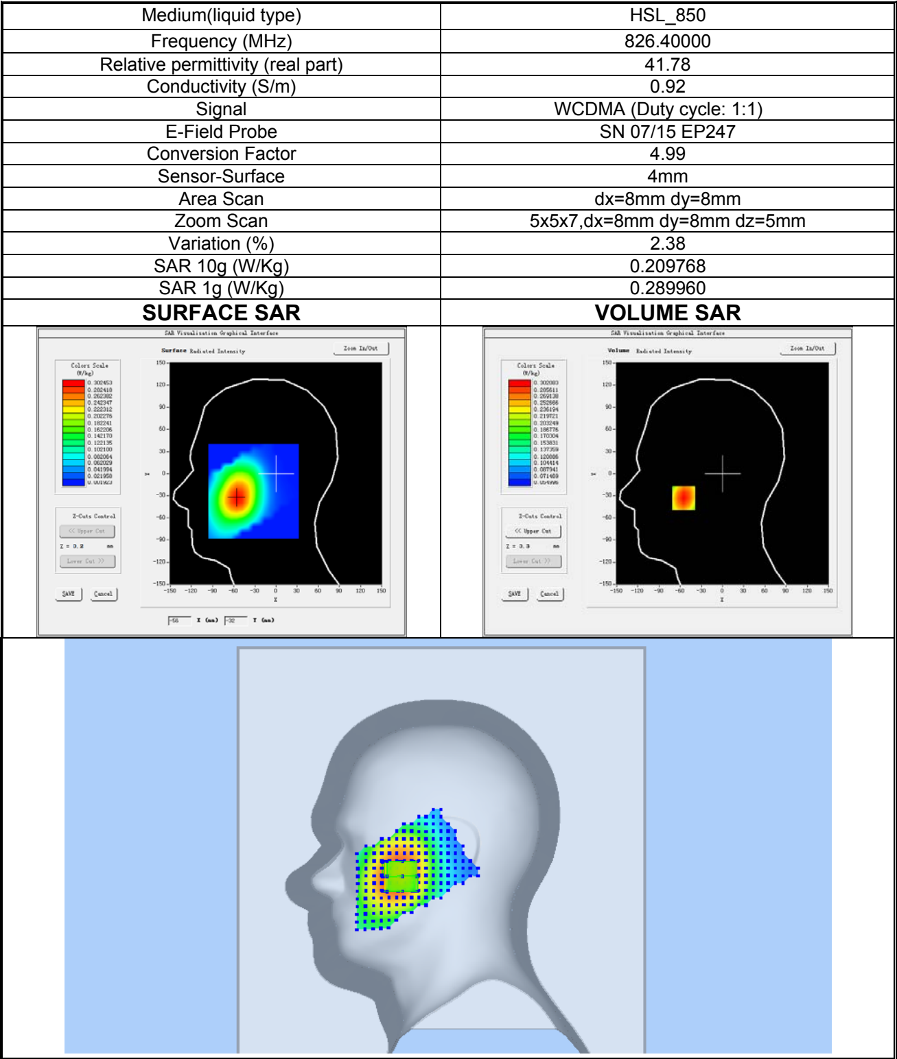
Plot 5: WCDMA BAND V, Low channel (Right Head Cheek) Product Description: SMARTPHONE Test Date: 2021-03-02
