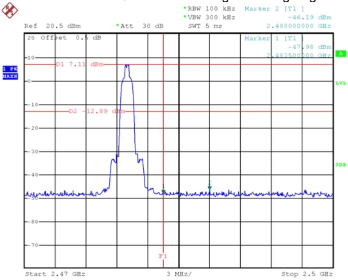
Pi/4 DQPSK Transmitting Band edge-right side
