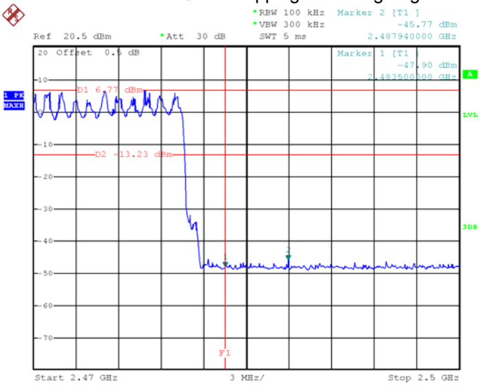
Pi/4 DQPSK Hopping Band edge-right side
