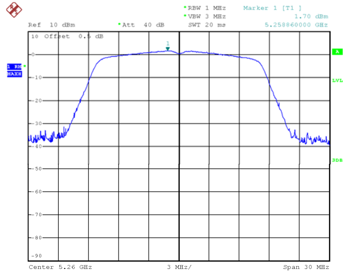
802.11a U-NII-2A Low channel
