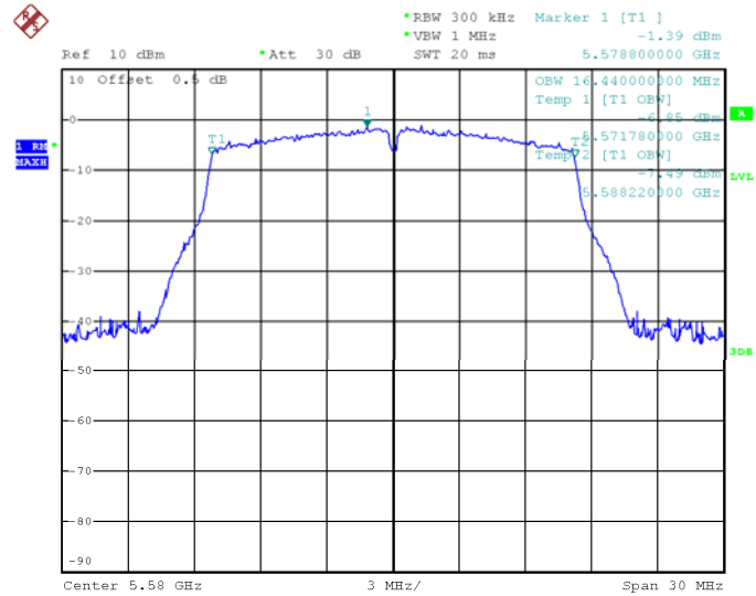
802.11a U-NII-2C Middle channel
