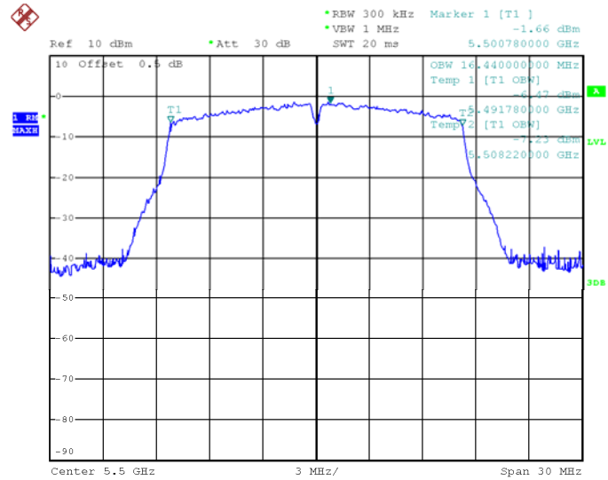
802.11a U-NII-2C Low channel
