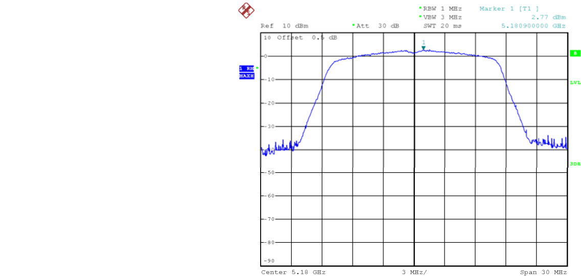
802.11a U-NII-1 Low channel
