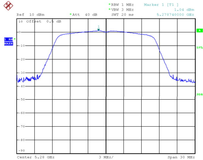
802.11a U-NII-2A Middle channel
