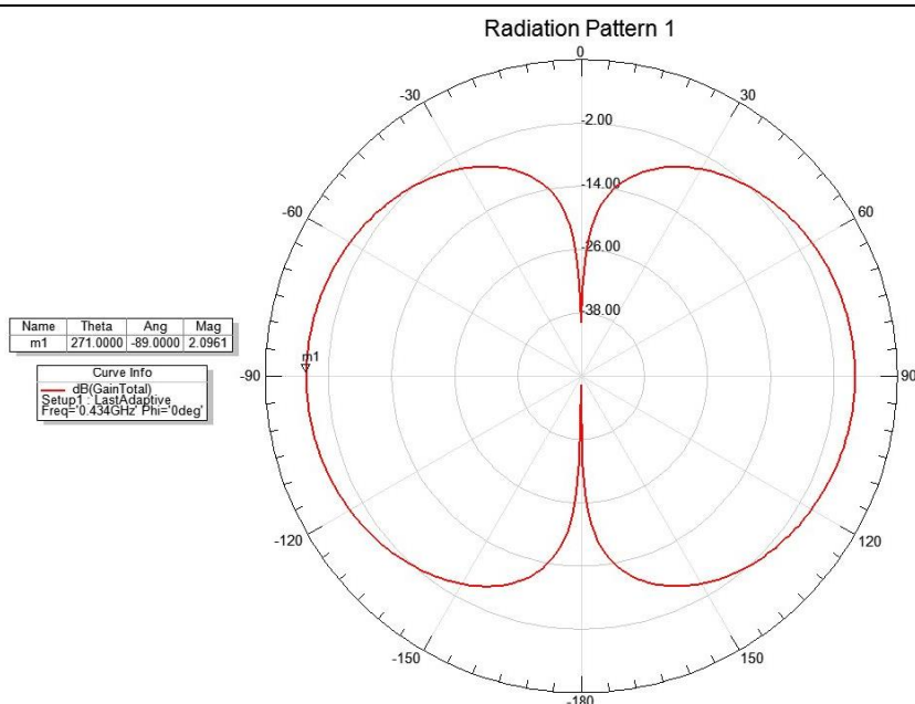
Figure2: Radiation Pattern for XZ-Plane, Horizontal Polarization
