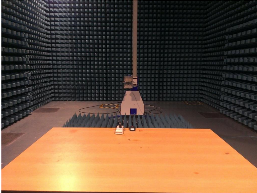
Photograph 3: Radiated Emission Test Configuration, (Above 1GHz) Front
