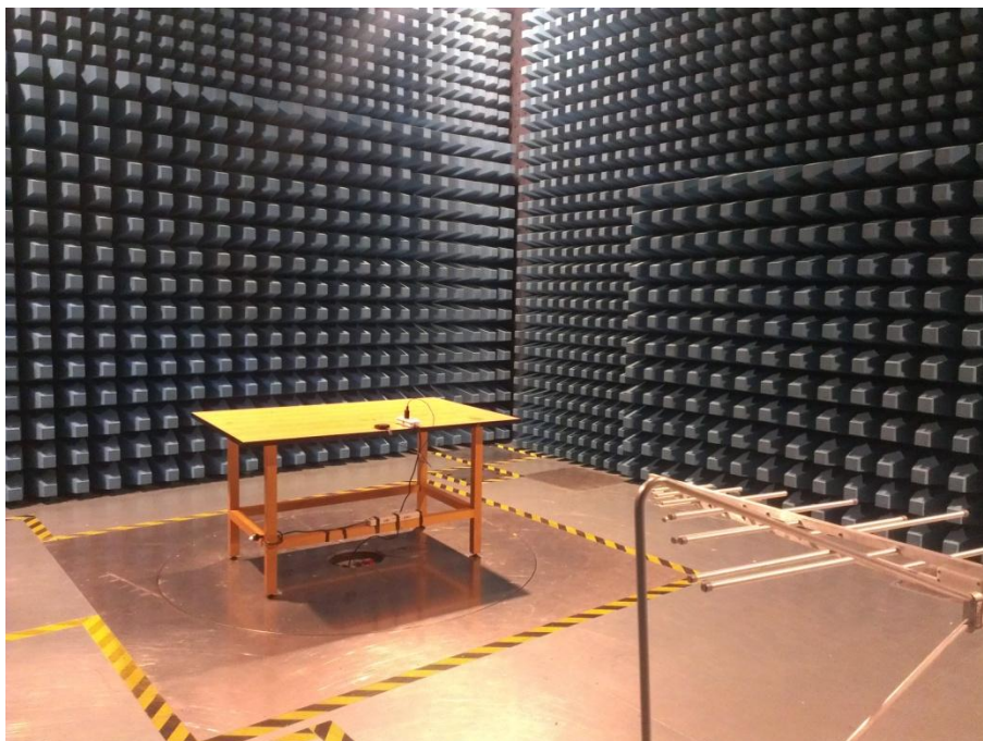
Photograph 2: Radiated Emission Test Configuration, (Below 1GHz) Back
