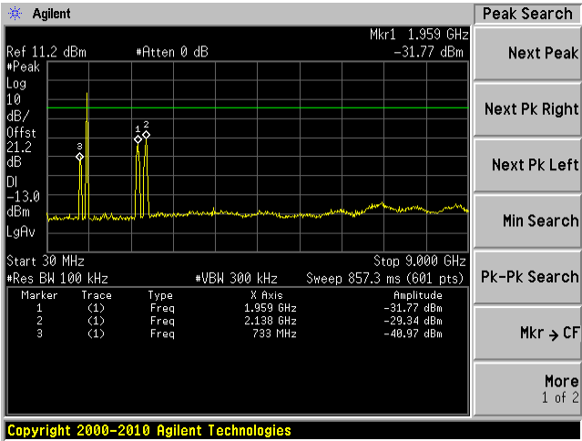
DL Middle 30MHz-9GHz
