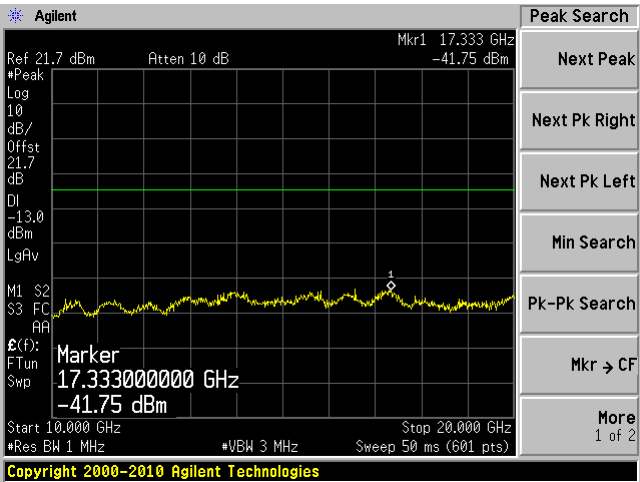
High 10GHz-20GHz
