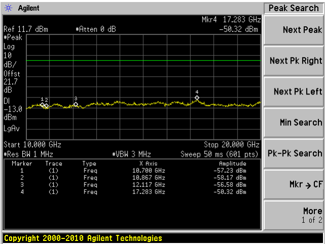
High 10GHz-20GHz
