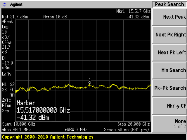
Middle 10GHz-20GHz
