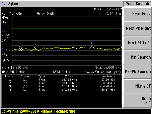
Low 10GHz-20GHz
