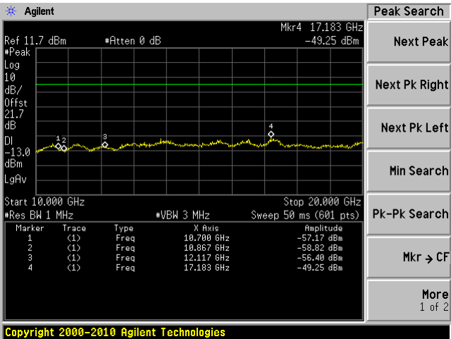
High 10GHz-20GHz
