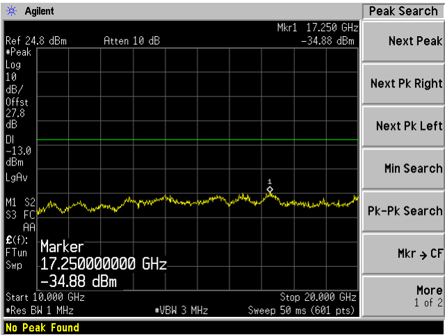
Low 10GHz-20GHz
