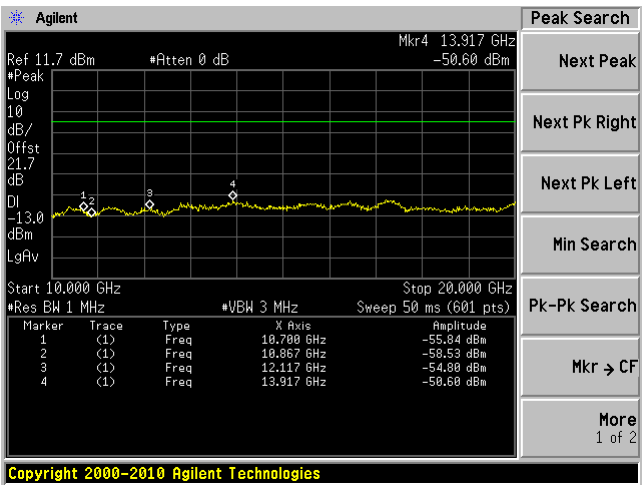
Middle 10GHz-20GHz
