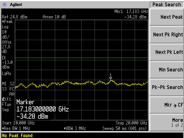
High 10GHz-20G
