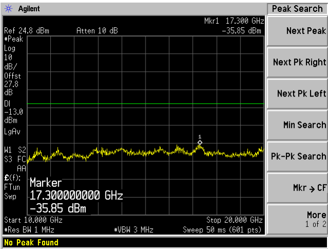
Middle 10GHz-20GHz
