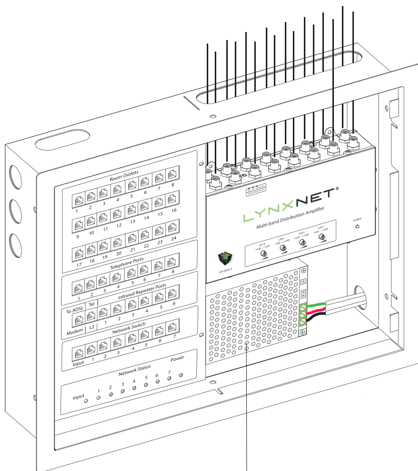
18V power supply
