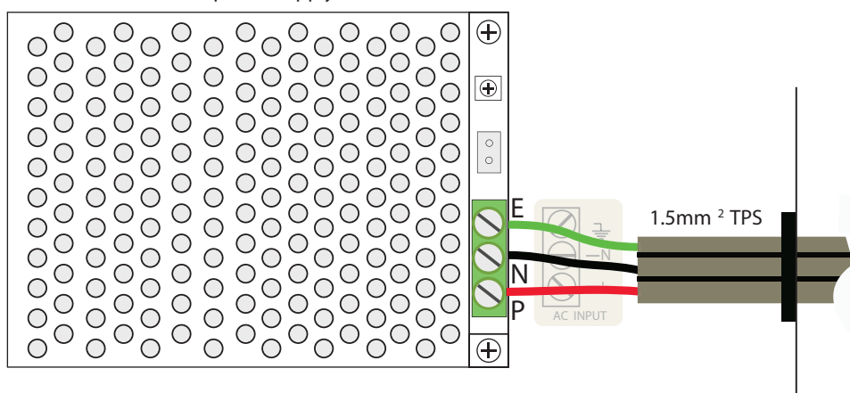
18V power supply
