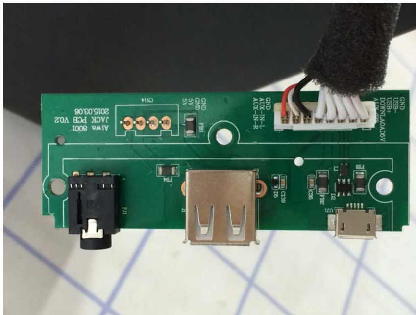
PCB 5 side 2 view
