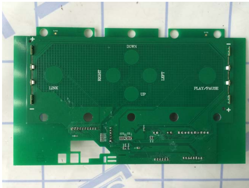
PCB 6 side 2 view
