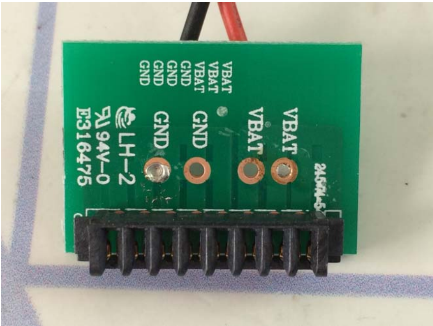
PCB 9 side 2 view
