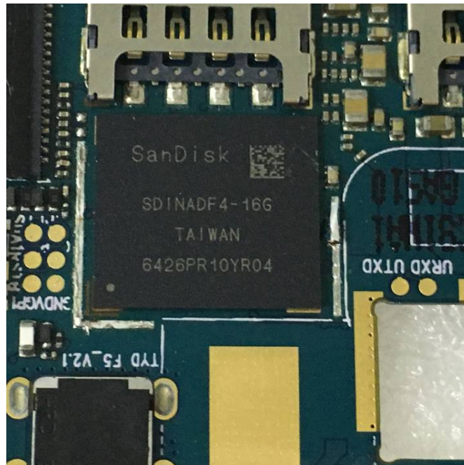
EUT – Main IC View 1
