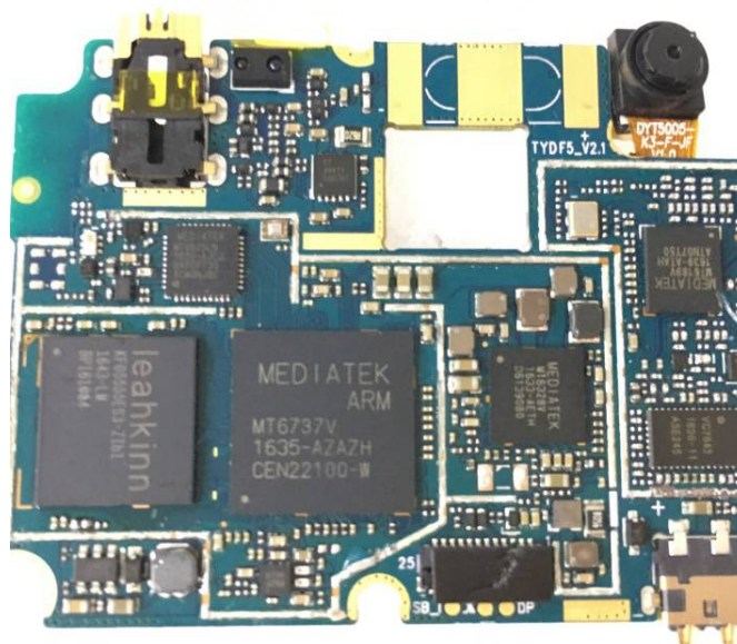
EUT – Main IC View 2
