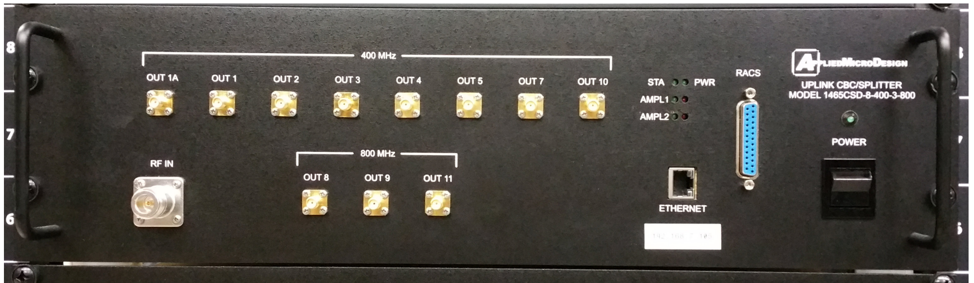
CBC Splitter - Front Panel
