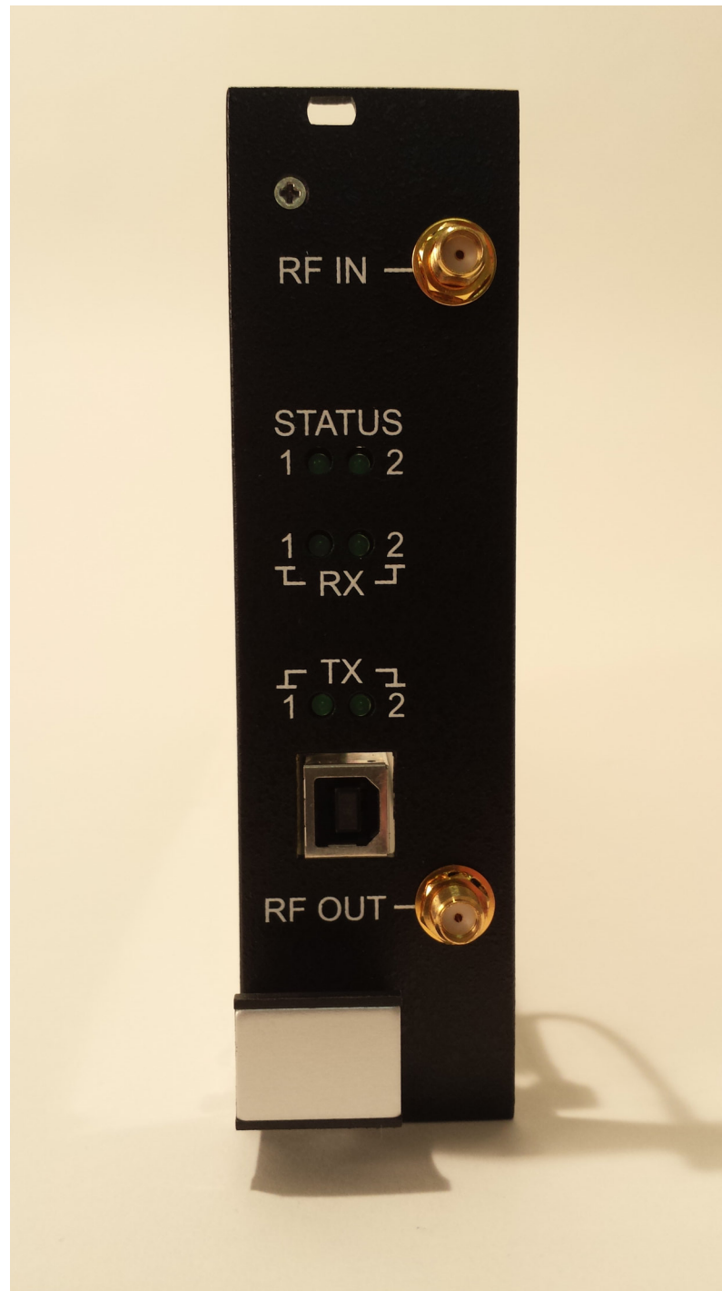
DSP Card - Front Panel
