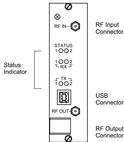
DSP Card
