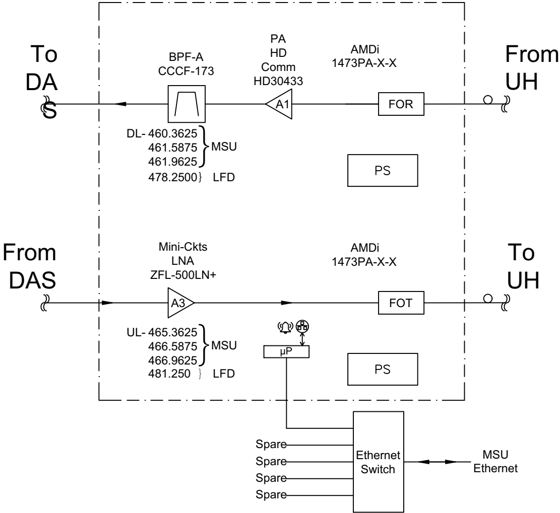
Typical Remote
