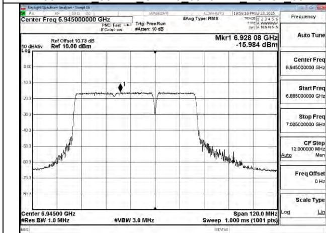
802.11be 80MHz Chain0 6945MHz 484+242 MRU4
