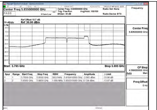
802.11n 40MHz Chain0 5835MHz UNII 3
