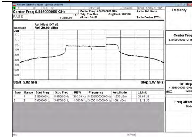
802.11n 20MHz Chain0 5845MHz UNII 3
