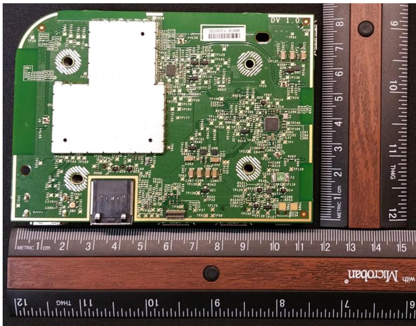
Motherboard Bottom
