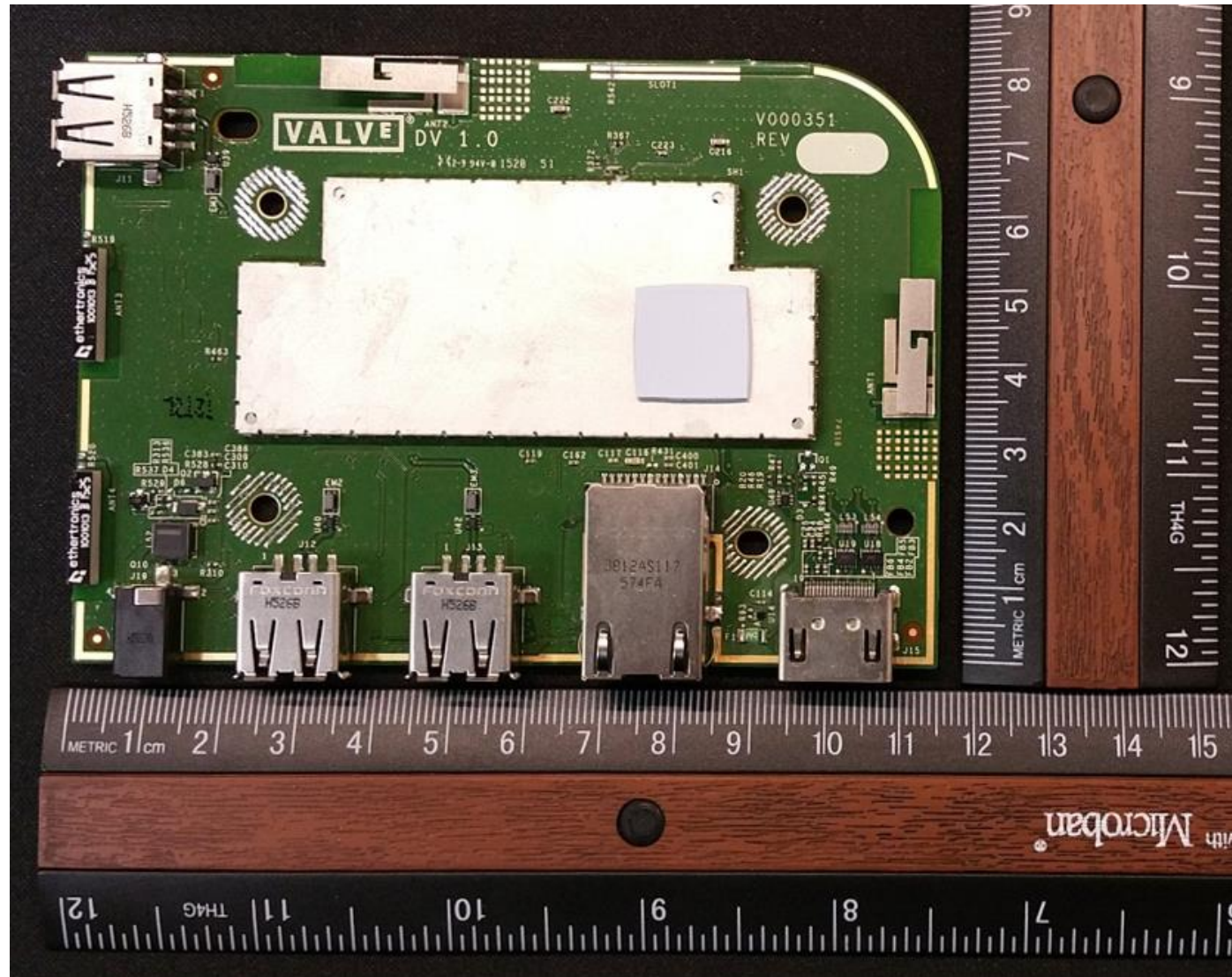
Motherboard Top
