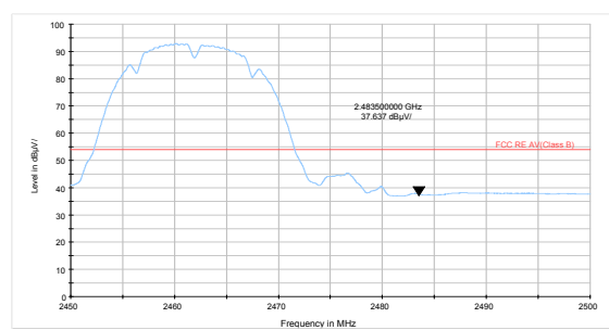
802.11b-Channel 11 Average
