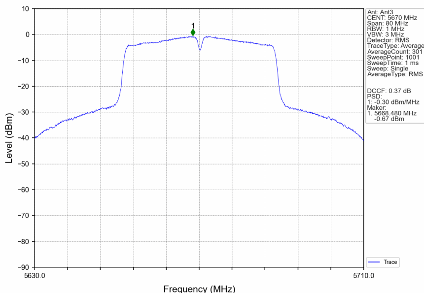
802.11n(HT40)_HCH_5670MHz_Ant3_NTNV
