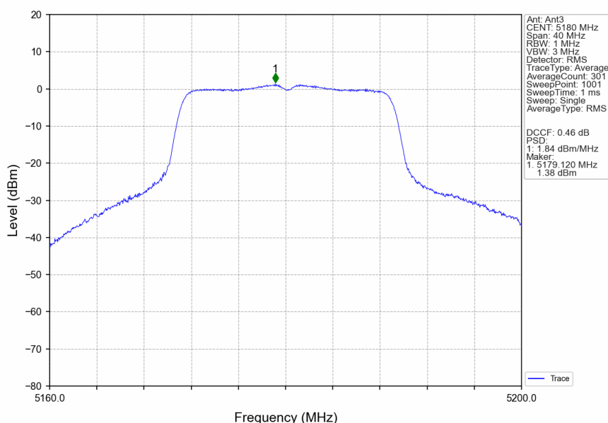
802.11ac(VHT20)_LCH_5180MHz_Ant3_NTNV
