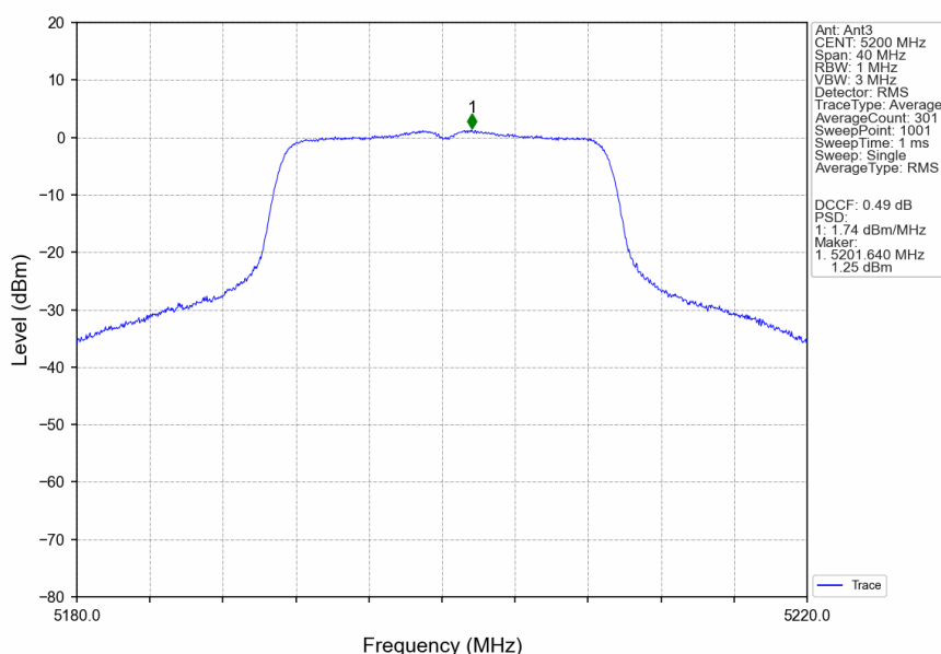
802.11ac(VHT20)_MCH_5200MHz_Ant3_NTNV
