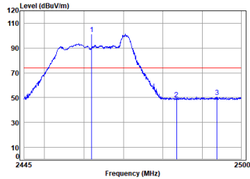
11ax_20M_Partial_RU26_TX_CH_11_Horizontal-Peak
