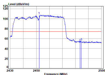
11ax_40M_Partial_RU242_TX_CH_09_Vertical-Peak
