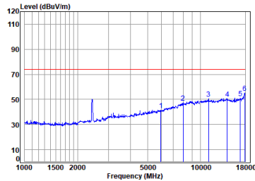
11ax_40M_TX_CH_03_Vertical-Peak
