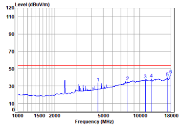
11ax_40M_TX_CH_03_Vertical-Avg
