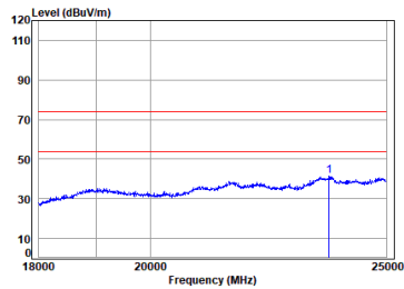
11ax_40M_TX_CH_09_Horizontal
