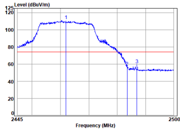
11ax_20M_TX_CH_11_Vertical-Peak
