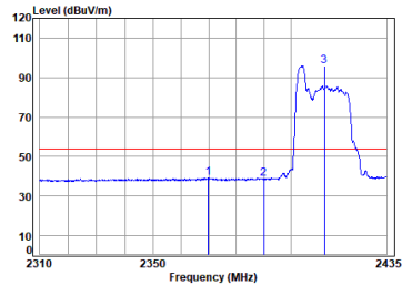
11ax_20M_Partial_RU26_TX_CH_01_Vertical-Avg
