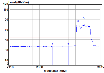
11ax_20M_Partial_RU26_TX_CH_01_Horizontal-Avg
