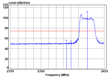
11ax_20M_Partial_RU26_TX_CH_01_Vertical-Peak
