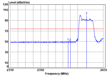
11ax_20M_Partial_RU26_TX_CH_01_Horizontal-Peak
