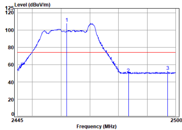
11ax_20M_Partial_RU26_TX_CH_11_Vertical-Peak
