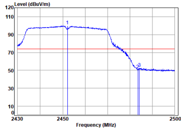
11n_HT(40M)_TX_CH_09_Horizontal-Peak
