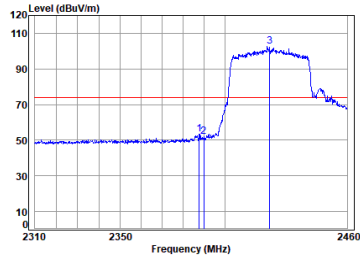
11ax_40M_TX_CH_03_Horizontal-Peak
