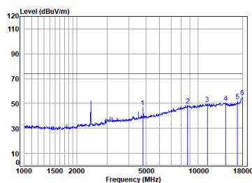
11b_TX_CH_01_Horizontal-Peak
