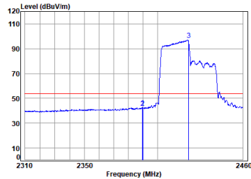
11ax_40M_Partial_RU242_TX_CH_03_Vertical-Avg
