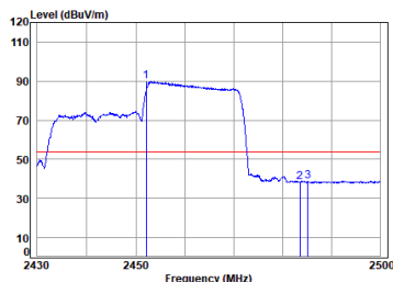
11ax_40M_Partial_RU242_TX_CH_09_Horizontal-Avg
