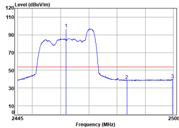
11ax_20M_Partial_RU26_TX_CH_11_Vertical-Avg
