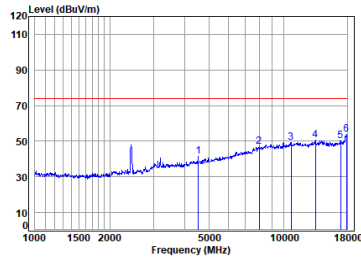
11n_HT(40M)_TX_CH_06_Vertical-Peak
