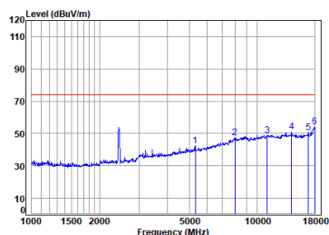
11ax_40M_TX_CH_06_Horizontal-Peak
