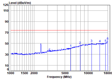
11n_HT(40M)_TX_CH_09_Vertical-Peak
