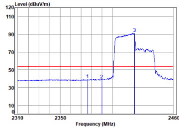
11ax_40M_Partial_RU242_TX_CH_03_Horizontal-Avg
