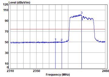
11ax_40M_Partial_RU242_TX_CH_03_Horizontal-Peak
