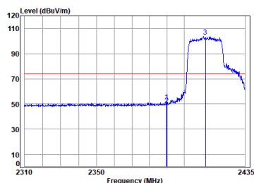
11ax_20M_TX_CH_01_Horizontal-Peak
