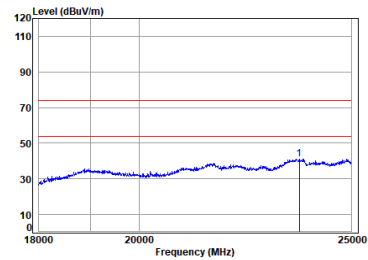
11ax_40M_TX_CH_09_Vertical
