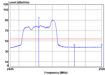
11ax_20M_Partial_RU26_TX_CH_11_Horizontal-Avg
