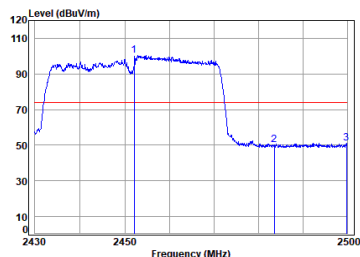
11ax_40M_Partial_RU242_TX_CH_09_Horizontal-Peak
