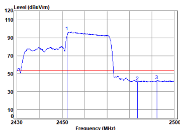
11ax_40M_Partial_RU242_TX_CH_09_Vertical-Avg
