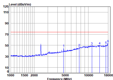
11ax_40M_TX_CH_06_Vertical-Peak
