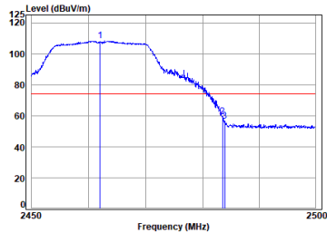
11n_HT(20M)_TX_CH_11_Vertical-Peak
