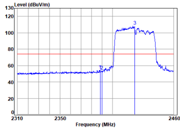
11ax_40M_Partial_RU242_TX_CH_03_Vertical-Peak
