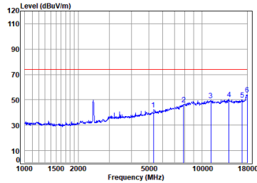
11n_HT(40M)_TX_CH_06_Horizontal-Peak
