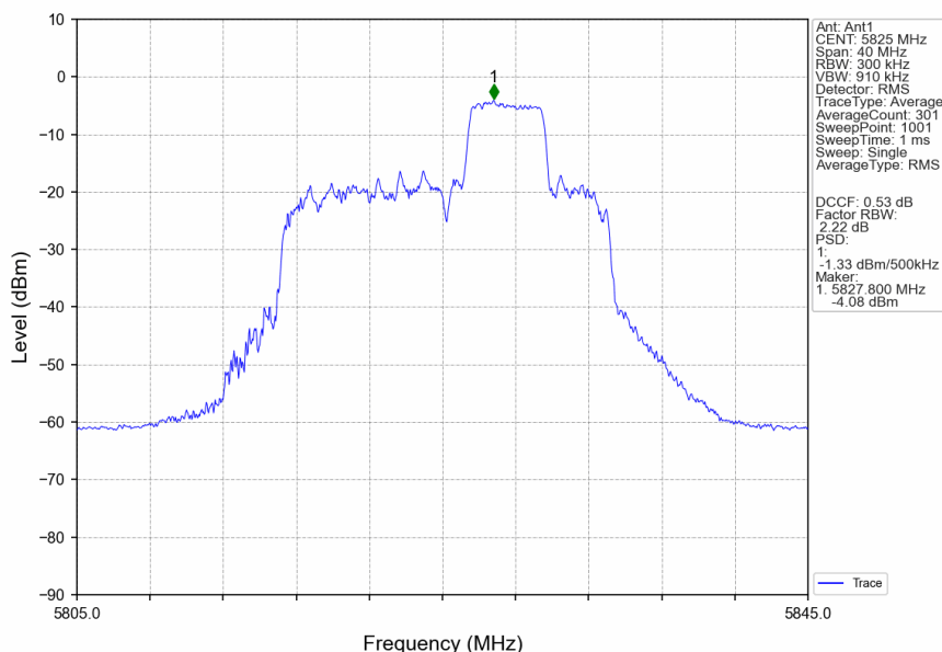
802.11ax(HEW20)_HCH_5825MHz_RU52_Right_Ant1_NTNV
