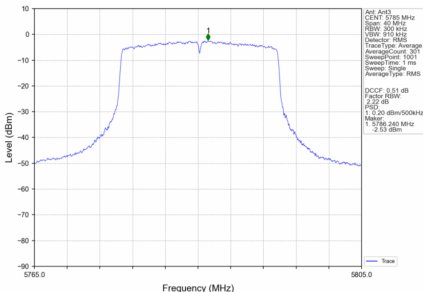
802.11ax(HEW20)_MCH_5785MHz_RU242_Left_Ant3_NTNV
