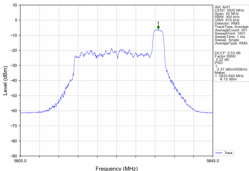
802.11ax(HEW20)_HCH_5825MHz_RU26_Right_Ant1_NTNV
