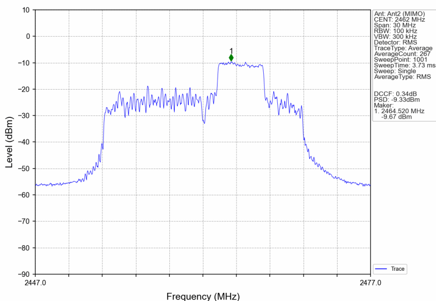
802.11ax(HEW20) HCH 2462MHz RU52 Right MIMO NTN
