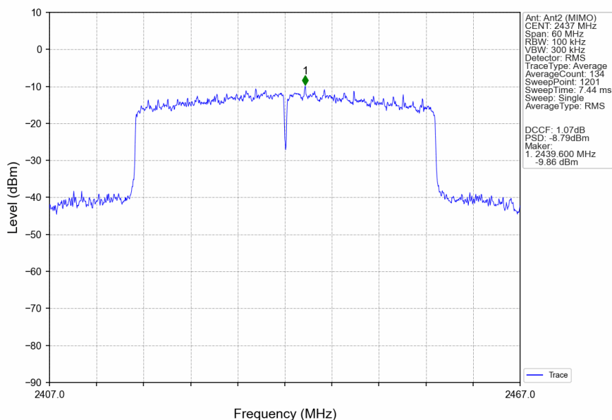
802.11ax(HEW40) MCH 2437MHz RU484 Left MIMO NTN
