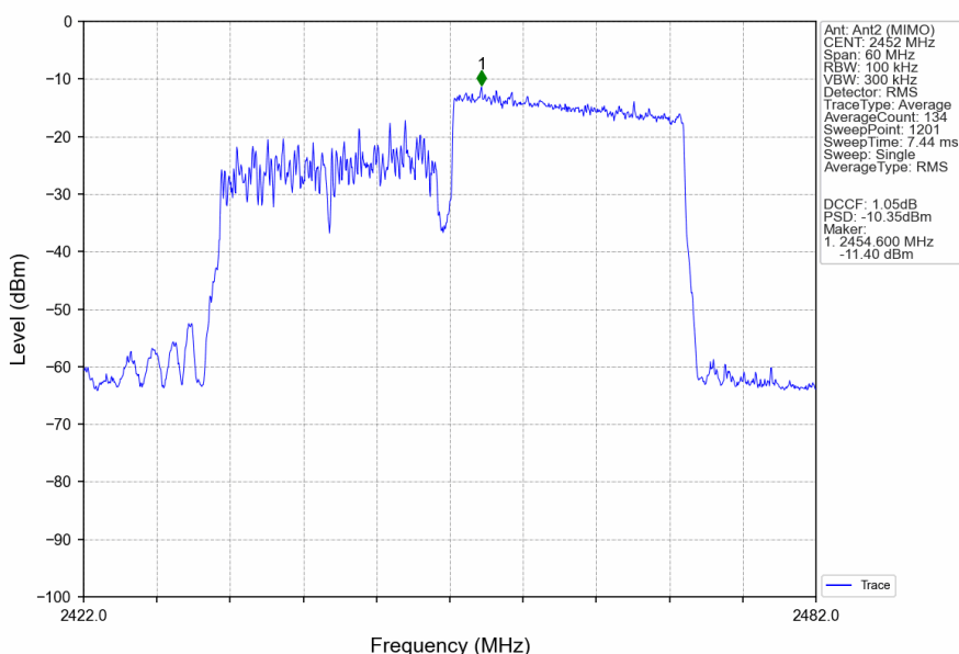
802.11ax(HEW40) HCH 2452MHz RU242 Right Ant2 (MIMO) NTN
