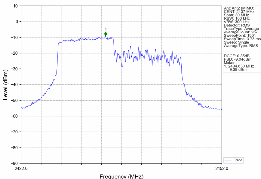
802.11ax(HEW20) MCH 2437MHz RU106 Left Ant2 (MIMO) NTNV
