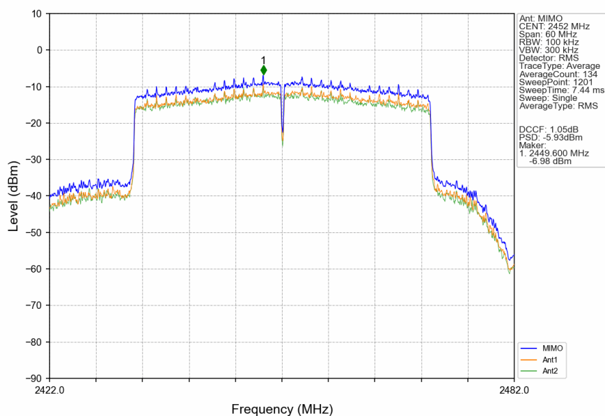
802.11ax(HEW40) HCH 2452MHz RU484 Left MIMO NTN
