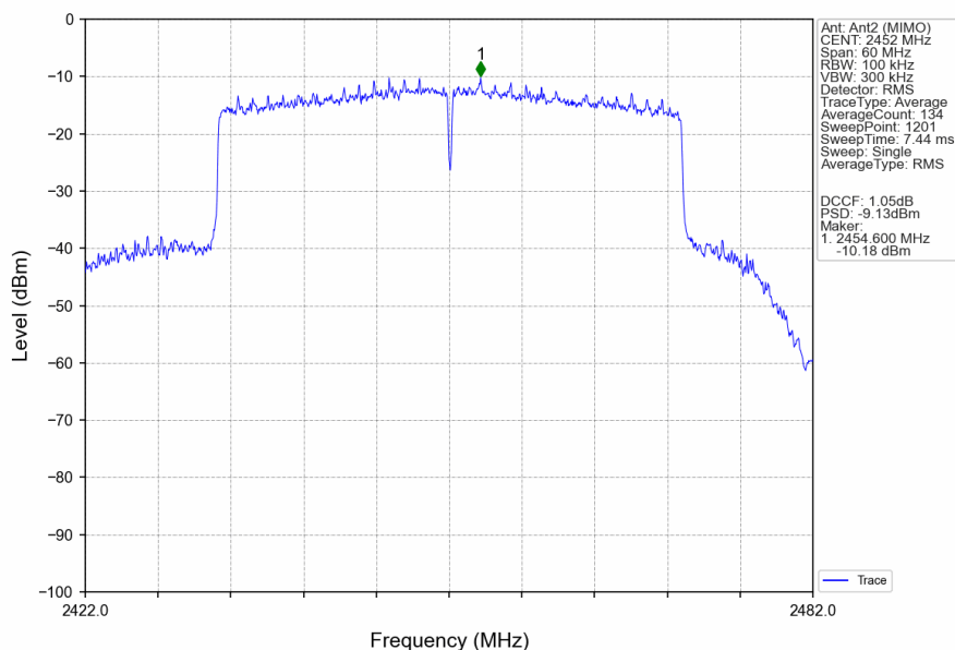
802.11ax(HEW40) HCH 2452MHz RU484 Left MIMO NTN
