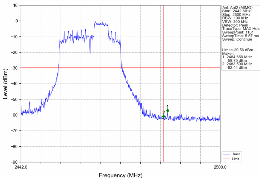
802.11ax(HEW20) HCH 2462MHz RU52 Right Ant2 (MIMO) NTNV
