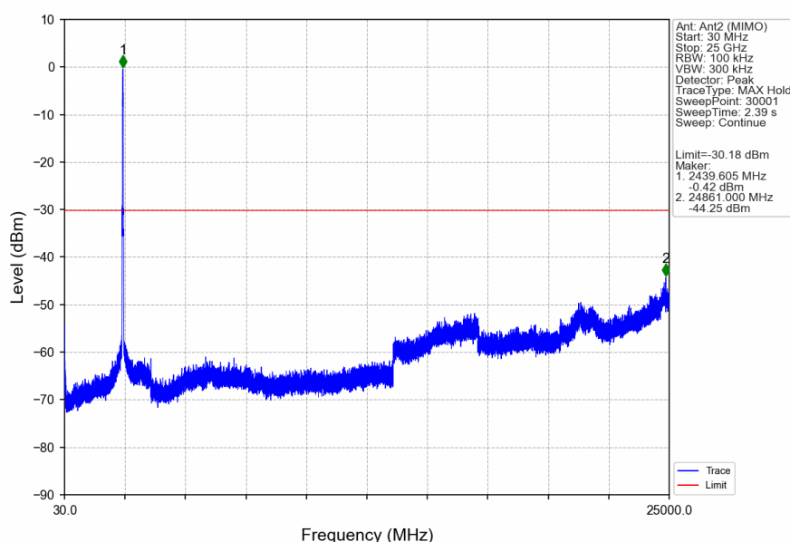
802.11ax(HEW40) MCH 2437MHz RU484 Left Ant2 (MIMO) NTV
