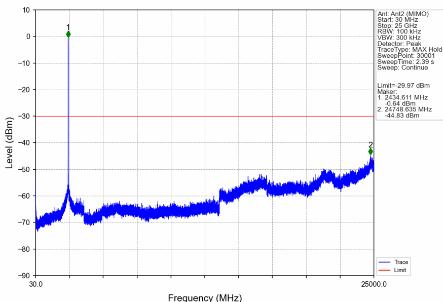
802.11ax(HEW20) MCH 2437MHz RU106 Left Ant2 (MIMO) NTV
