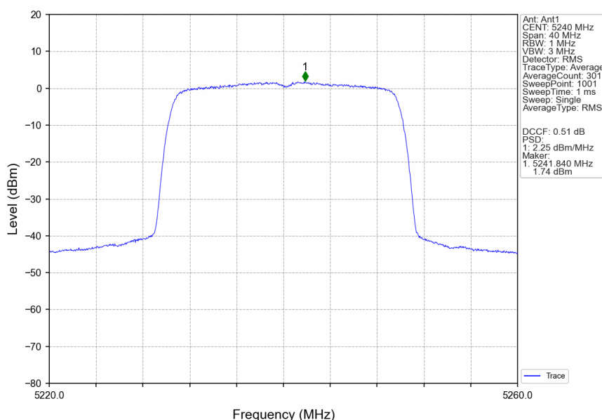
802.11ax(HEW20)_HCH_5240MHz_RU242_Left_Ant1_NTNV
