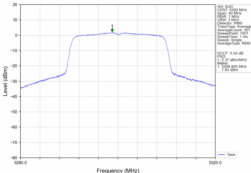
802.11ax(HEW20)_MCH_5300MHz_RU242_Left_Ant3_NTNV
