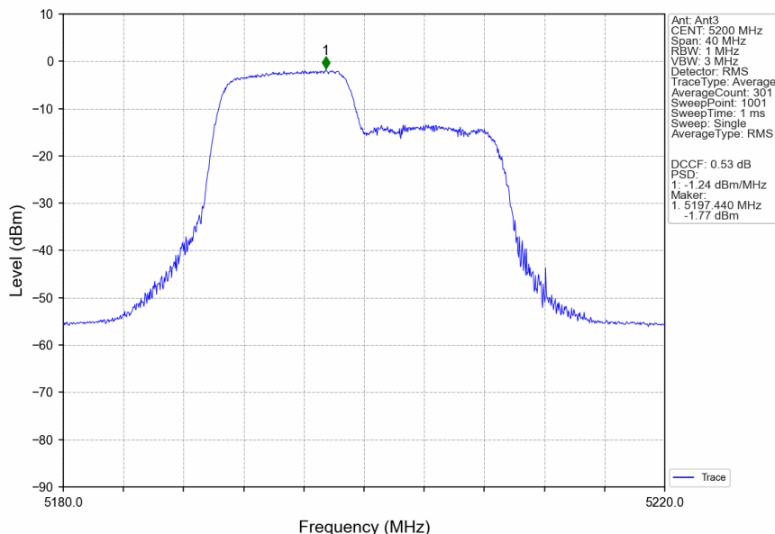
802.11ax(HEW20)_MCH_5200MHz_RU106_Left_Ant3_NTNV
