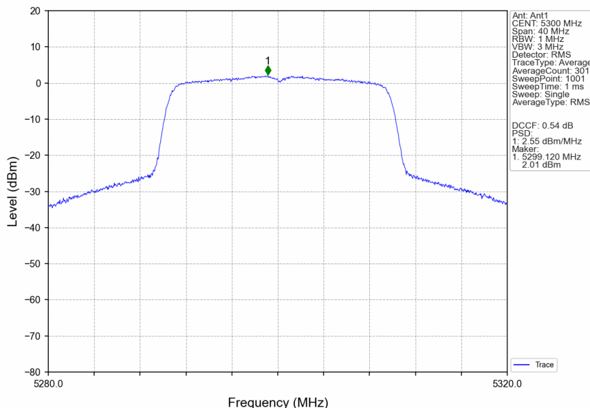
802.11ax(HEW20)_MCH_5300MHz_RU242_Left_Ant1_NTNV
