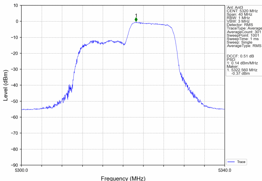
802.11ax(HEW20)_HCH_5320MHz_RU106_Right_Ant3_NTNV
