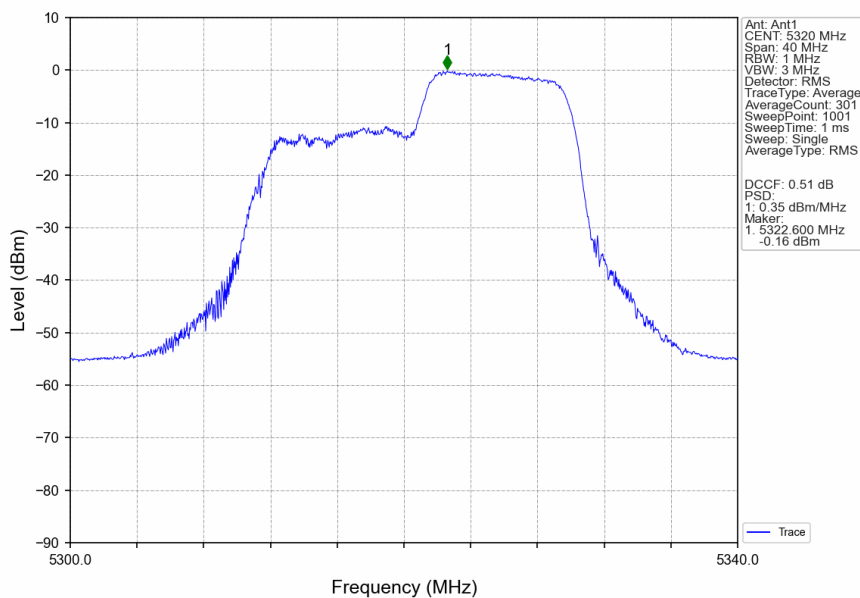
802.11ax(HEW20)_HCH_5320MHz_RU106_Right_Ant1_NTNV
