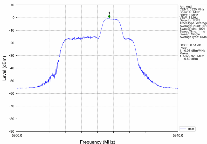
802.11ax(HEW20)_HCH_5320MHz_RU52_Right_Ant1_NTNV
