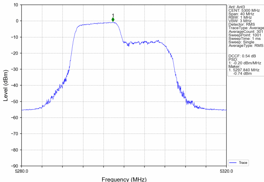
802.11ax(HEW20)_MCH_5300MHz_RU106_Left_Ant3_NTNV
