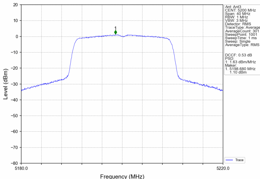
802.11ax(HEW20)_MCH_5200MHz_RU242_Left_Ant3_NTNV
