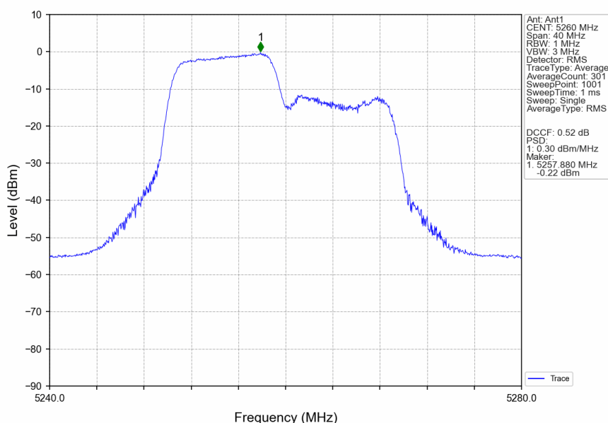
802.11ax(HEW20)_LCH_5260MHz_RU106_Left_Ant1_NTNV
