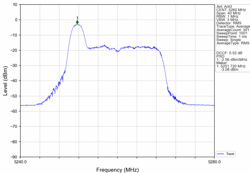
802.11ax(HEW20)_LCH_5260MHz_RU26_Left_Ant3_NTNV
