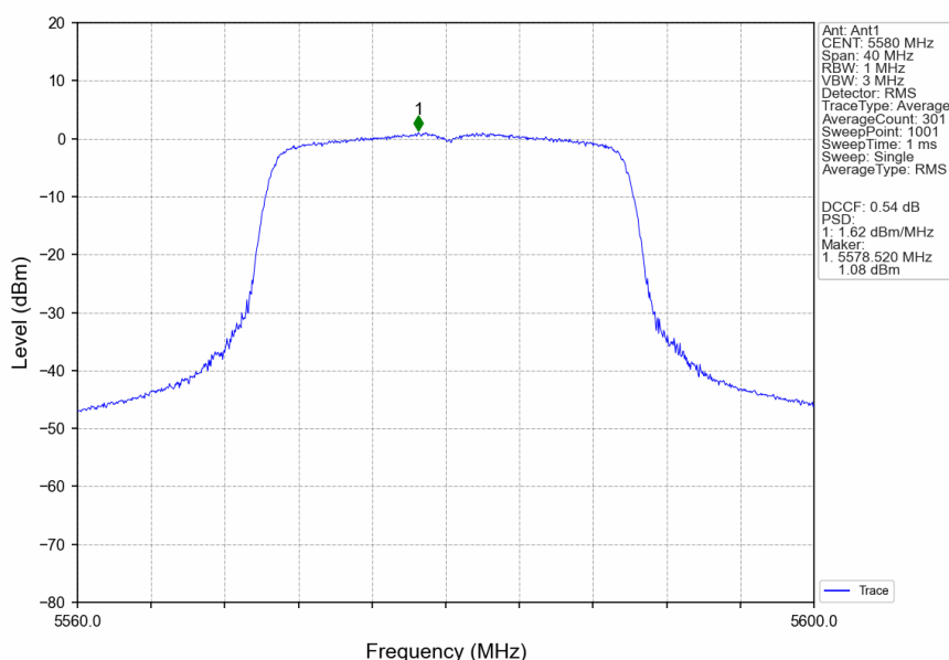
802.11ax(HEW20)_MCH_5580MHz_RU242_Left_Ant1_NTNV
