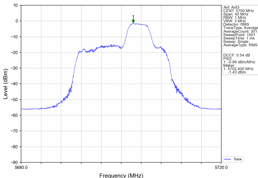
802.11ax(HEW20)_HCH_5700MHz_RU52_Right_Ant3_NTNV
