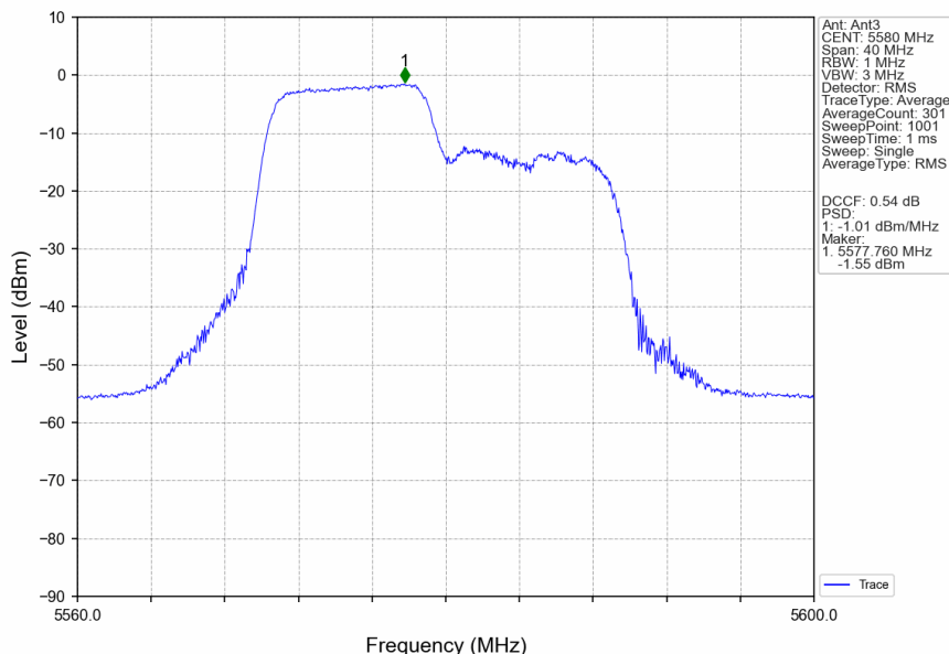
802.11ax(HEW20)_MCH_5580MHz_RU106_Left_Ant3_NTNV
