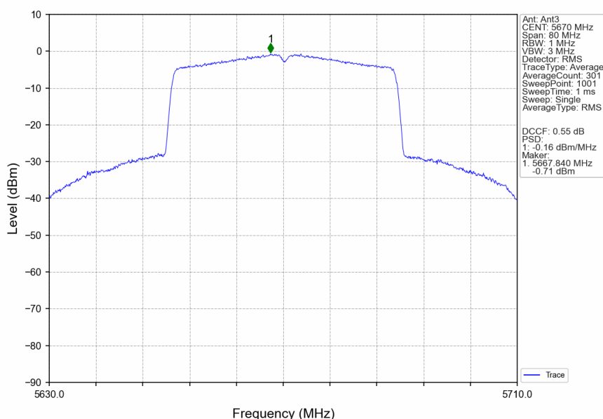
802.11ax(HEW40)_HCH_5670MHz_RU484_Left_Ant3_NTNV
