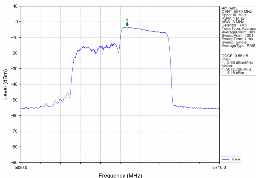
802.11ax(HEW40)_HCH_5670MHz_RU242_Right_Ant3_NTNV
