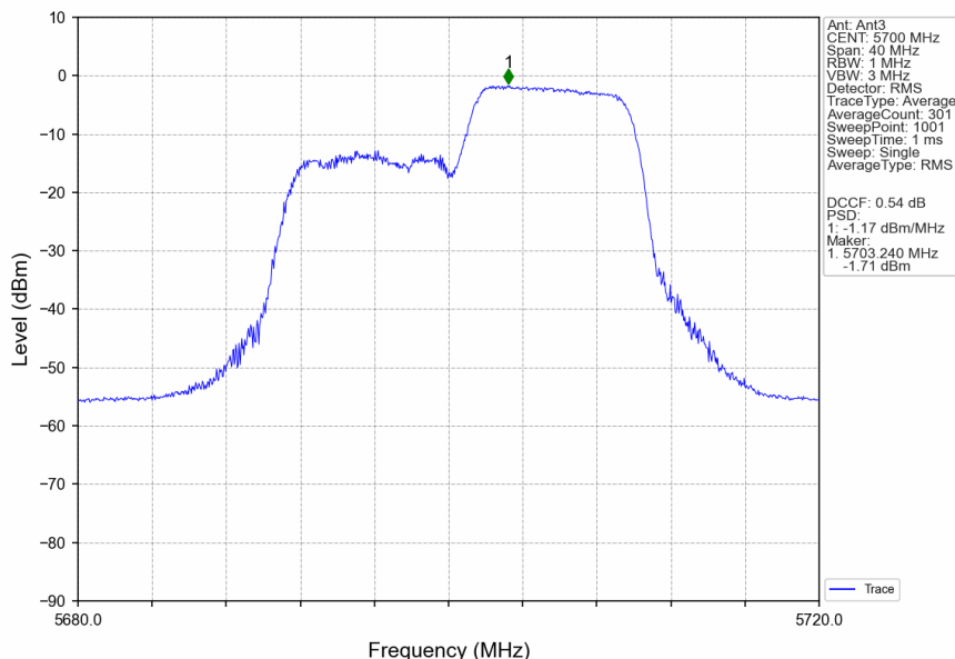
802.11ax(HEW20)_HCH_5700MHz_RU106_Right_Ant3_NTNV
