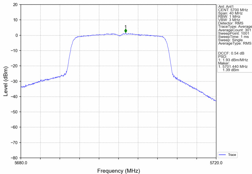
802.11ax(HEW20)_HCH_5700MHz_RU242_Left_Ant1_NTNV
