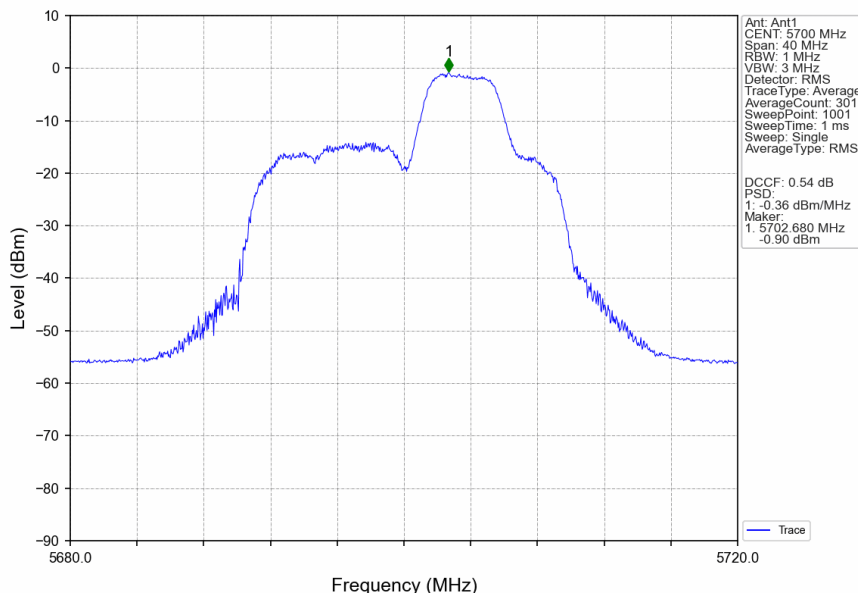
802.11ax(HEW20)_HCH_5700MHz_RU52_Right_Ant1_NTNV
