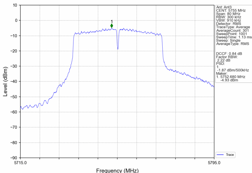
802.11ac(VHT40)_LCH_5755MHz_Ant3_NTNV
