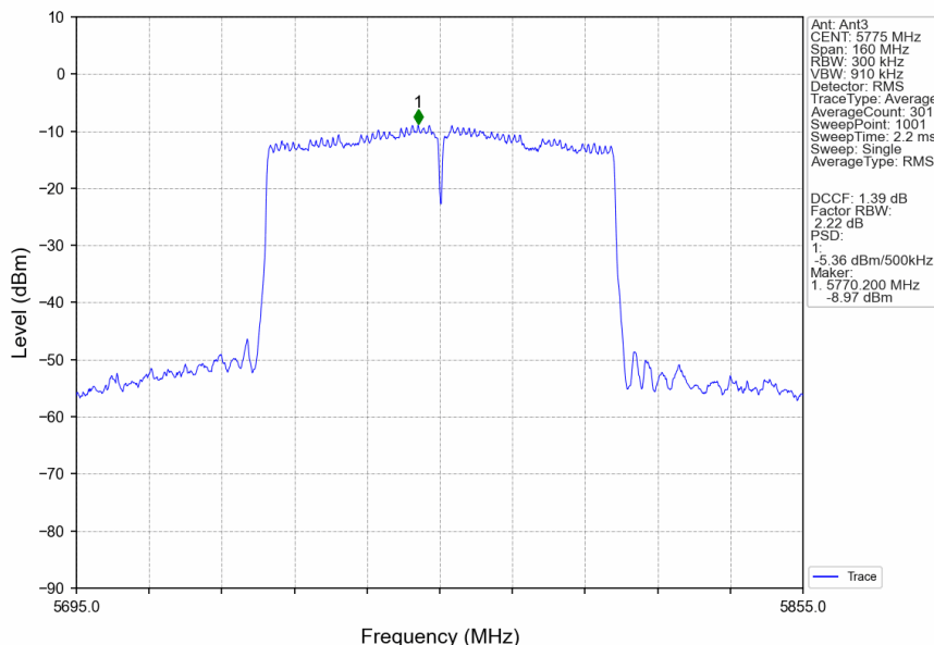
802.11ac(VHT80)_MCH_5775MHz_Ant3_NTNV
