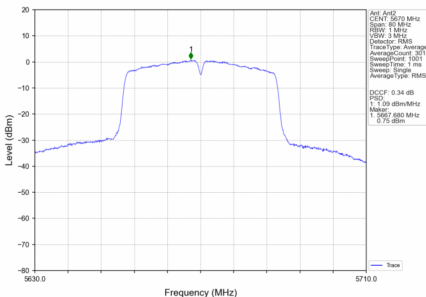
802.11ac(VHT40)_HCH_5670MHz_MIMO_NTNV
