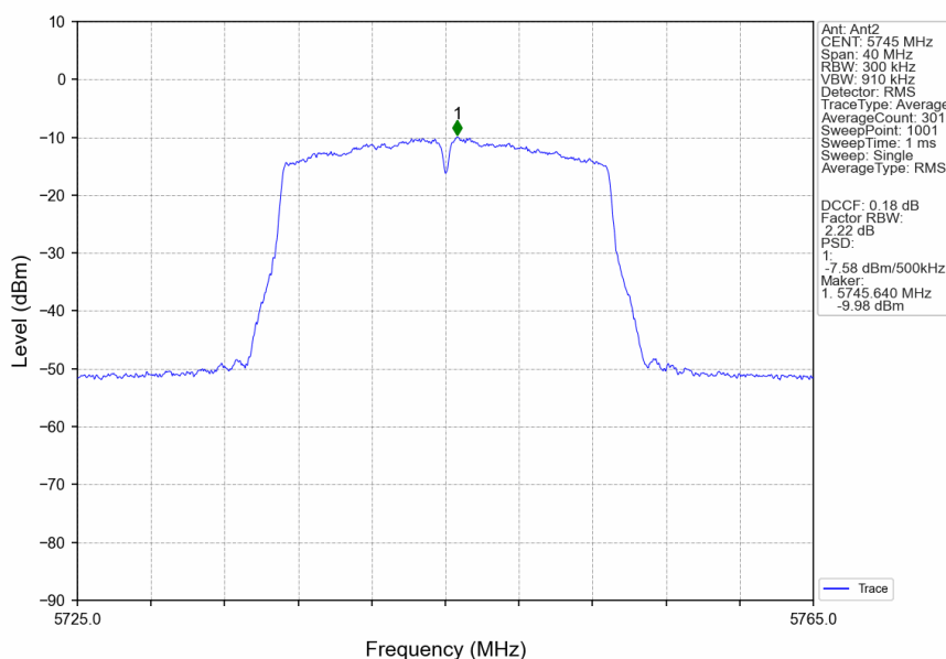
802.11ac(VHT20)_LCH_5745MHz_MIMO_NTNV
