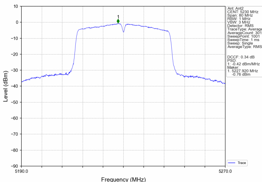
802.11ac(VHT40)_HCH_5230MHz_Ant2_NTNV
