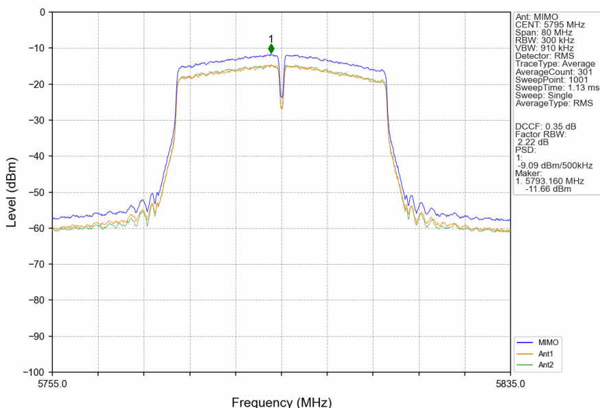
802.11ac(VHT40)_HCH_5795MHz_MIMO_NTNV
