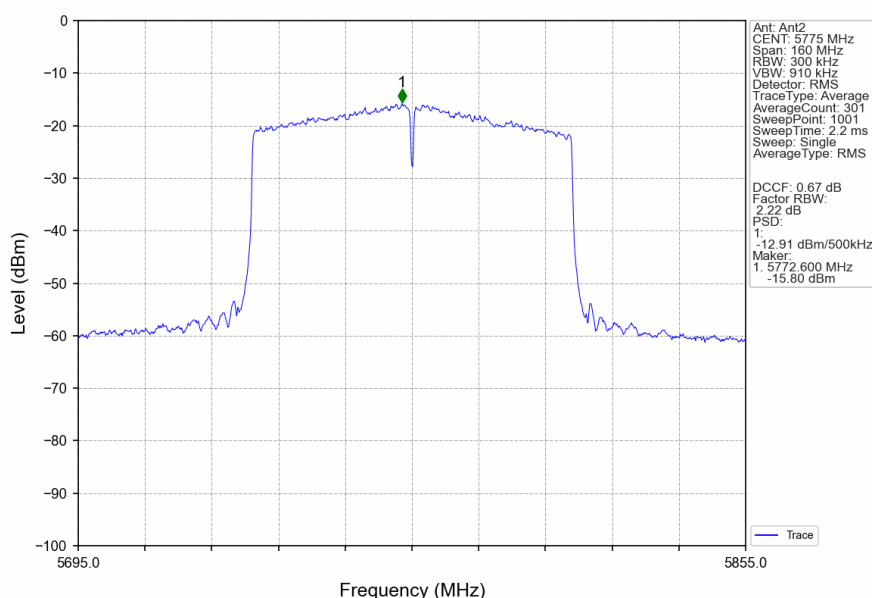
802.11ac(VHT80)_MCH_5775MHz_Ant2_NTNV
