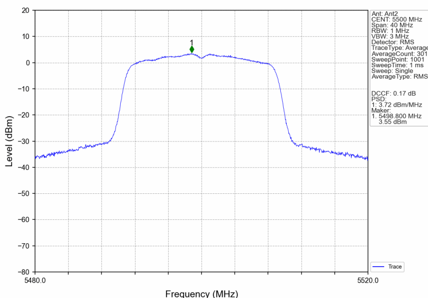
802.11ac(VHT20)_LCH_5500MHz_Ant2_NTNV
