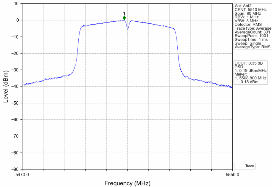
802.11n(HT40)_LCH_5510MHz_MIMO_NTNV
