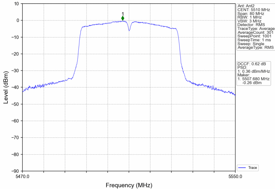
802.11ac(VHT40)_LCH_5510MHz_MIMO_NTNV
