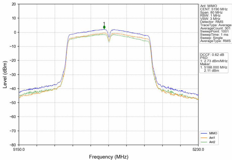
802.11ac(VHT40)_LCH_5190MHz_MIMO_NTNV
