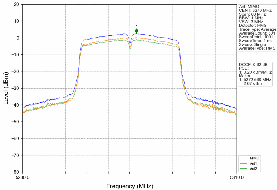
802.11ac(VHT40)_LCH_5270MHz_MIMO_NTNV
