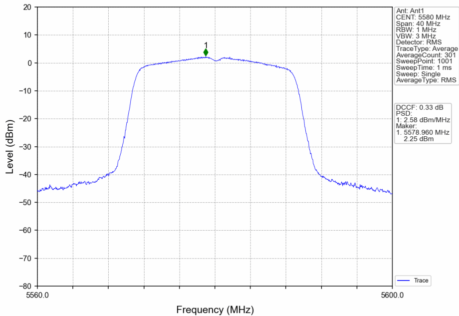
802.11ac(VHT20)_MCH_5580MHz_Ant1_NTNV
