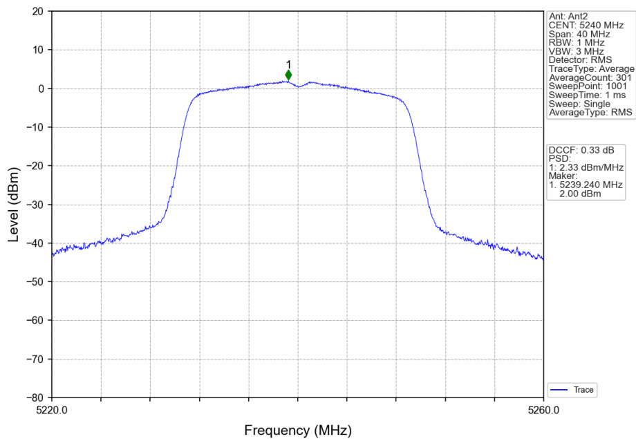
802.11ac(VHT20)_HCH_5240MHz_Ant2_NTNV
