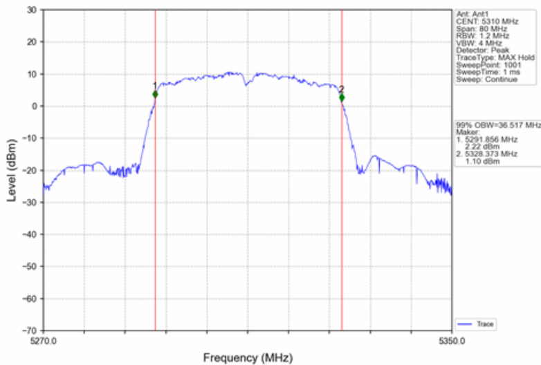
802.11ac(VHT40)_HCH_5310MHz_Ant1_NTNV 2
