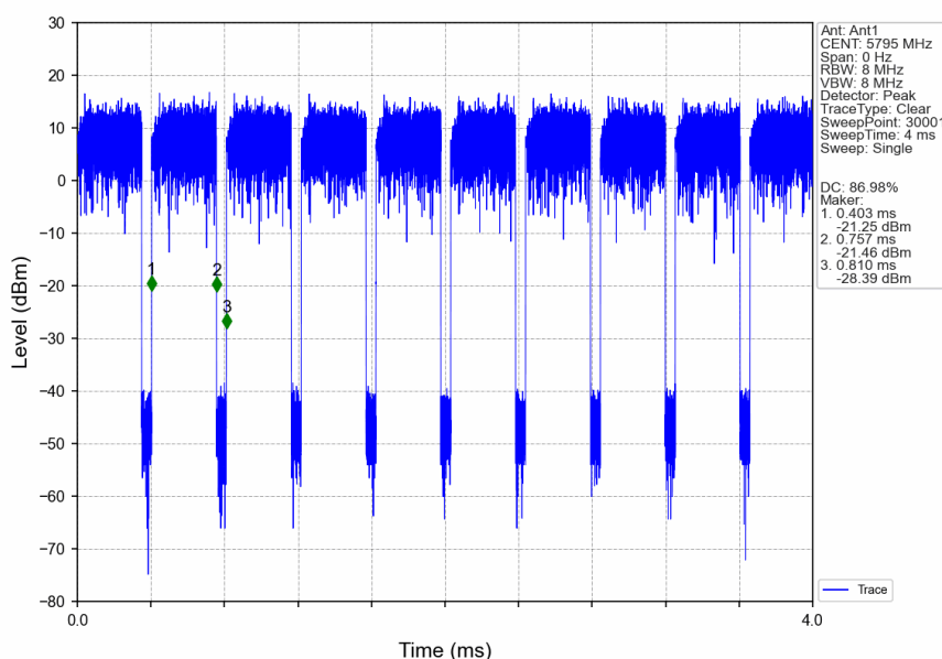
802.11ac(VHT40)_HCH_5795MHz_Ant1_NTNV
